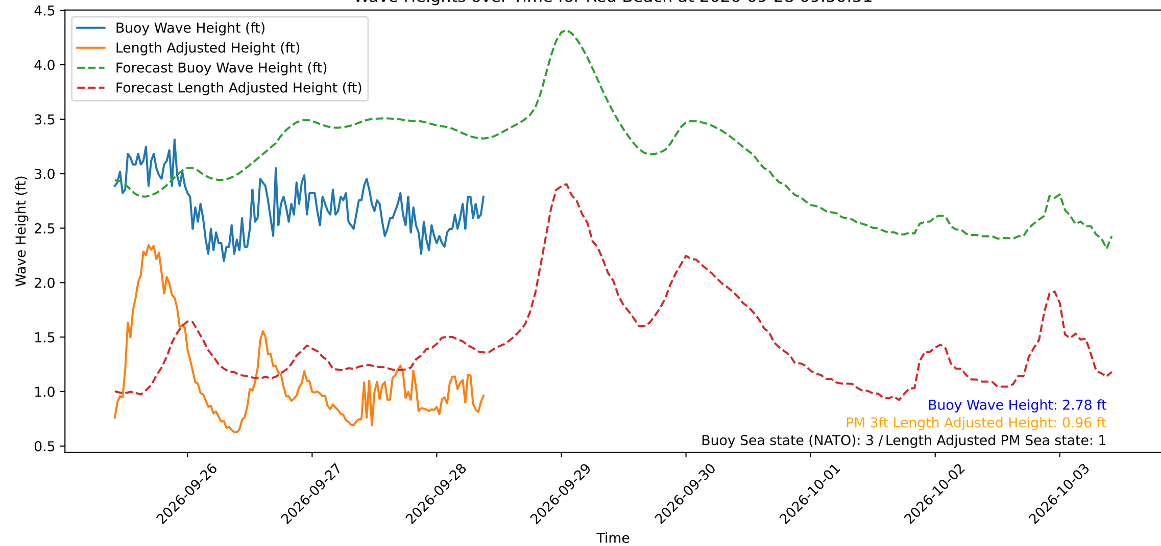
Wave Heights over Time for Red Beach at 2026-09-28 09:50:51
