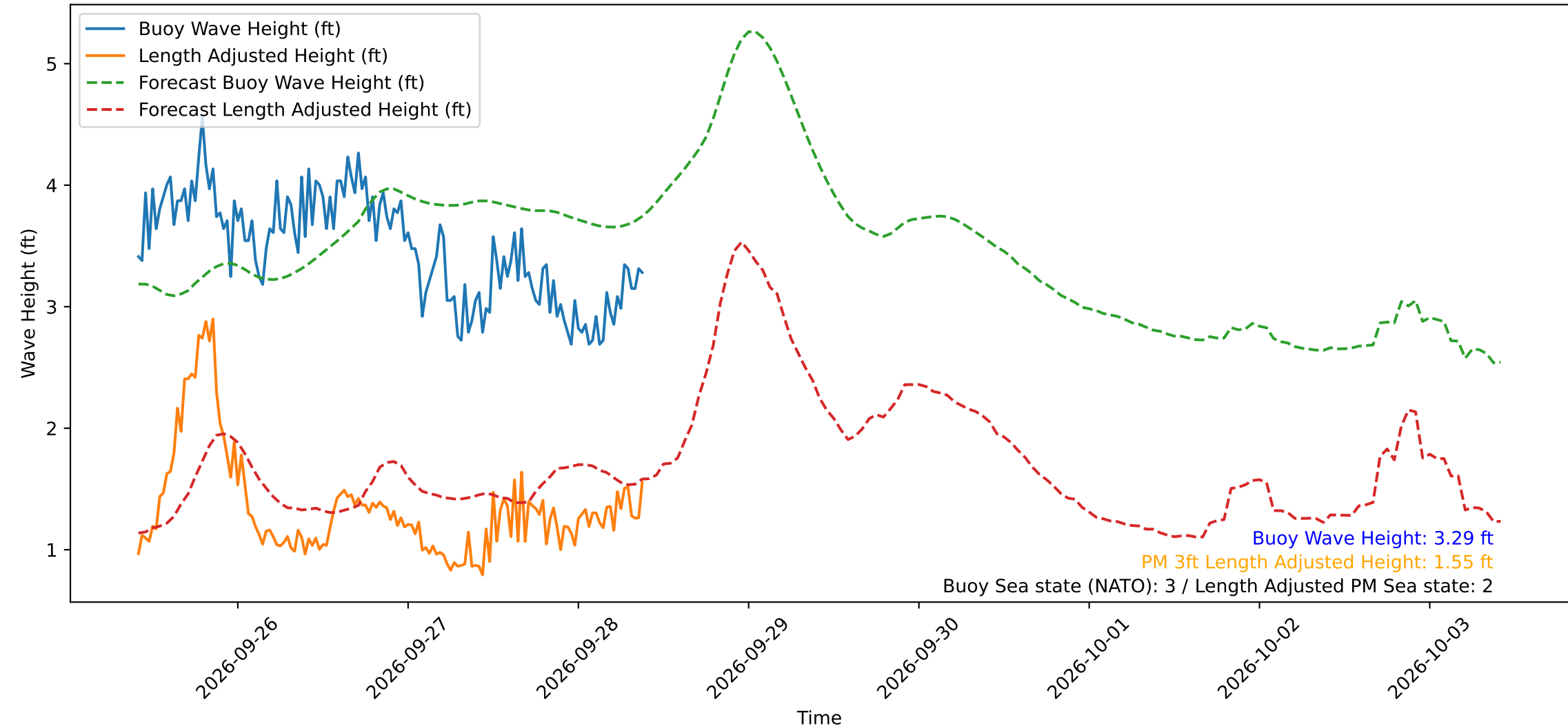
Wave Heights over Time for Green Beach at 2026-09-28 09:51:15
