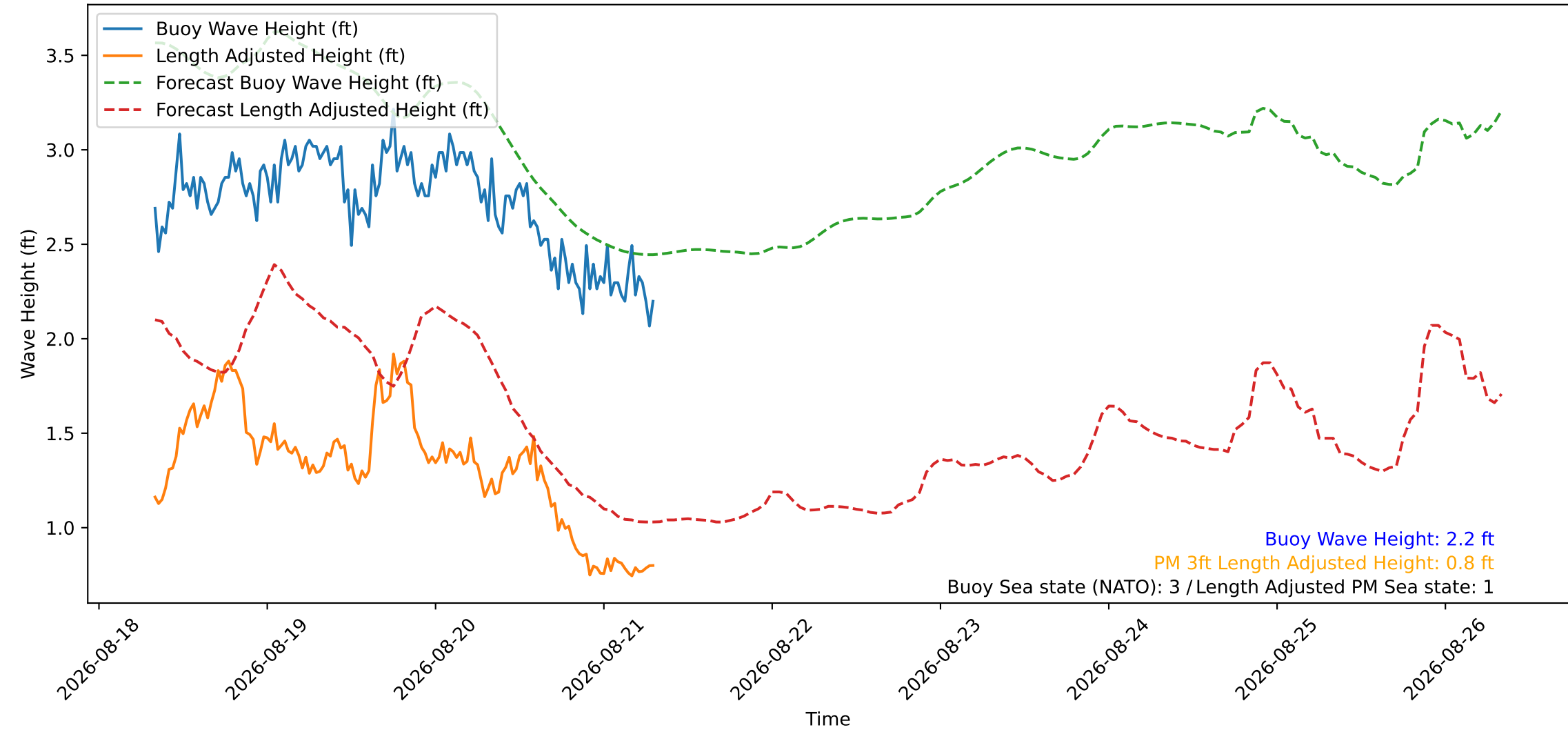
Wave Heights over Time for Red Beach at 2026-08-21 07:40:45
