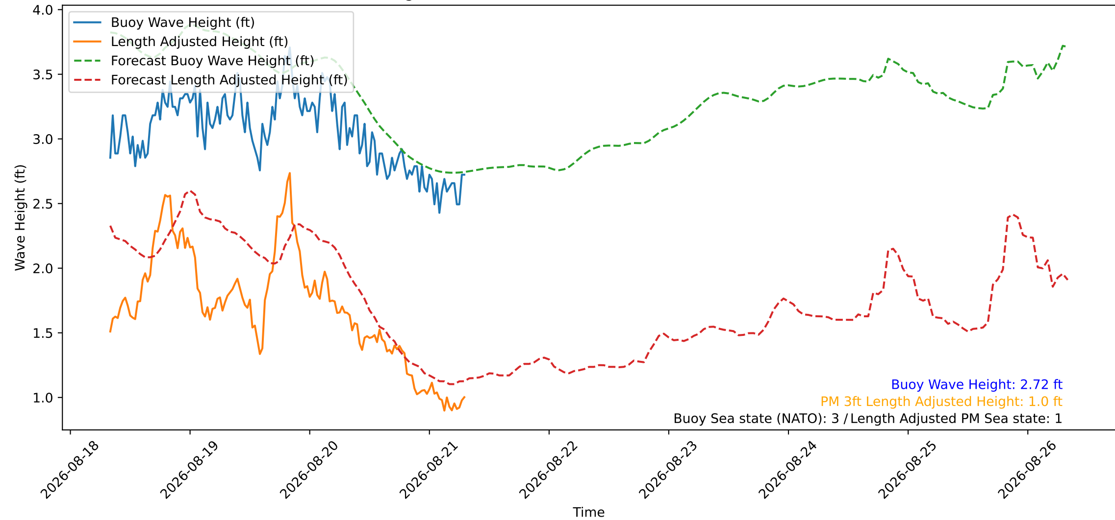
Wave Heights over Time for Green Beach at 2026-08-21 07:41:07
