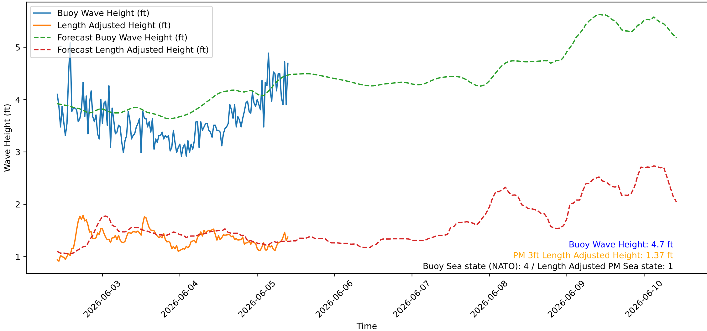
Wave Heights over Time for Oceanside Harbor at 2026-06-05 10:10:26
