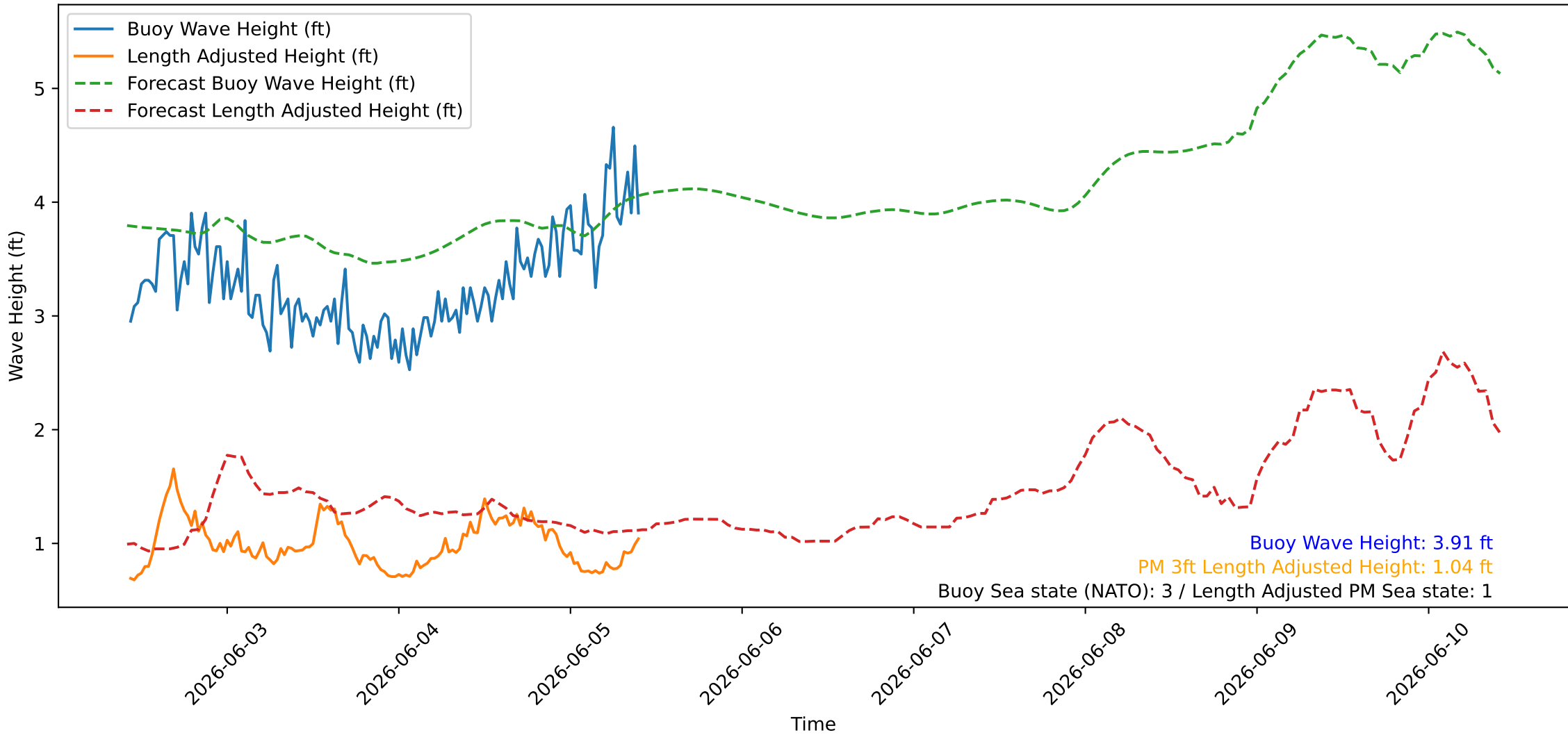
Wave Heights over Time for Red Beach at 2026-06-05 10:10:45
