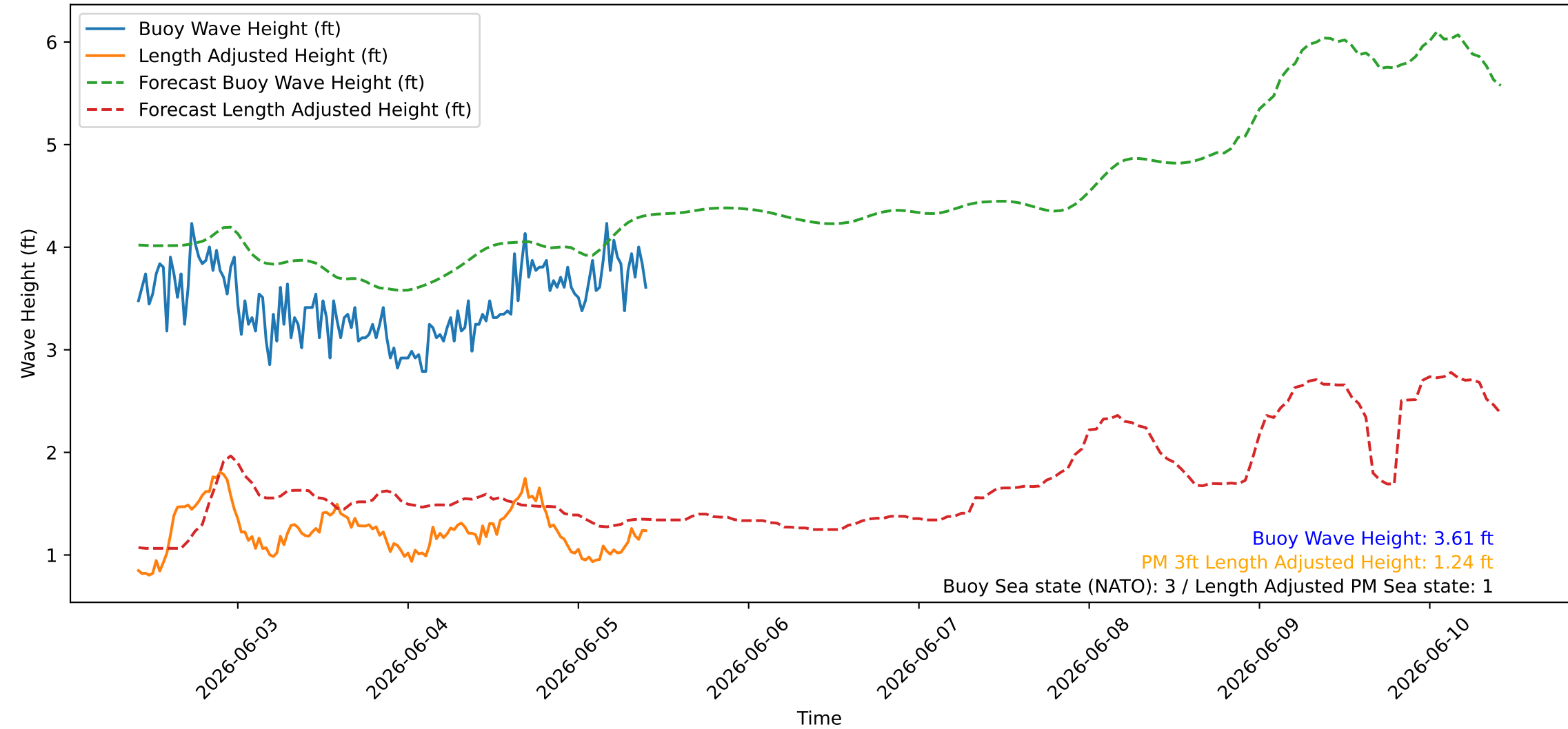
Wave Heights over Time for Green Beach at 2026-06-05 10:11:08
