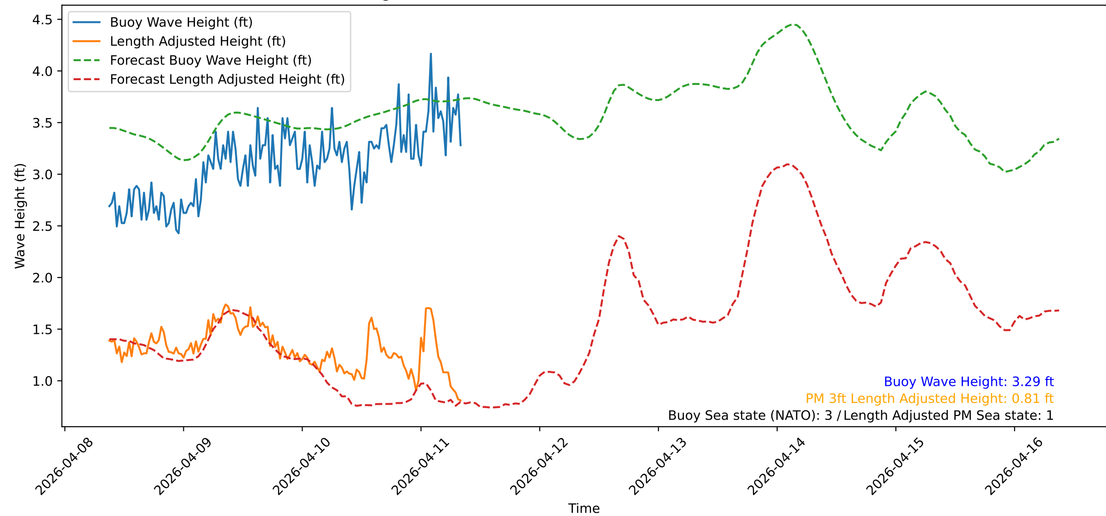
Wave Heights over Time for Oceanside Harbor at 2026-04-11 09:00:32
