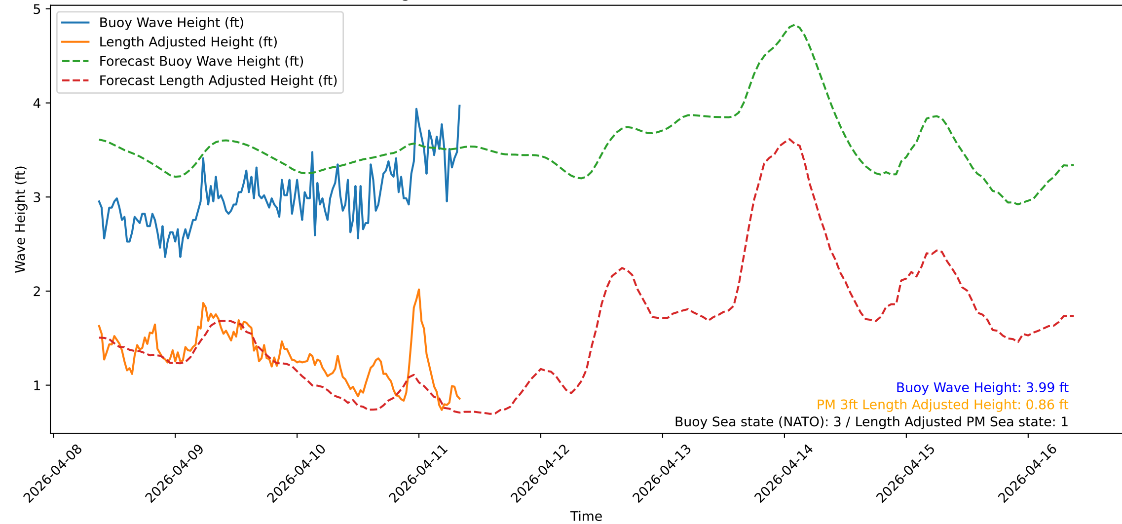
Wave Heights over Time for Green Beach at 2026-04-11 09:01:13
