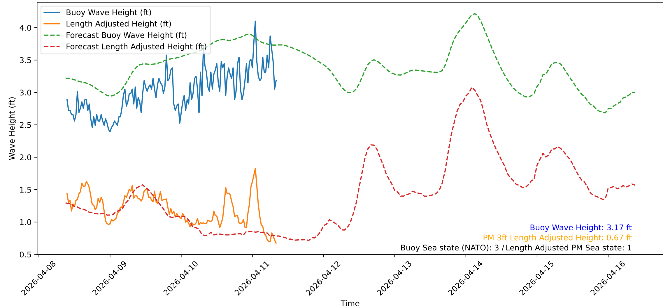
Wave Heights over Time for Red Beach at 2026-04-11 09:00:51
