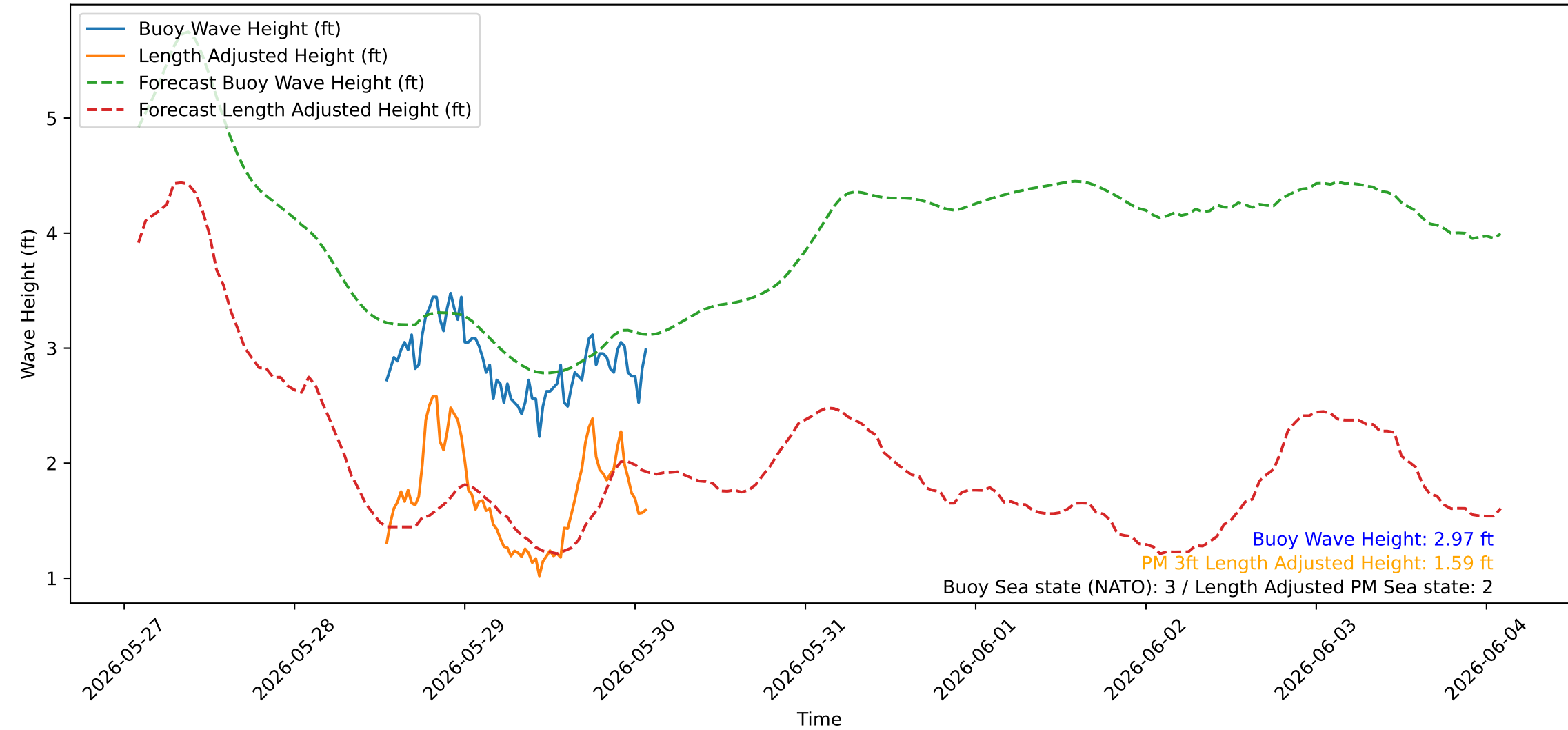
Wave Heights over Time for Oceanside Harbor at 2026-05-30 02:10:23
