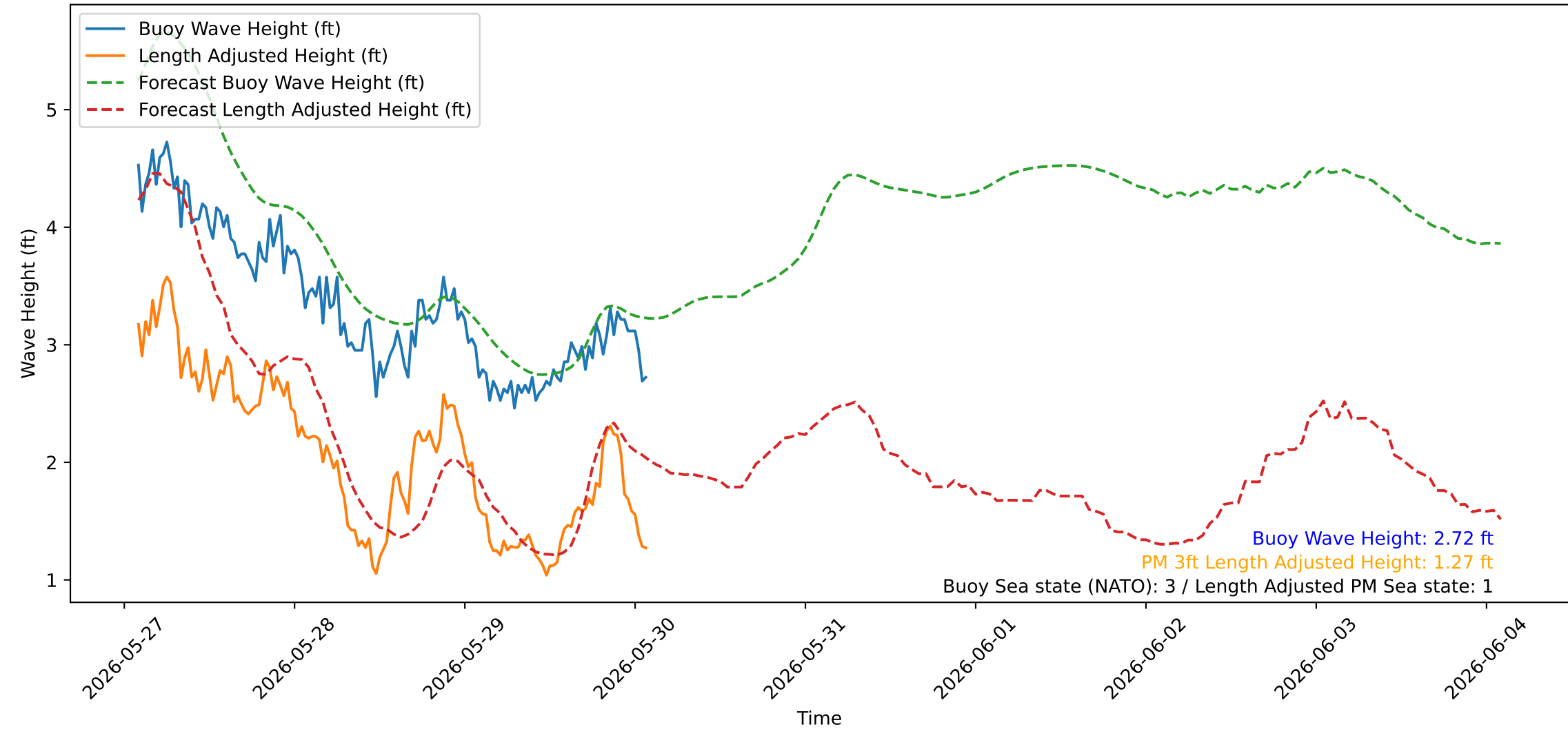
Wave Heights over Time for Green Beach at 2026-05-30 02:11:04
