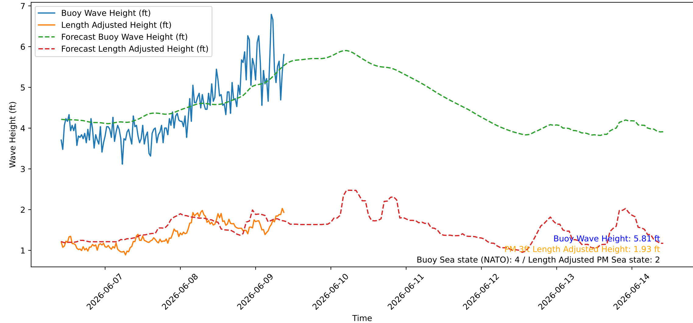
Wave Heights over Time for Green Beach at 2026-06-09 09:51:08
