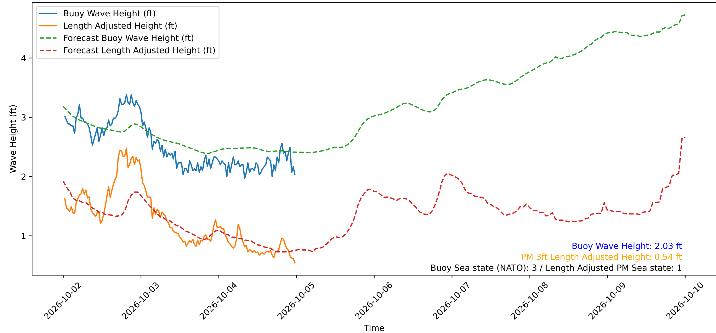
Wave Heights over Time for Green Beach at 2026-10-05 00:21:15
