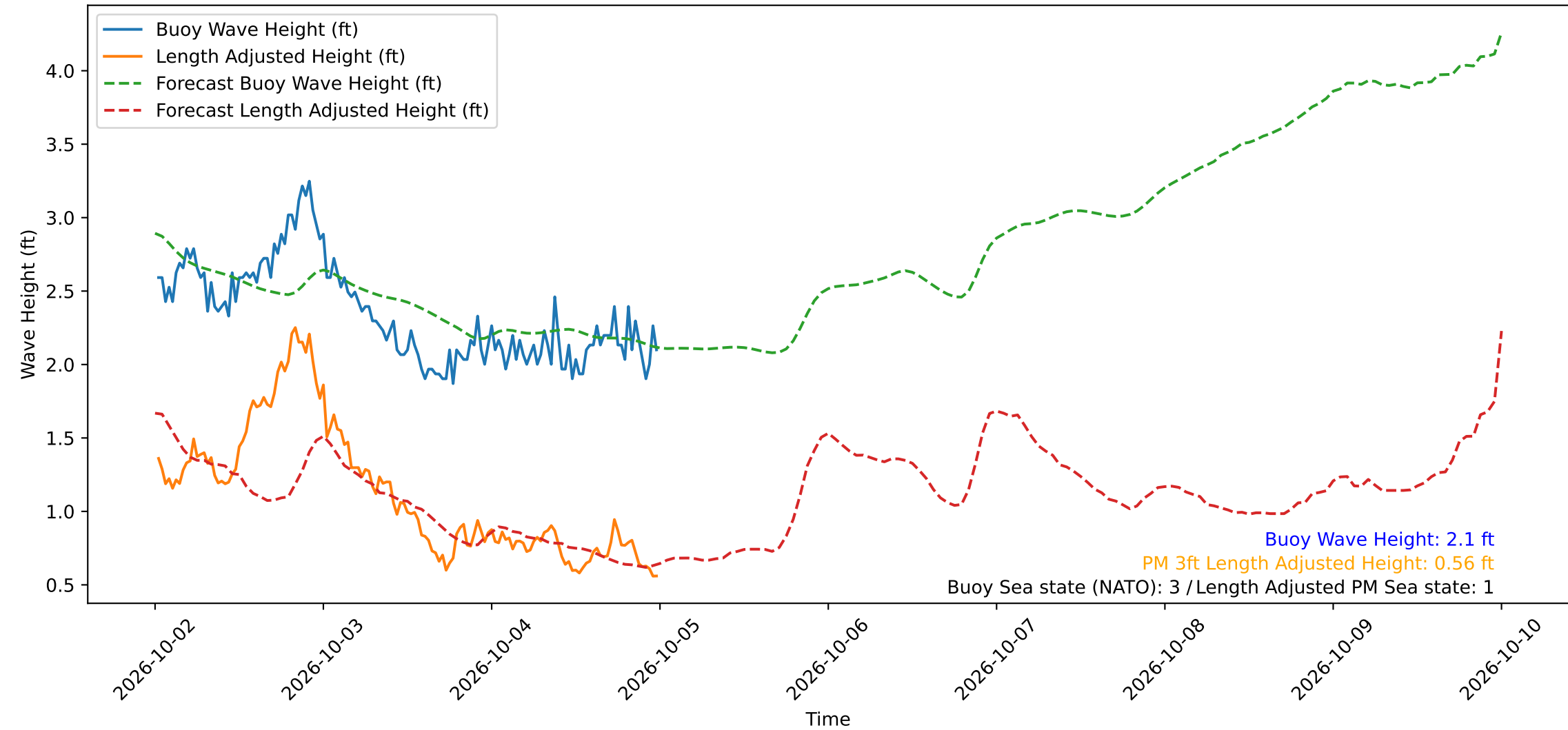
Wave Heights over Time for Red Beach at 2026-10-05 00:20:51
