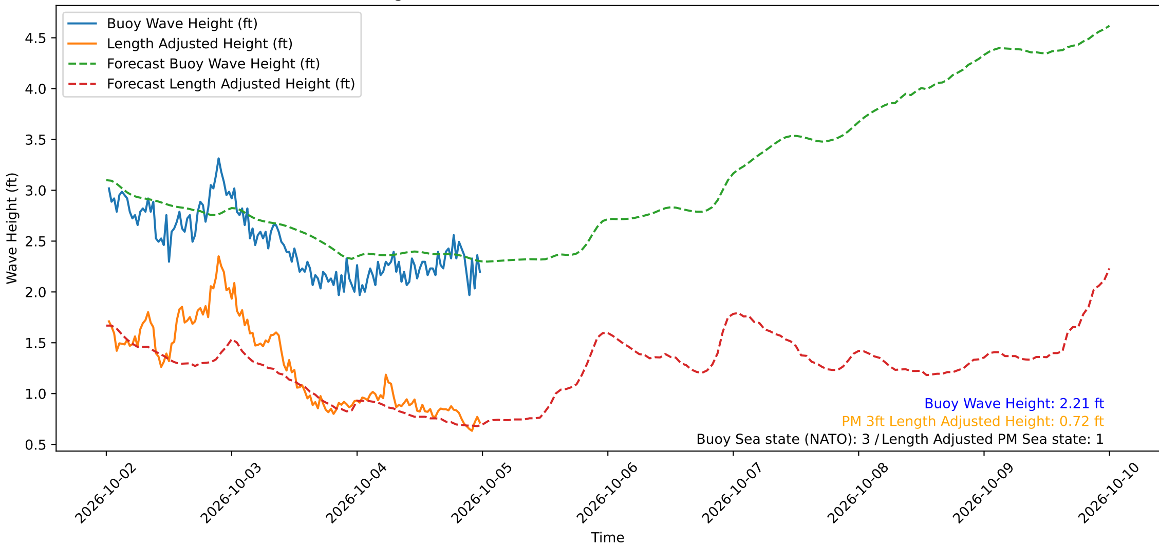
Wave Heights over Time for Oceanside Harbor at 2026-10-05 00:20:30
