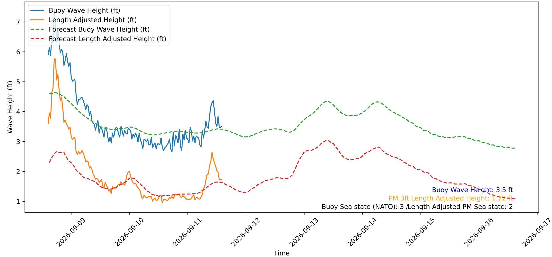
Wave Heights over Time for Oceanside Harbor at 2026-09-11 14:40:30
