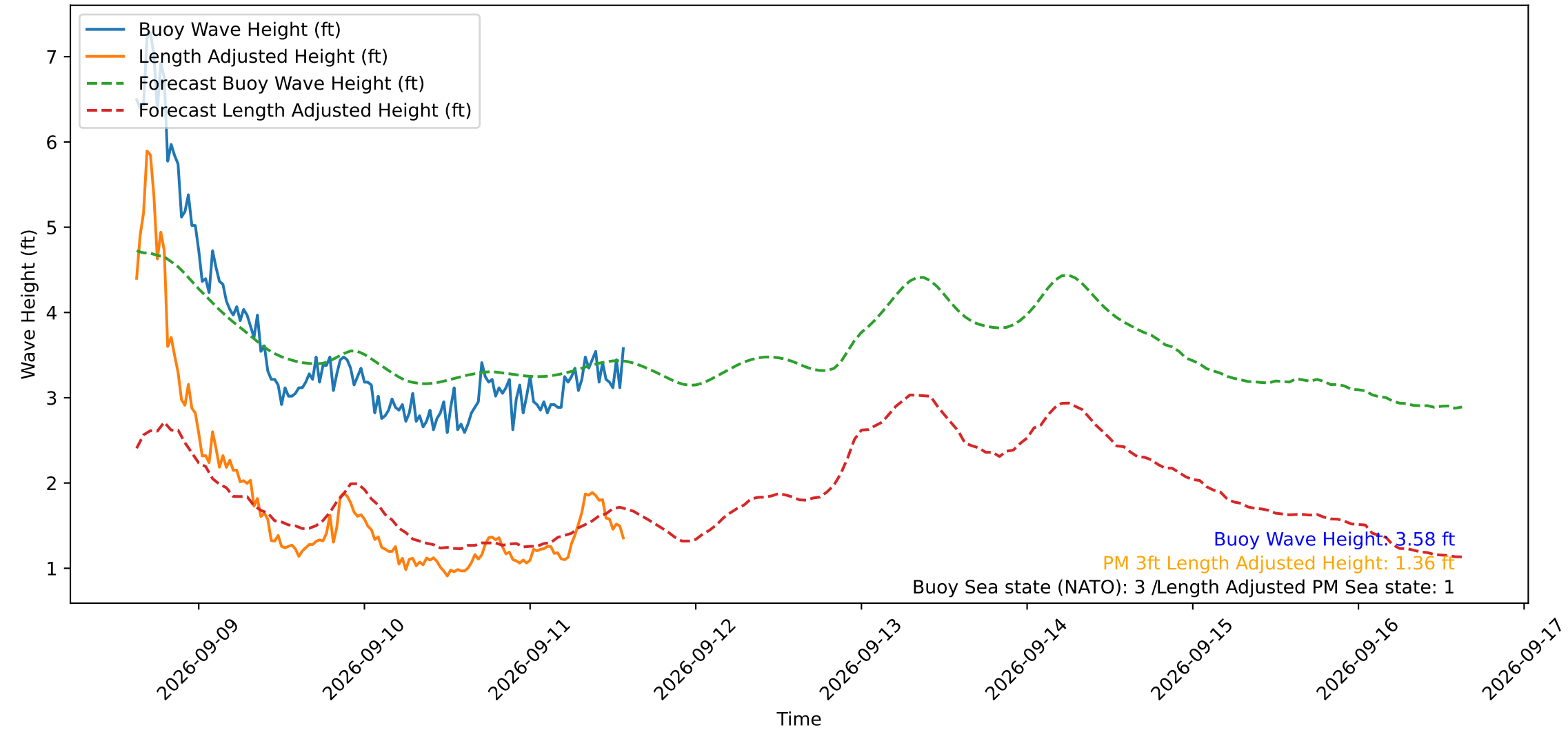
Wave Heights over Time for Green Beach at 2026-09-11 14:41:13
