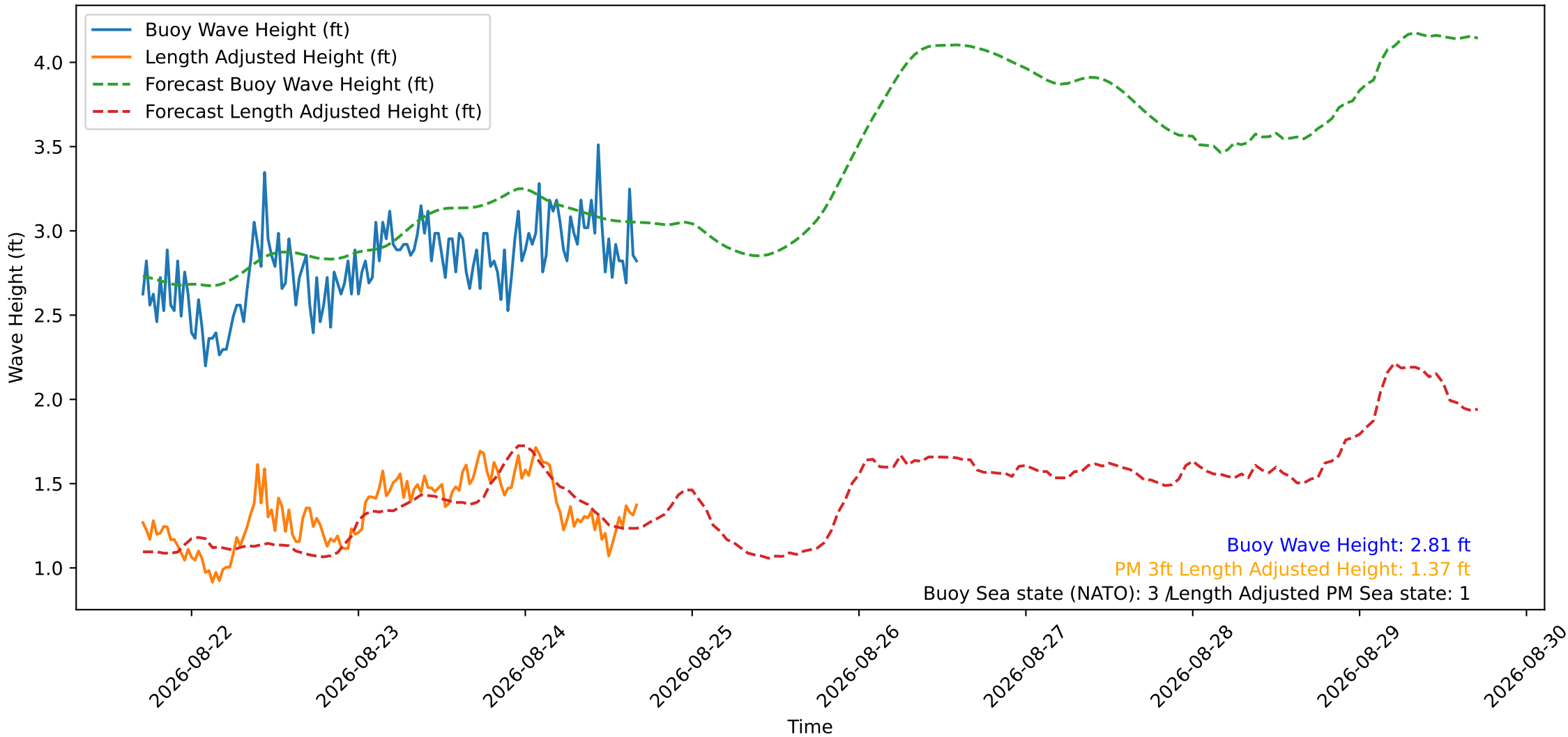
Wave Heights over Time for Oceanside Harbor at 2026-08-24 17:10:29
