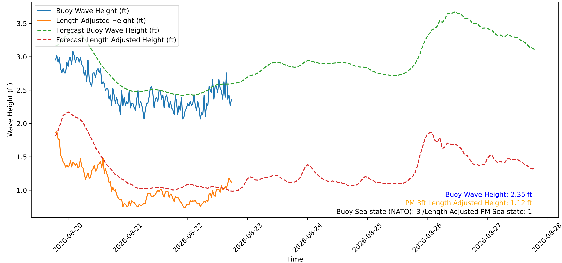
Wave Heights over Time for Red Beach at 2026-08-22 18:40:48
