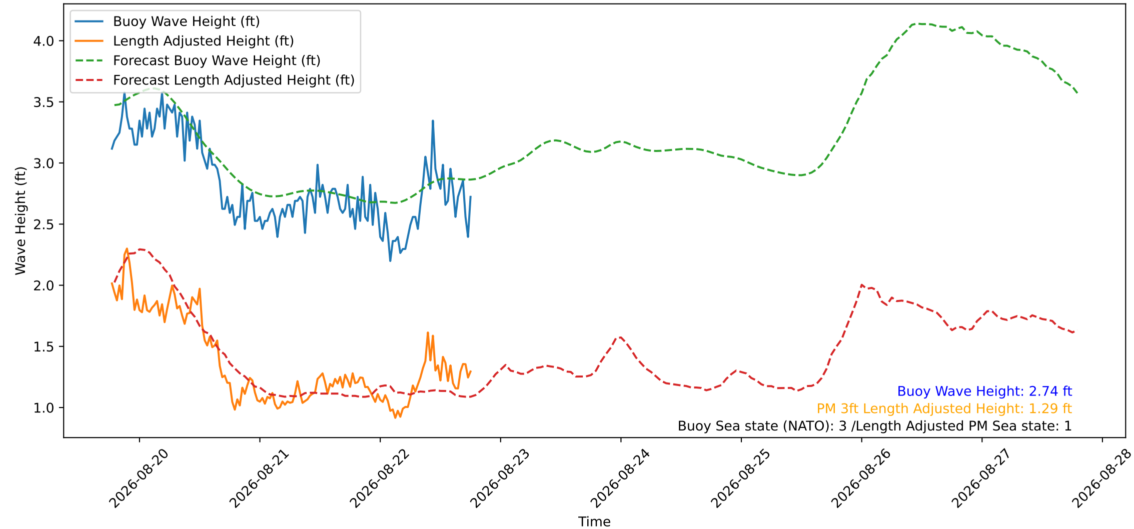
Wave Heights over Time for Oceanside Harbor at 2026-08-22 18:40:29
