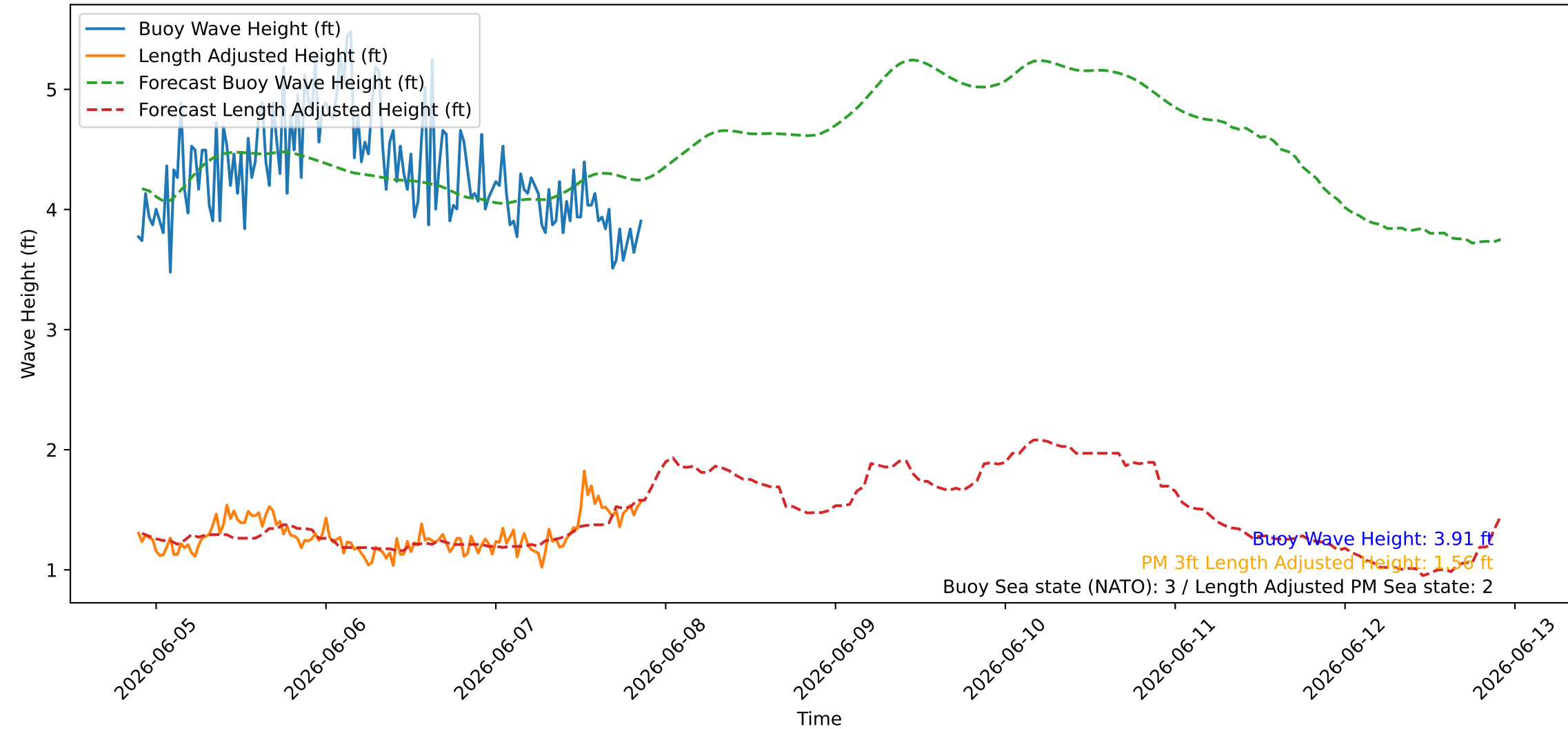
Wave Heights over Time for Oceanside Harbor at 2026-06-07 21:30:26
