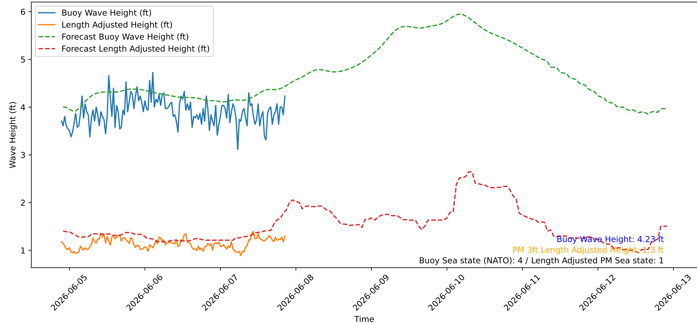
Wave Heights over Time for Green Beach at 2026-06-07 21:31:08
