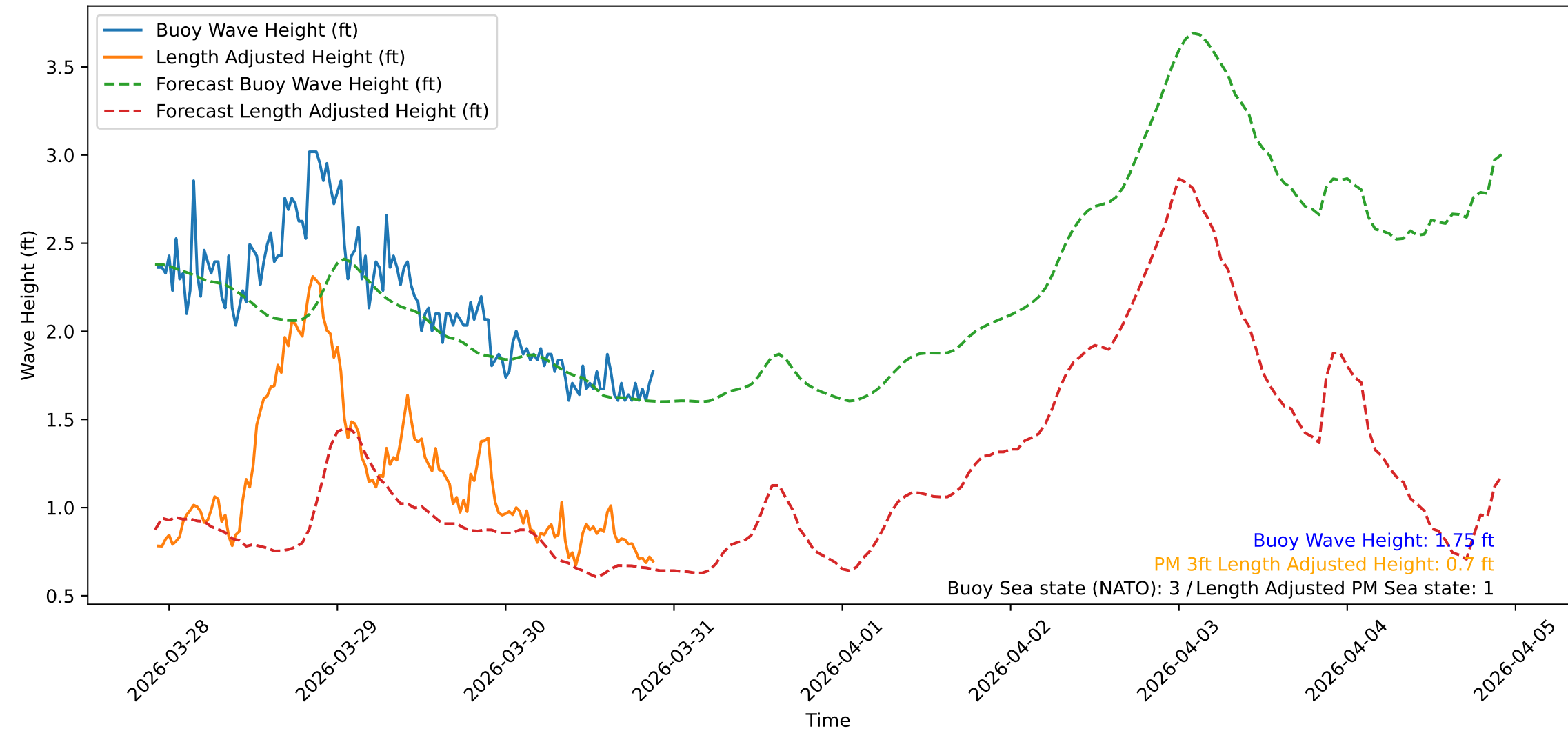
Wave Heights over Time for Red Beach at 2026-03-30 22:00:48
