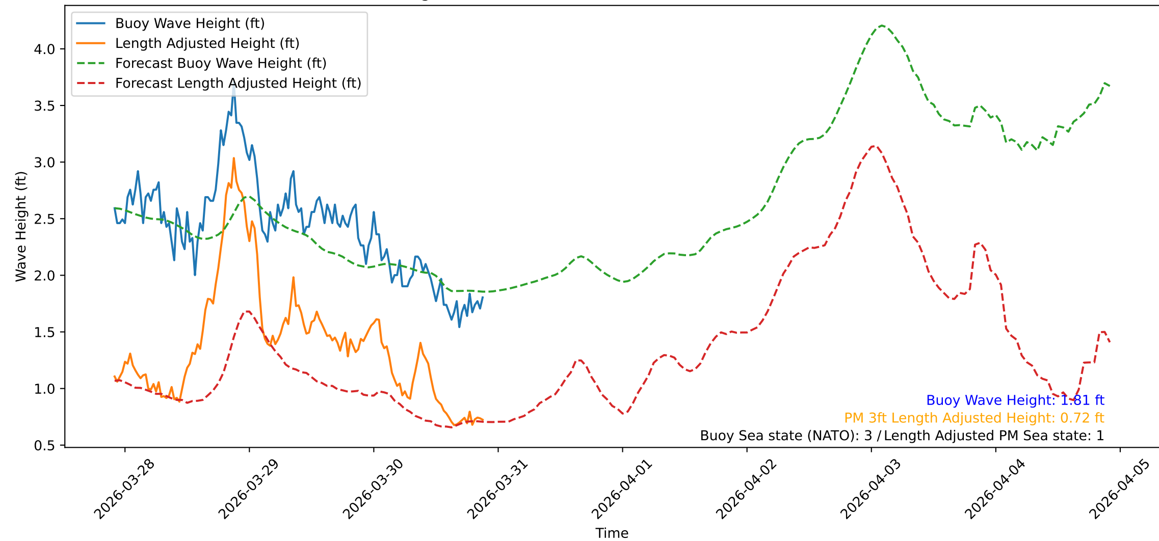
Wave Heights over Time for Green Beach at 2026-03-30 22:01:10
