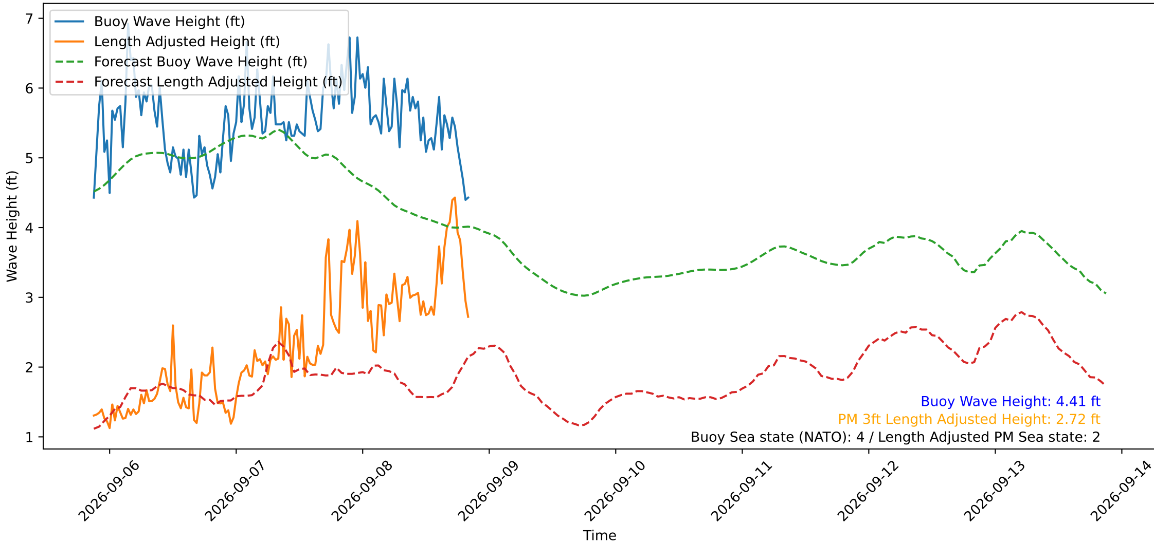
Wave Heights over Time for Red Beach at 2026-09-08 20:40:49
