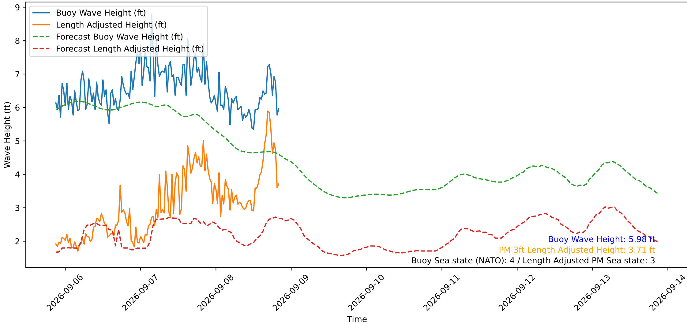
Wave Heights over Time for Green Beach at 2026-09-08 20:41:12
