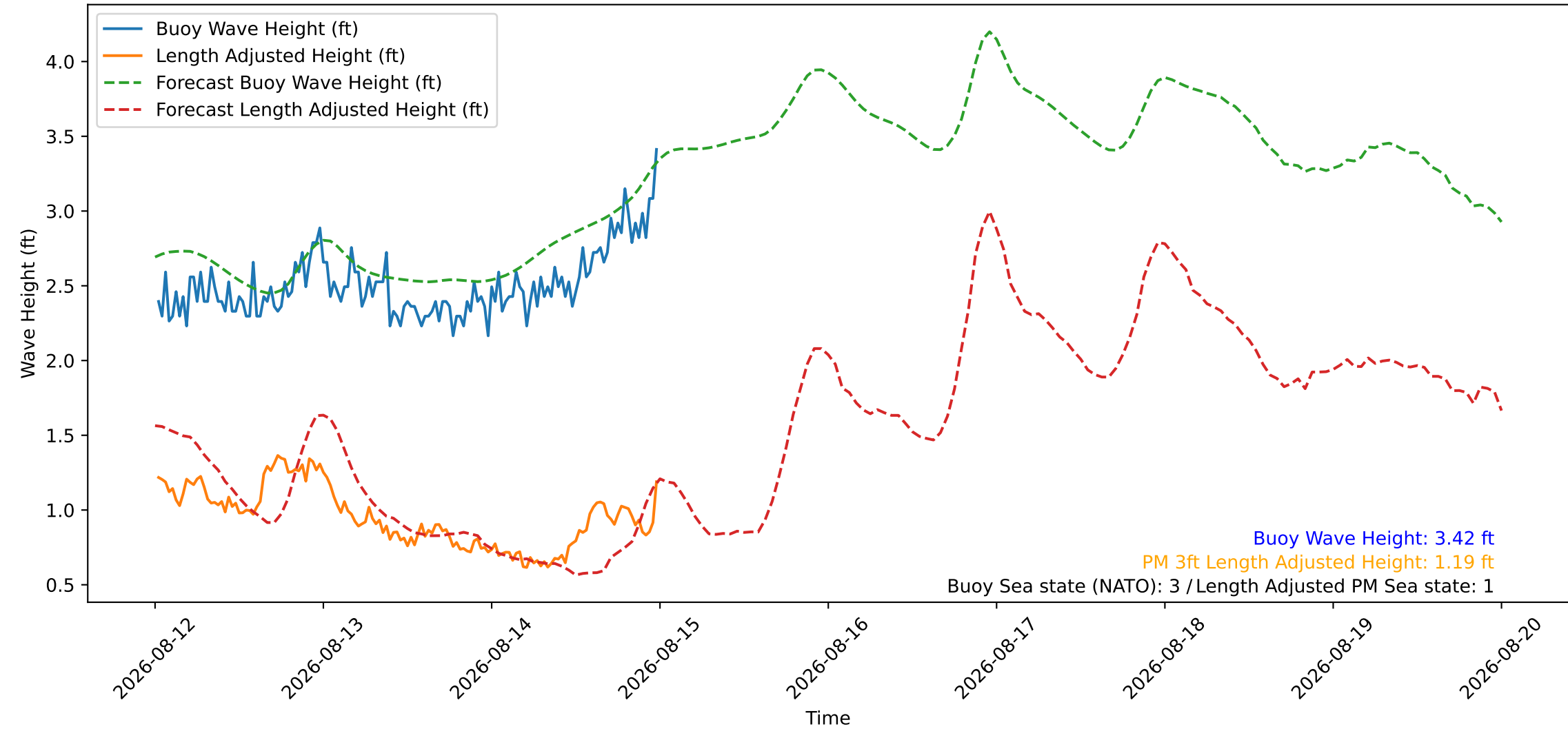
Wave Heights over Time for Red Beach at 2026-08-15 00:20:48
