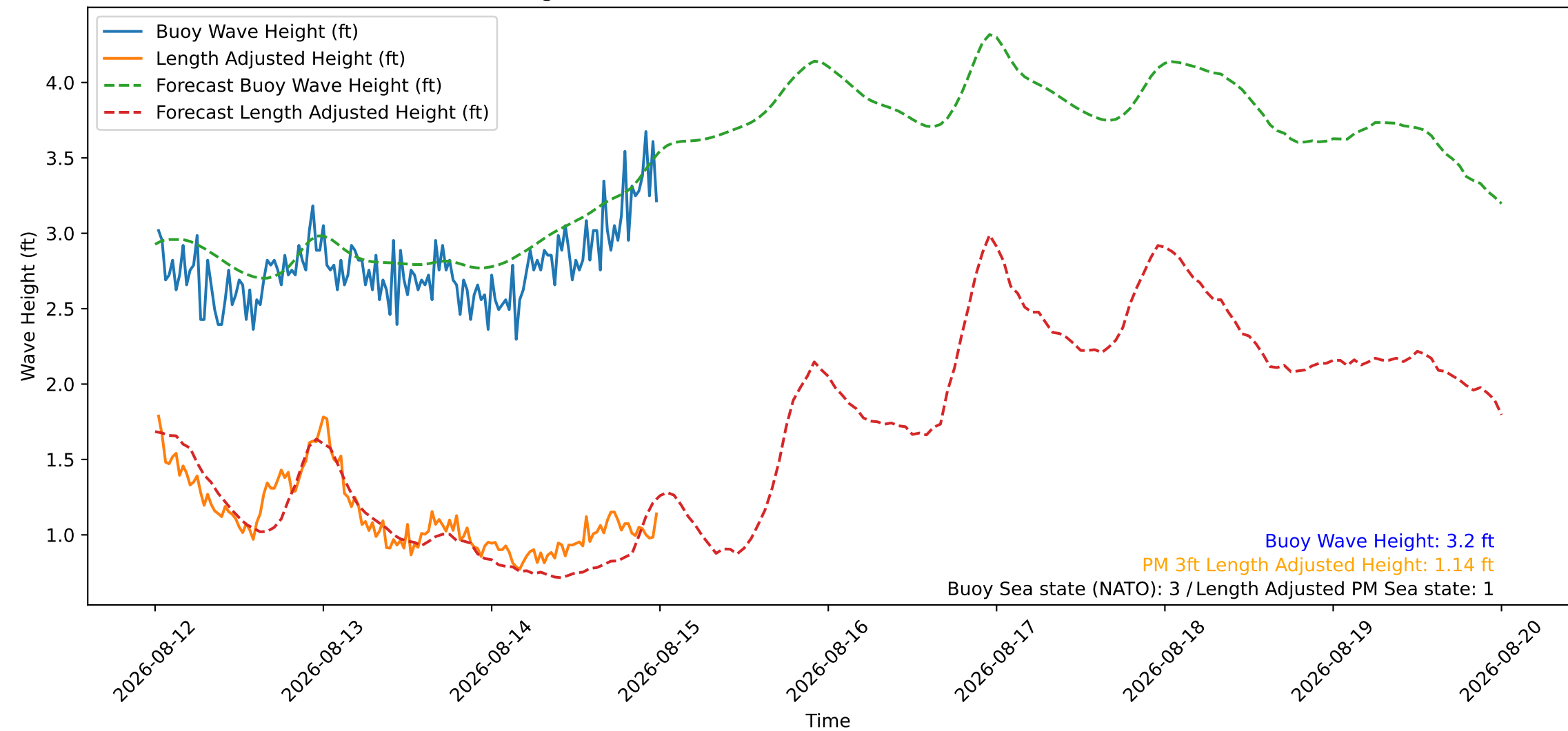
Wave Heights over Time for Oceanside Harbor at 2026-08-15 00:20:27
