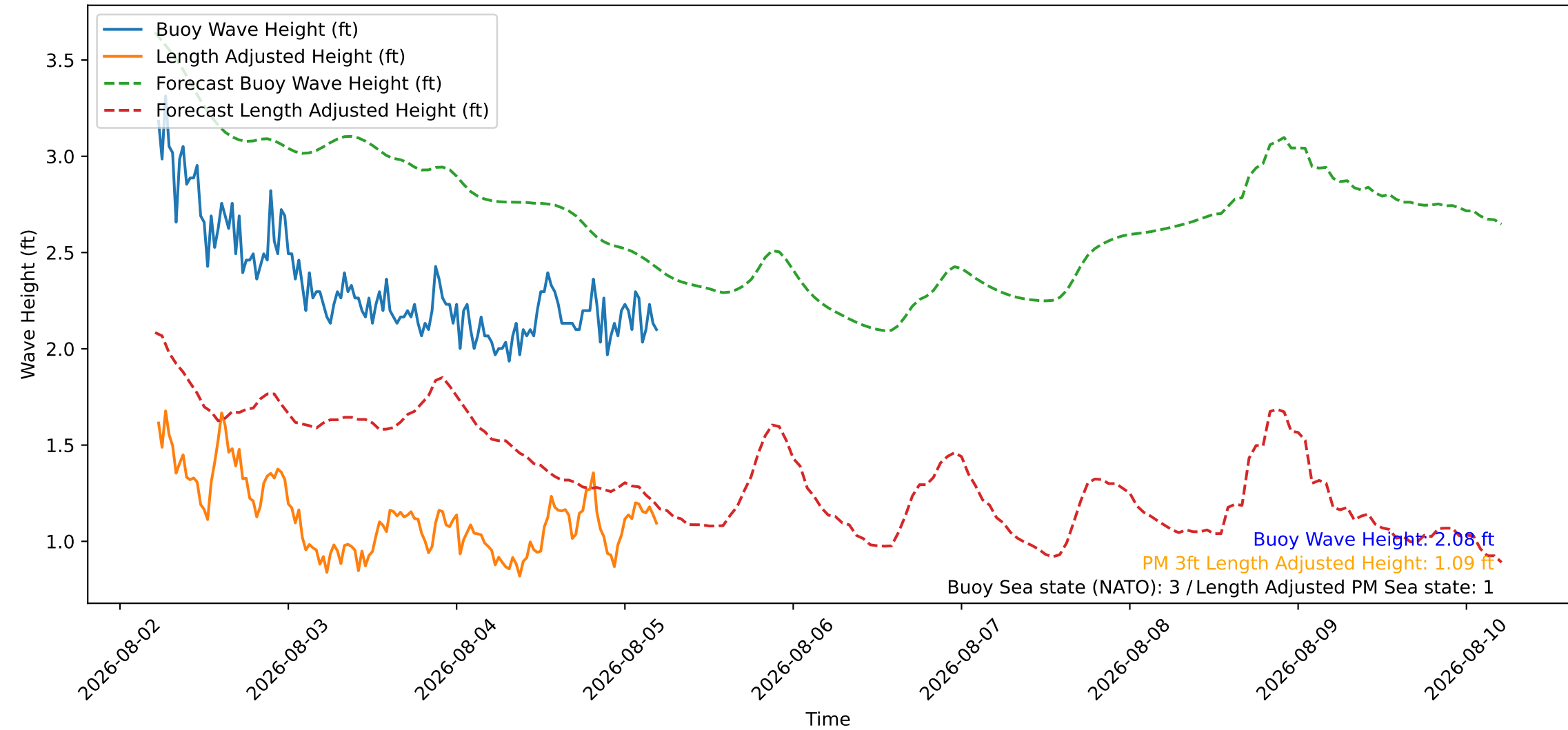
Wave Heights over Time for Green Beach at 2026-08-05 05:21:09
