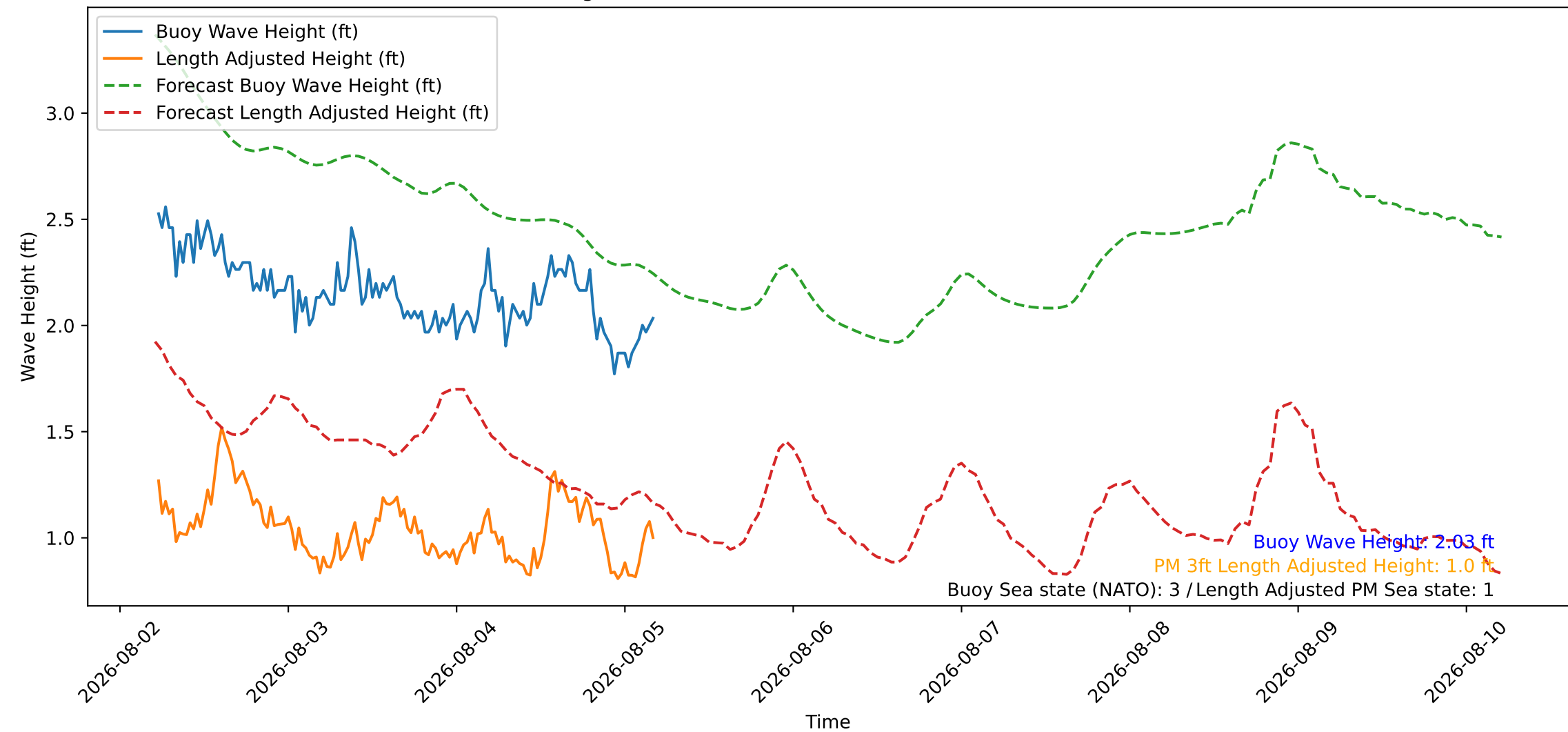
Wave Heights over Time for Red Beach at 2026-08-05 05:20:46
