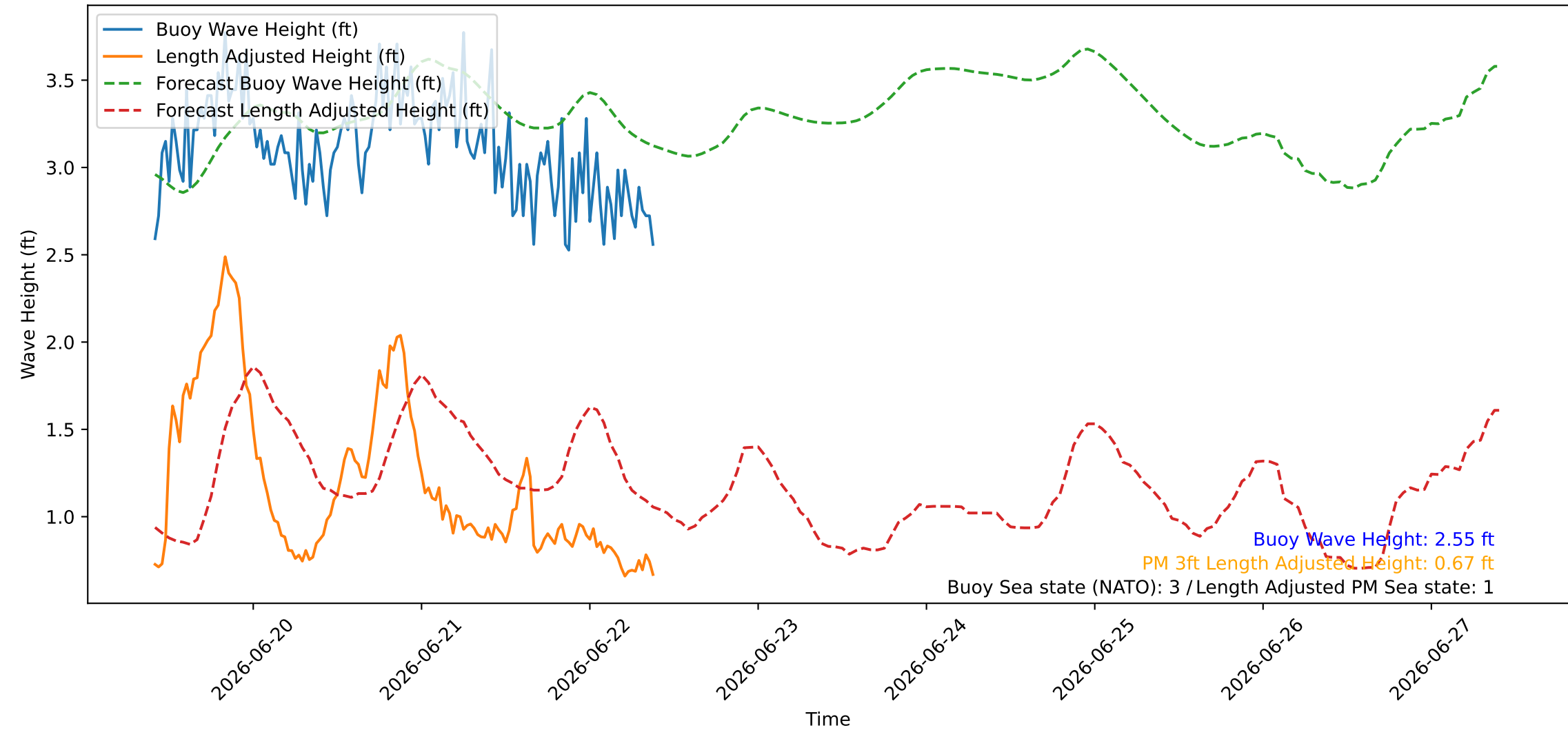
Wave Heights over Time for Red Beach at 2026-06-22 09:50:46
