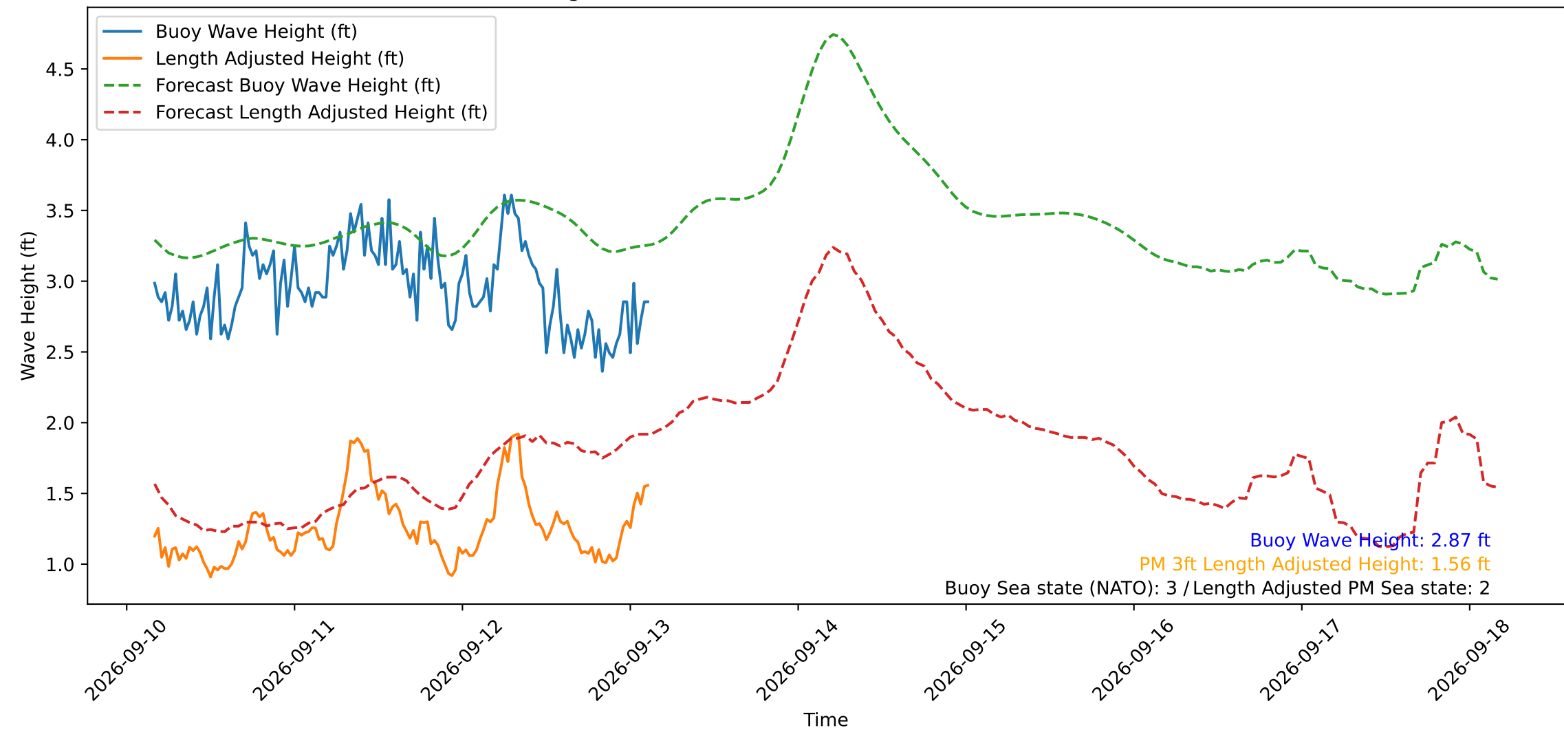
Wave Heights over Time for Green Beach at 2026-09-13 03:31:11
