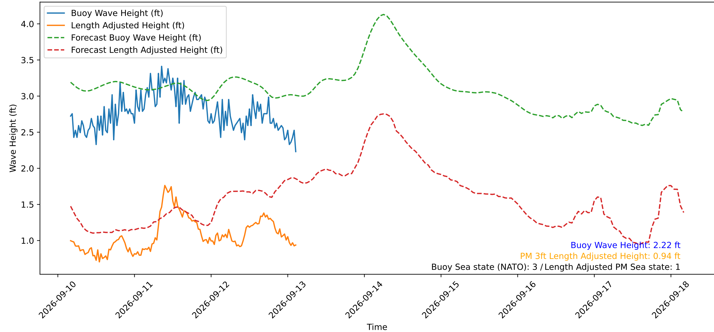
Wave Heights over Time for Red Beach at 2026-09-13 03:30:49
