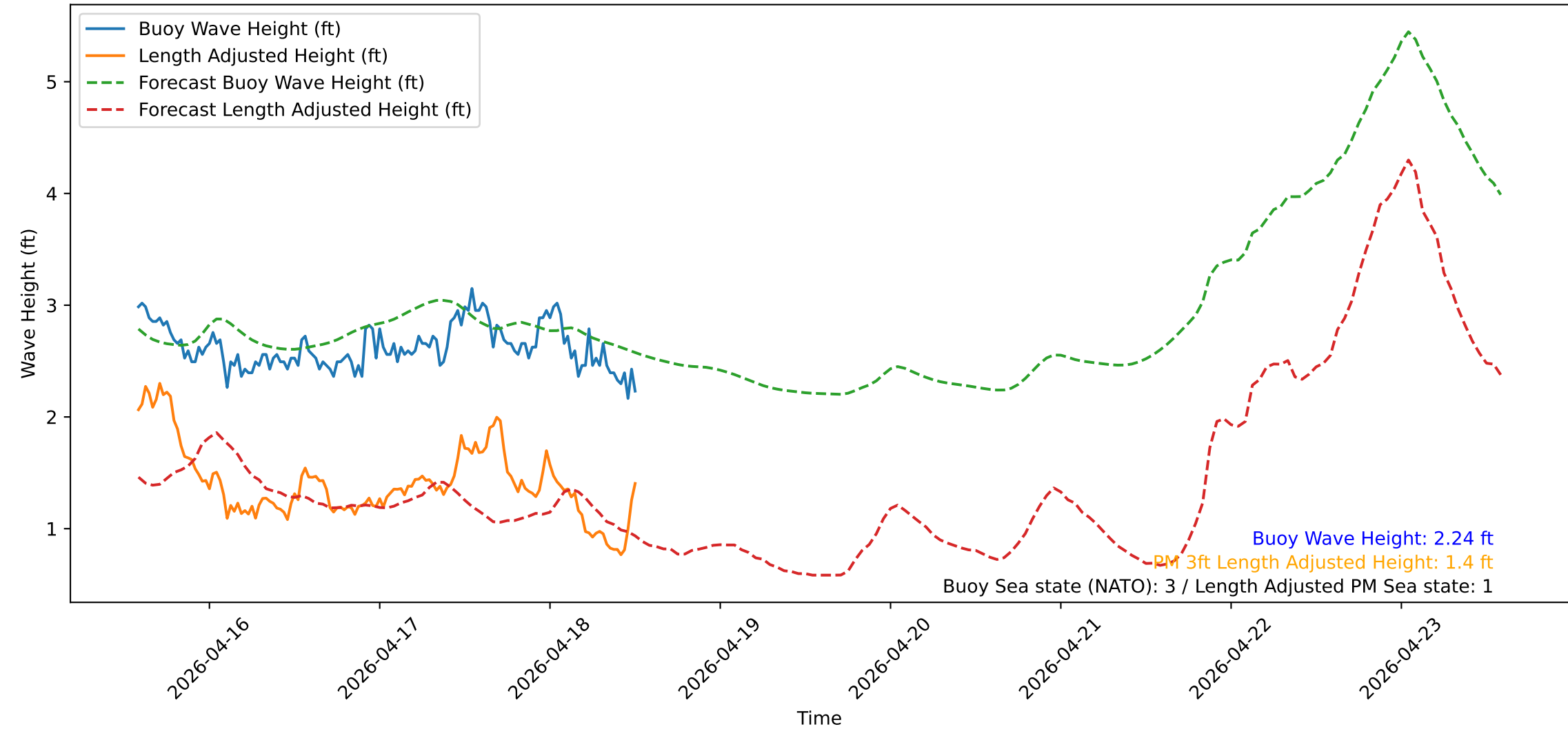
Wave Heights over Time for Red Beach at 2026-04-18 13:30:50
