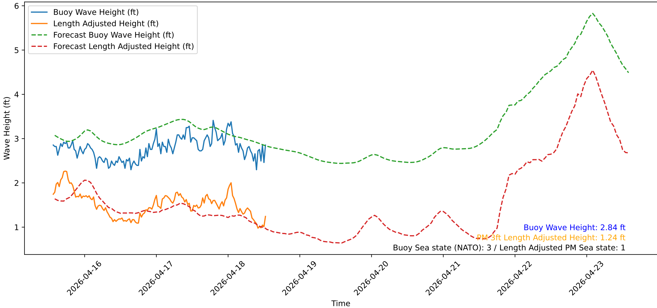
Wave Heights over Time for Oceanside Harbor at 2026-04-18 13:30:31
