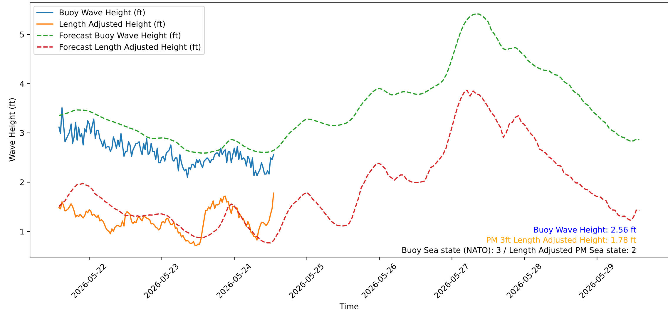
Wave Heights over Time for Oceanside Harbor at 2026-05-24 14:10:32
