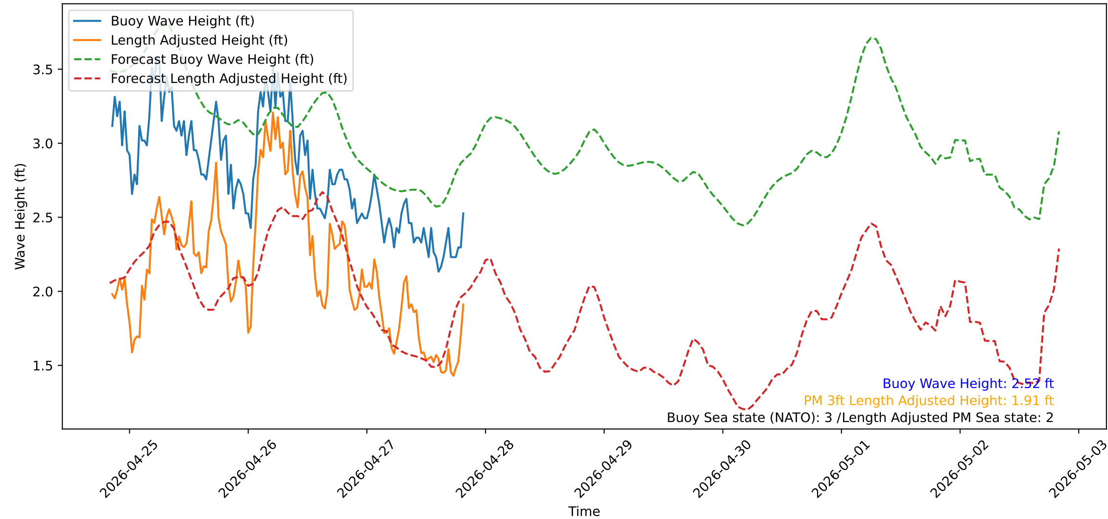
Wave Heights over Time for Green Beach at 2026-04-27 20:21:14
