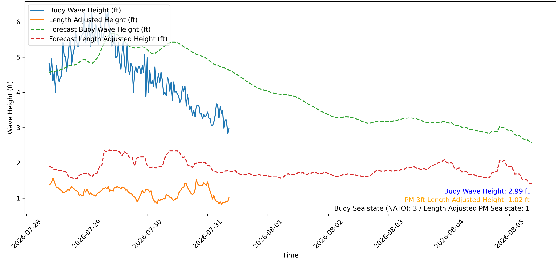
Wave Heights over Time for Green Beach at 2026-07-31 09:11:09
