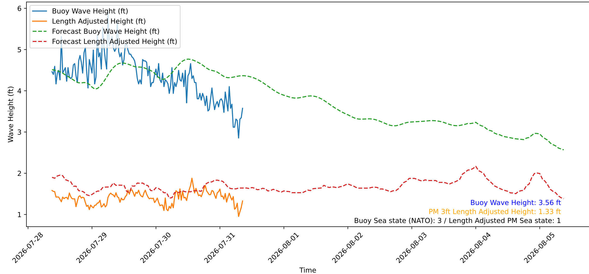
Wave Heights over Time for Oceanside Harbor at 2026-07-31 09:10:26
