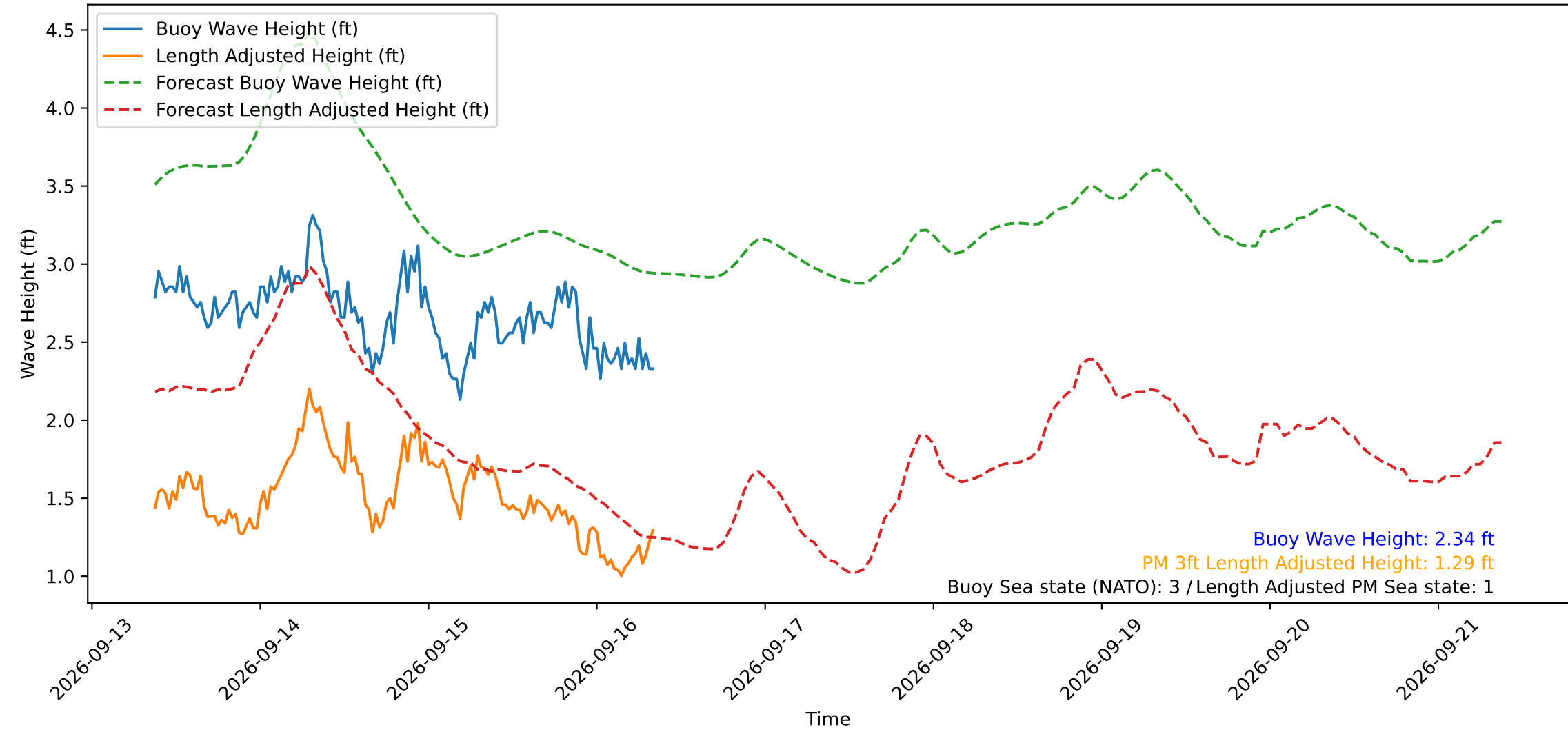
Wave Heights over Time for Green Beach at 2026-09-16 08:41:12
