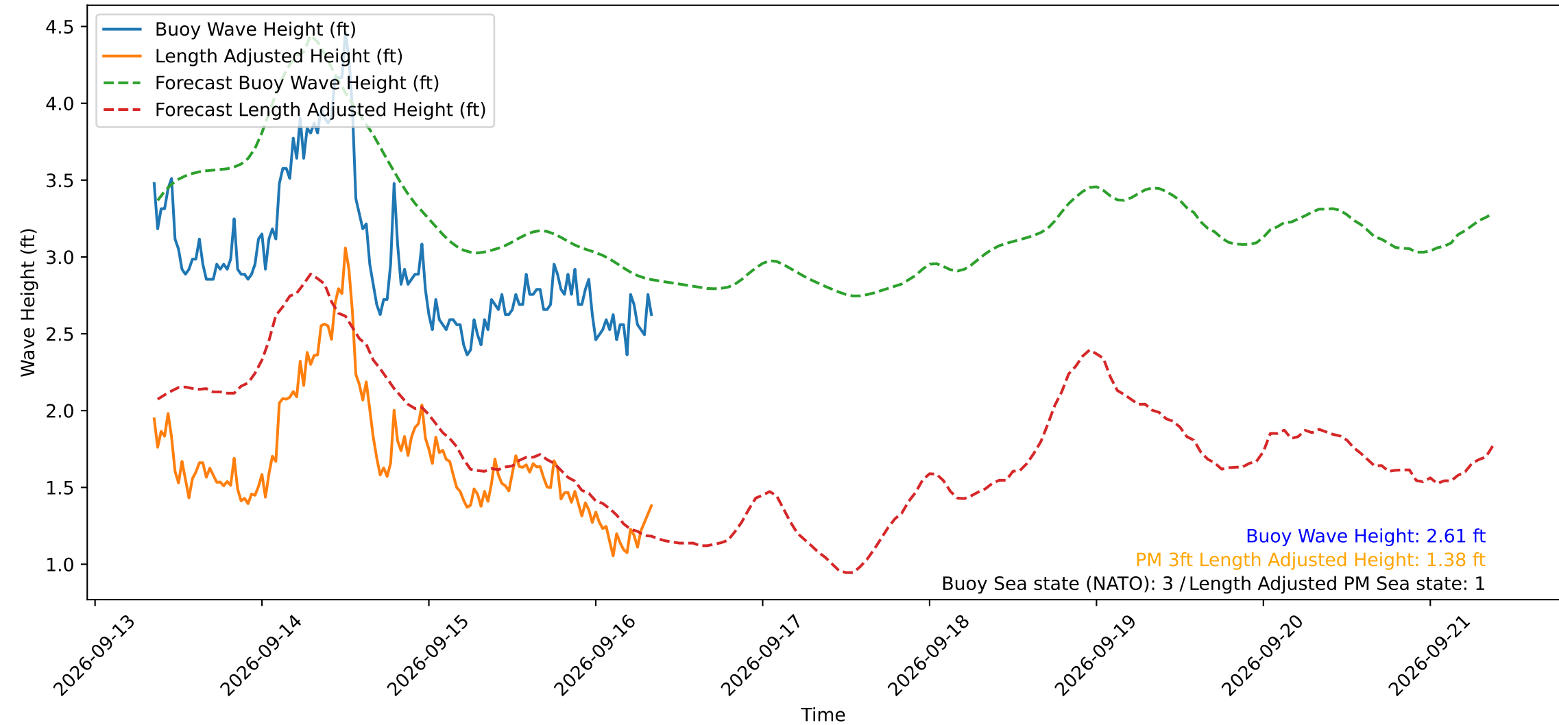
Wave Heights over Time for Oceanside Harbor at 2026-09-16 08:40:29
