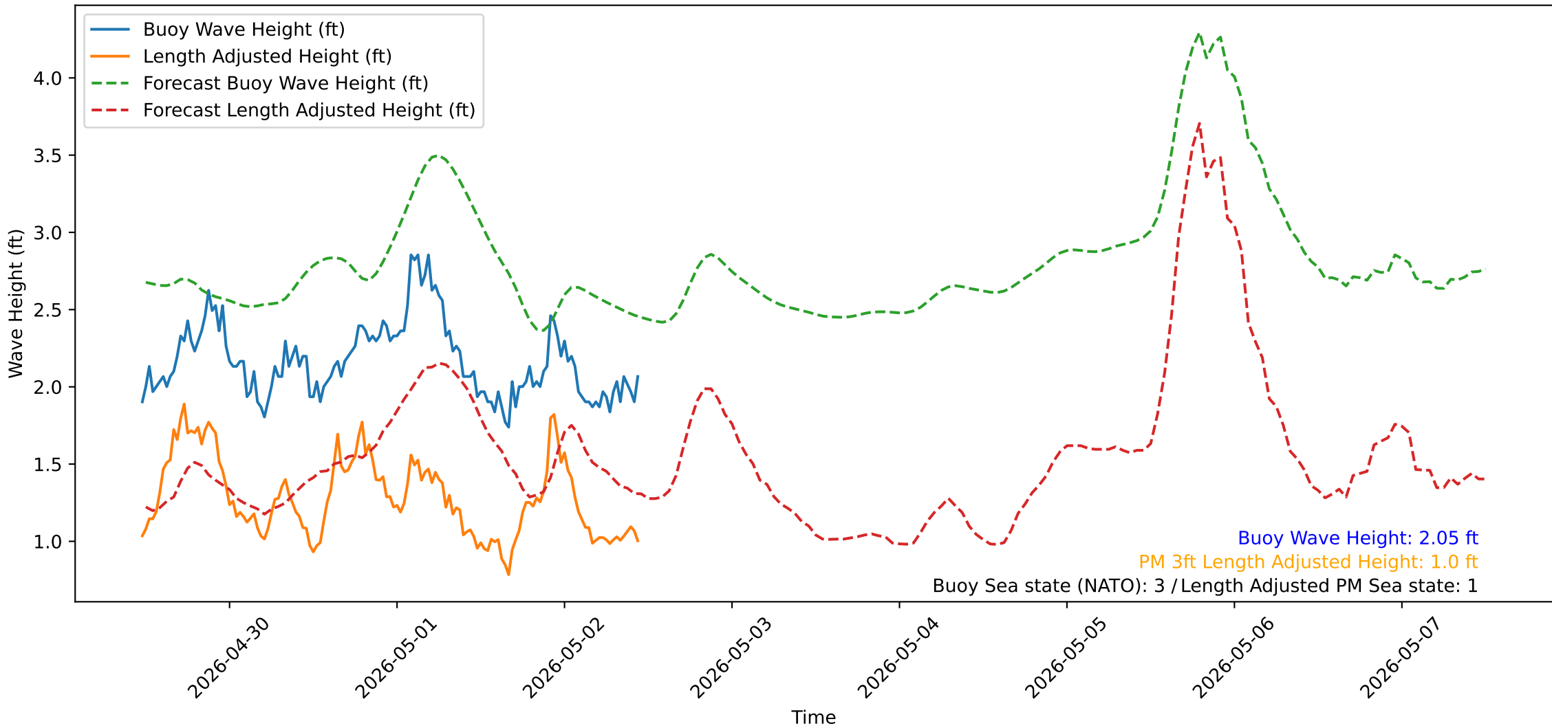
Wave Heights over Time for Green Beach at 2026-05-02 11:31:13
