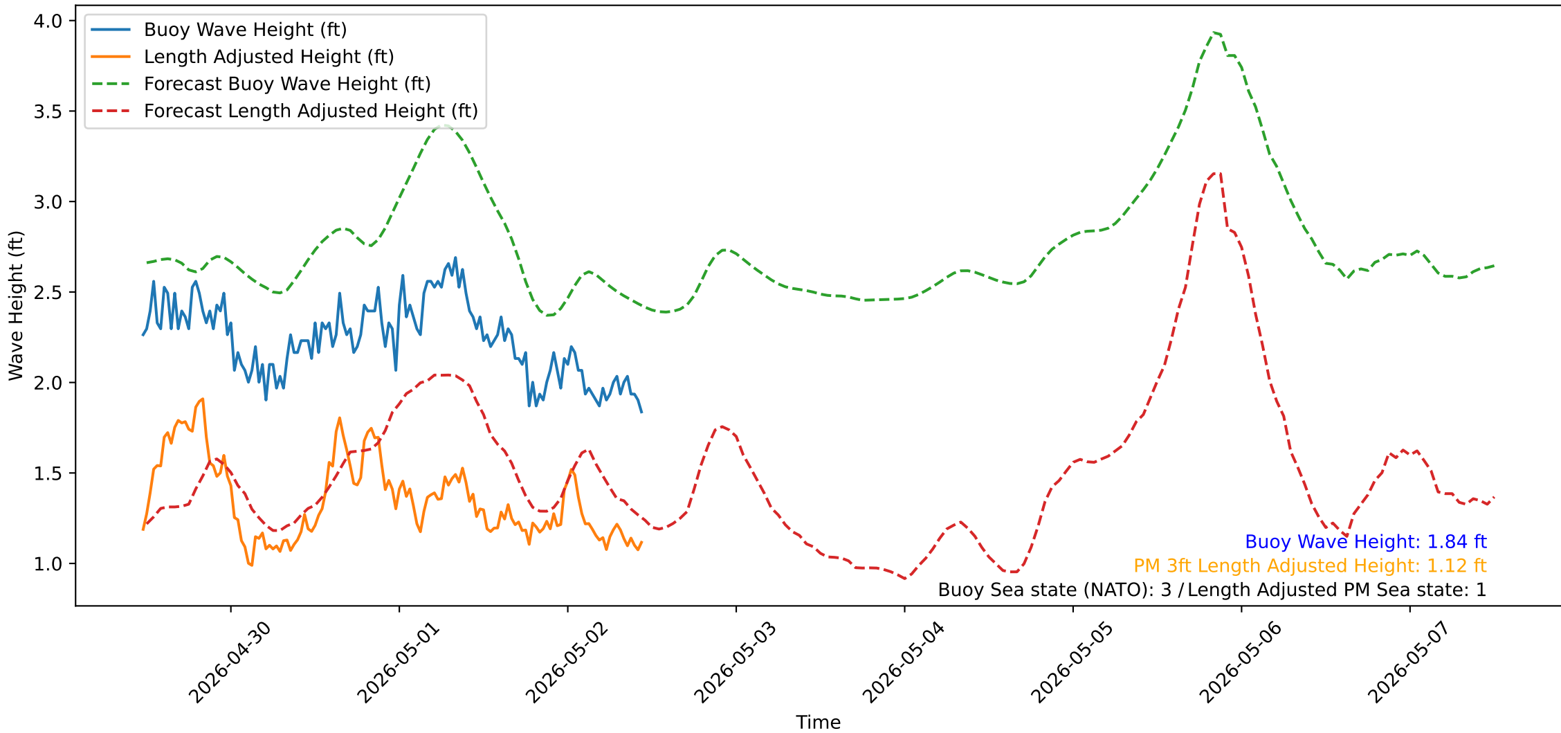
Wave Heights over Time for Oceanside Harbor at 2026-05-02 11:30:31
