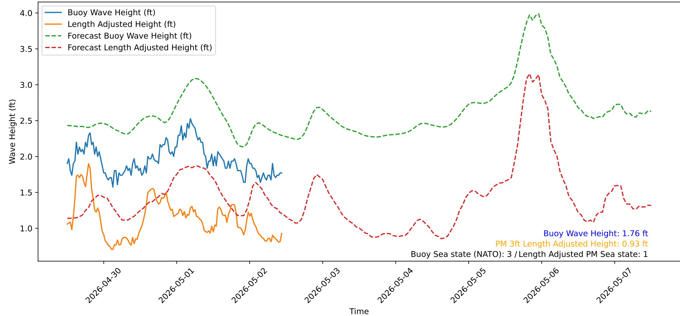
Wave Heights over Time for Red Beach at 2026-05-02 11:30:50
