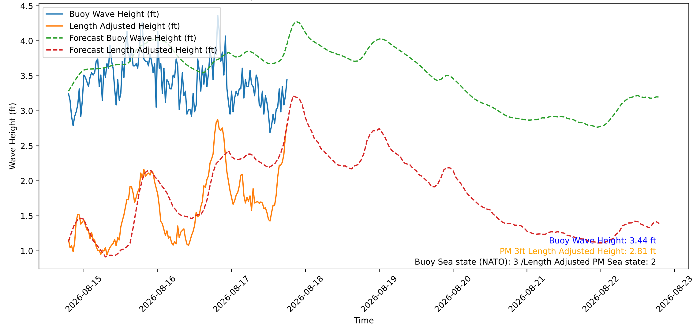
Wave Heights over Time for Green Beach at 2026-08-17 18:51:13
