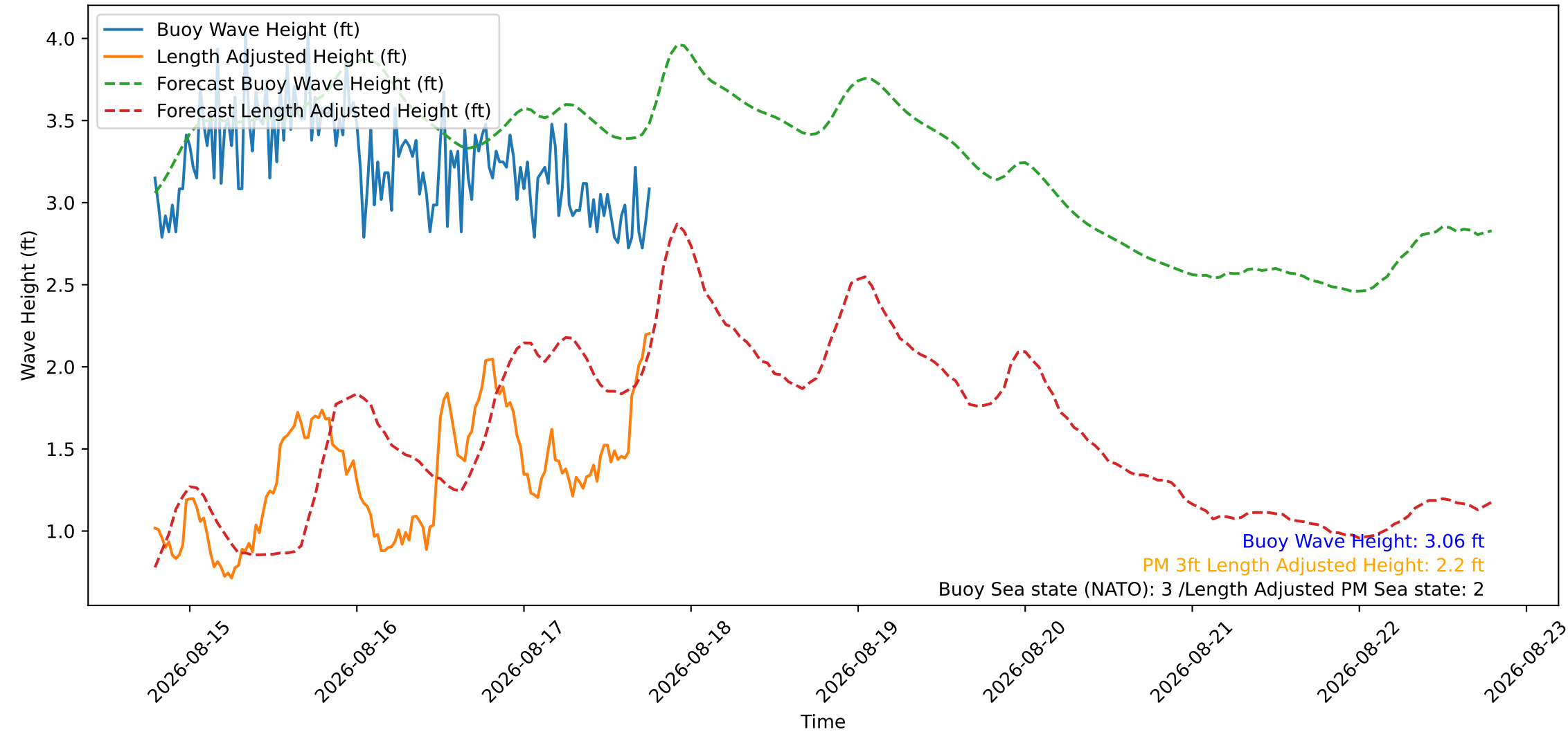
Wave Heights over Time for Red Beach at 2026-08-17 18:50:48
