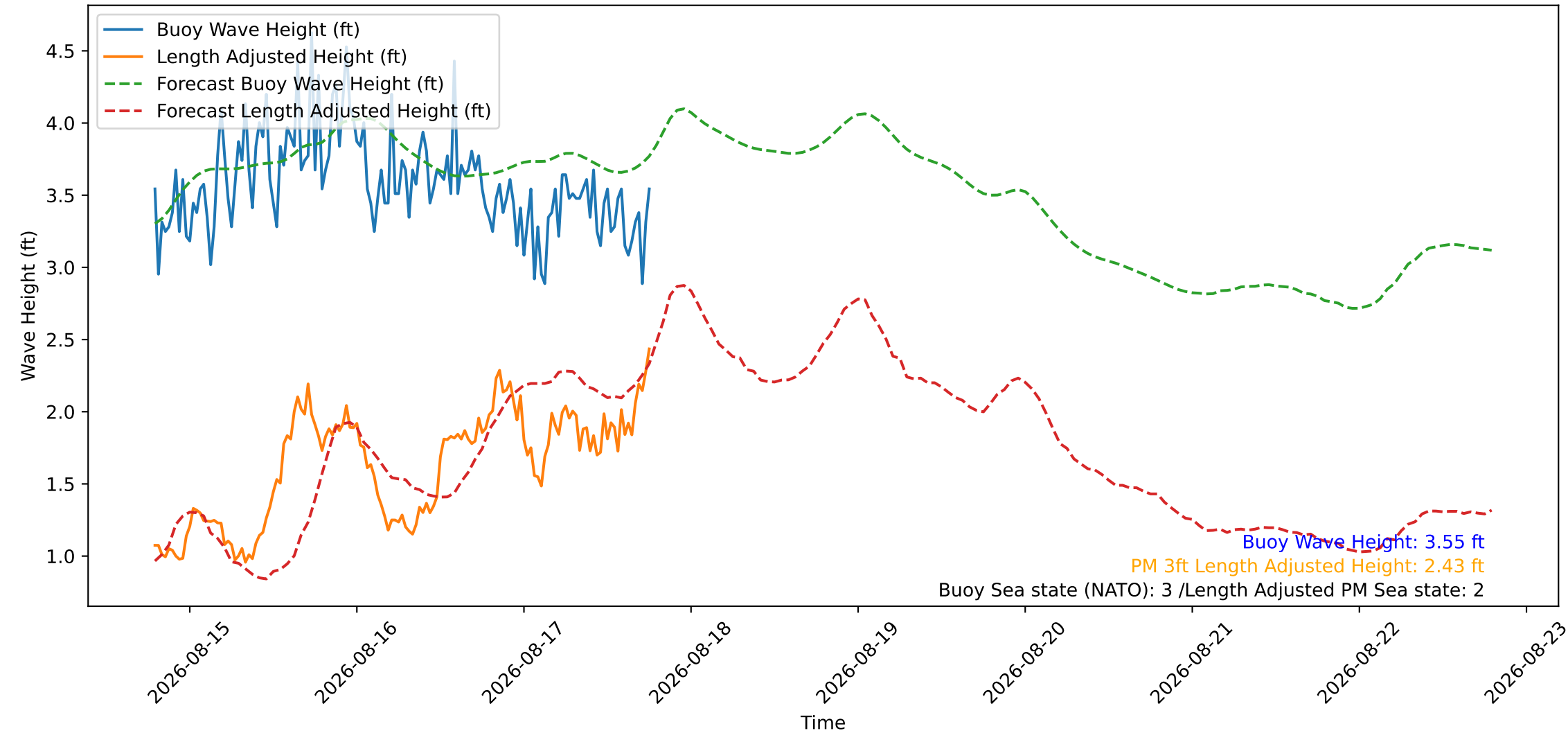
Wave Heights over Time for Oceanside Harbor at 2026-08-17 18:50:27
