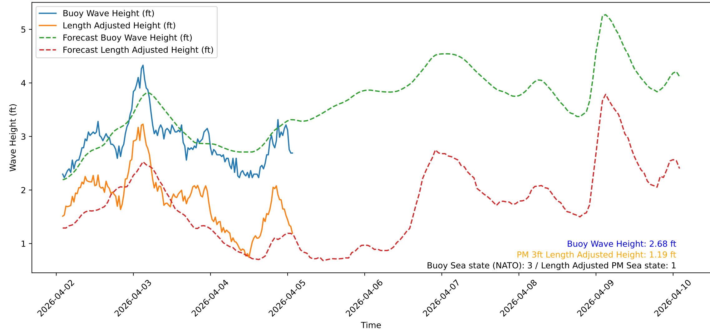
Wave Heights over Time for Green Beach at 2026-04-05 02:11:10
