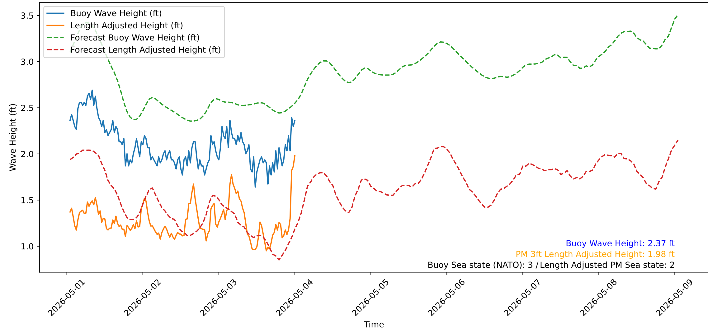
Wave Heights over Time for Oceanside Harbor at 2026-05-04 00:50:32
