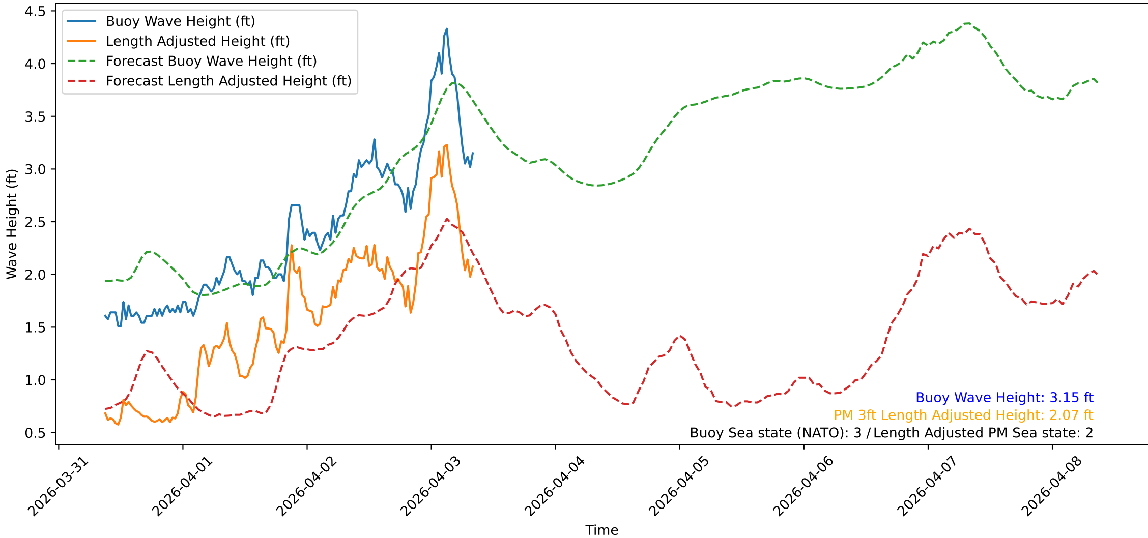
Wave Heights over Time for Green Beach at 2026-04-03 09:01:11
