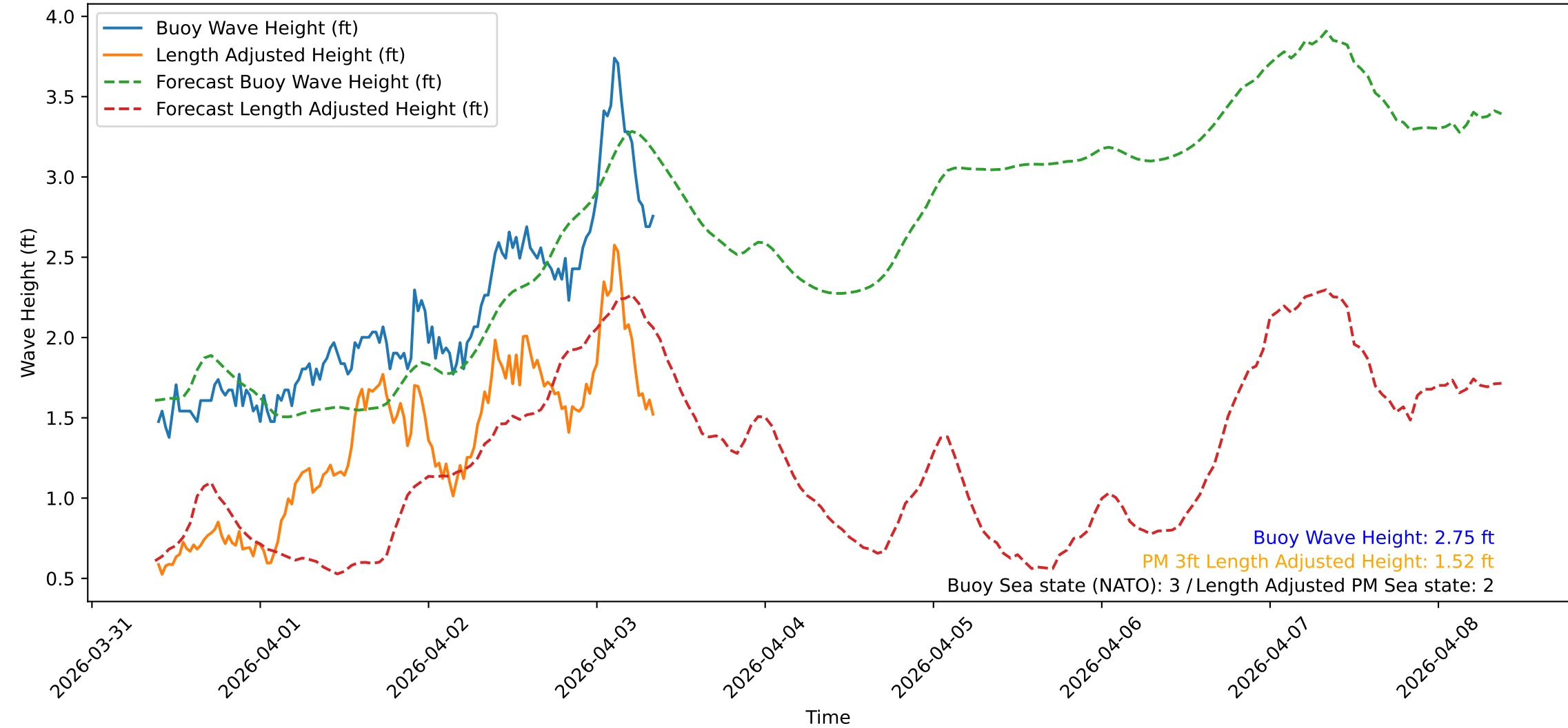
Wave Heights over Time for Red Beach at 2026-04-03 09:00:48
