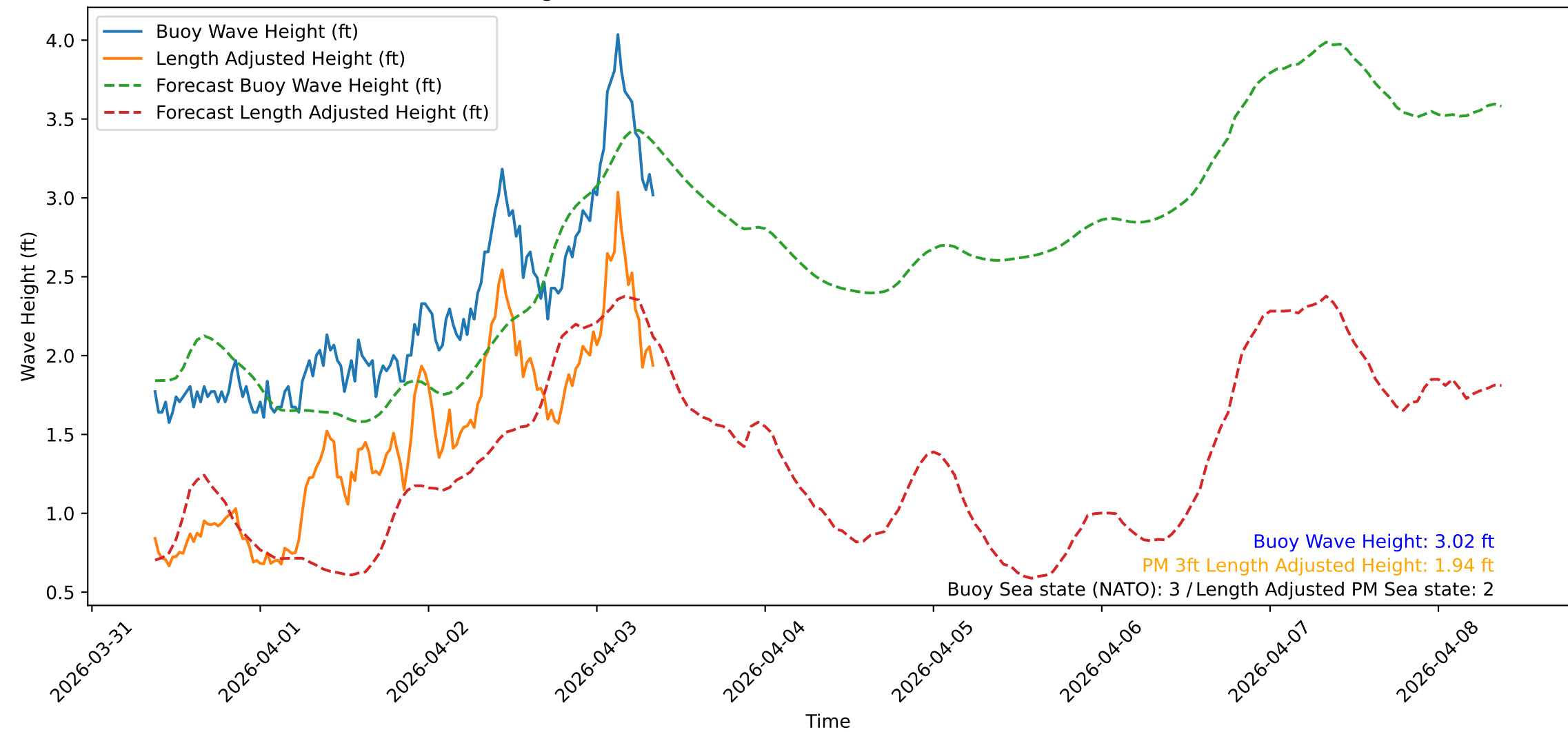
Wave Heights over Time for Oceanside Harbor at 2026-04-03 09:00:31
