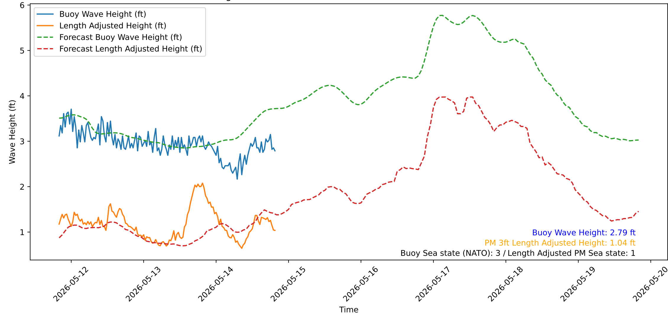
Wave Heights over Time for Oceanside Harbor at 2026-05-14 20:10:32
