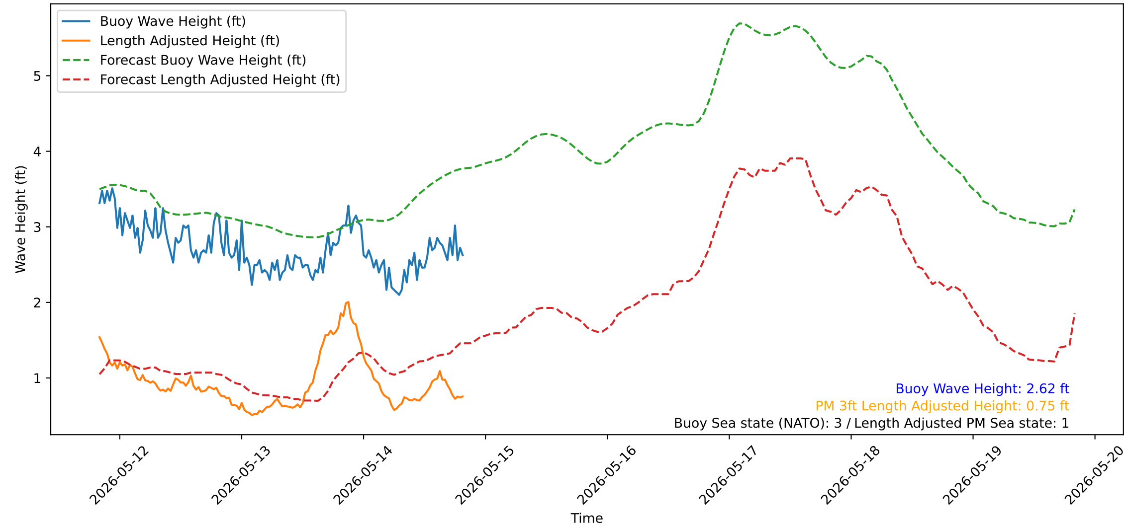
Wave Heights over Time for Green Beach at 2026-05-14 20:11:14
