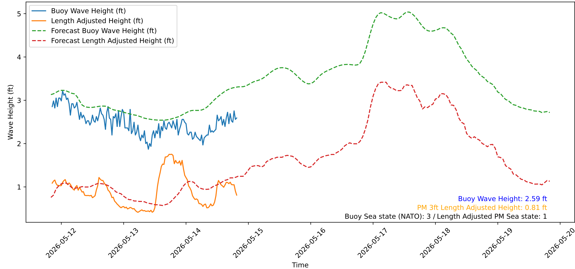
Wave Heights over Time for Red Beach at 2026-05-14 20:10:51
