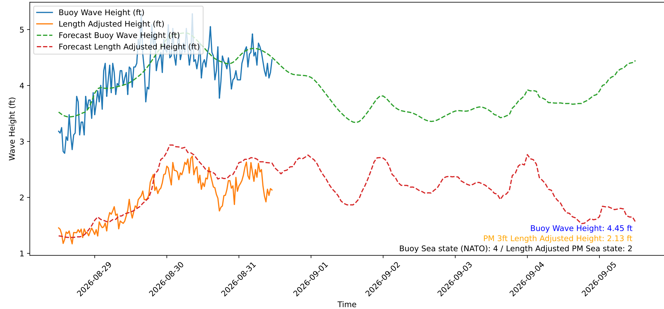
Wave Heights over Time for Oceanside Harbor at 2026-08-31 12:10:30
