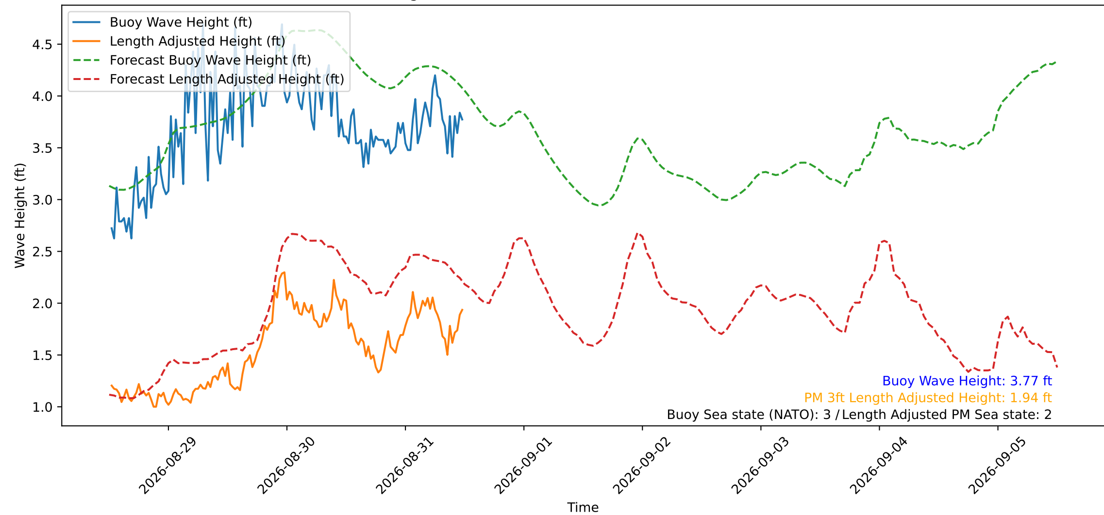
Wave Heights over Time for Red Beach at 2026-08-31 12:10:49
