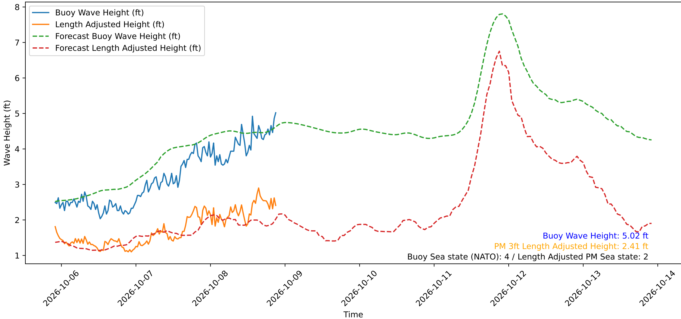
Wave Heights over Time for Oceanside Harbor at 2026-10-08 21:50:30
