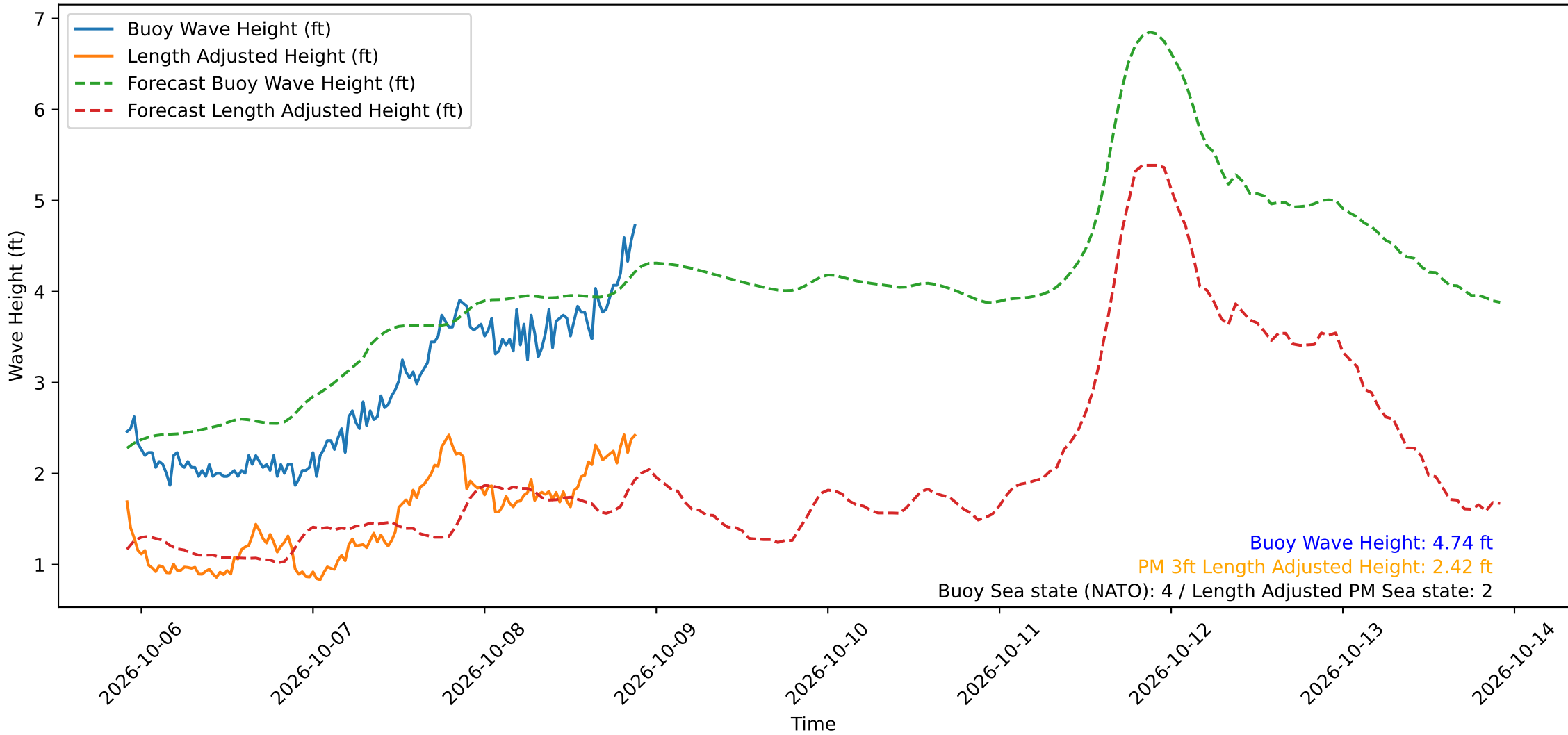
Wave Heights over Time for Red Beach at 2026-10-08 21:50:50
