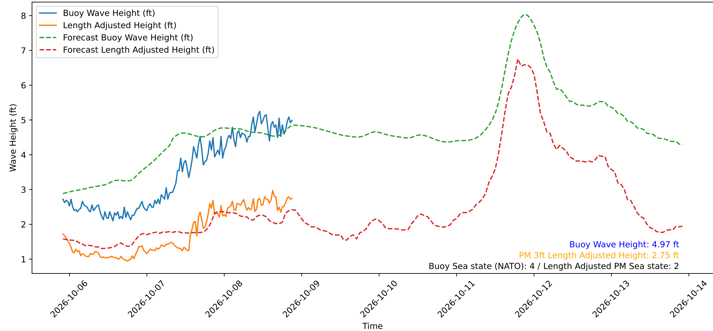
Wave Heights over Time for Green Beach at 2026-10-08 21:51:14
