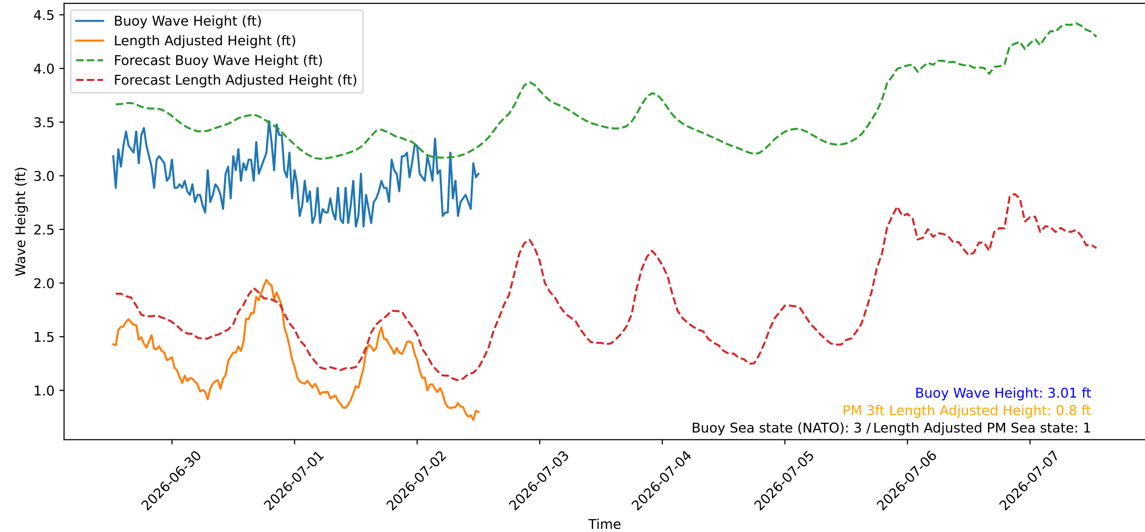
Wave Heights over Time for Green Beach at 2026-07-02 12:41:09
