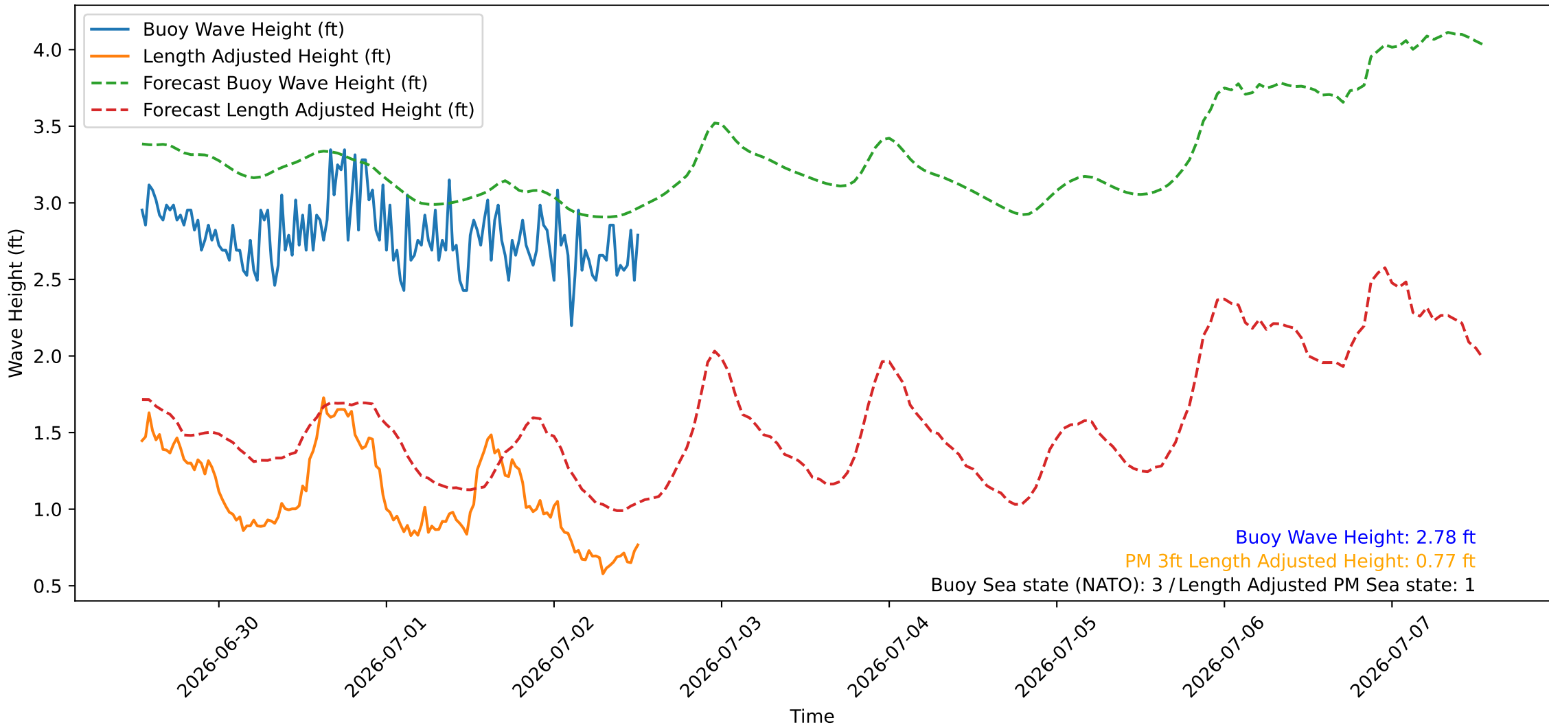
Wave Heights over Time for Red Beach at 2026-07-02 12:40:46
