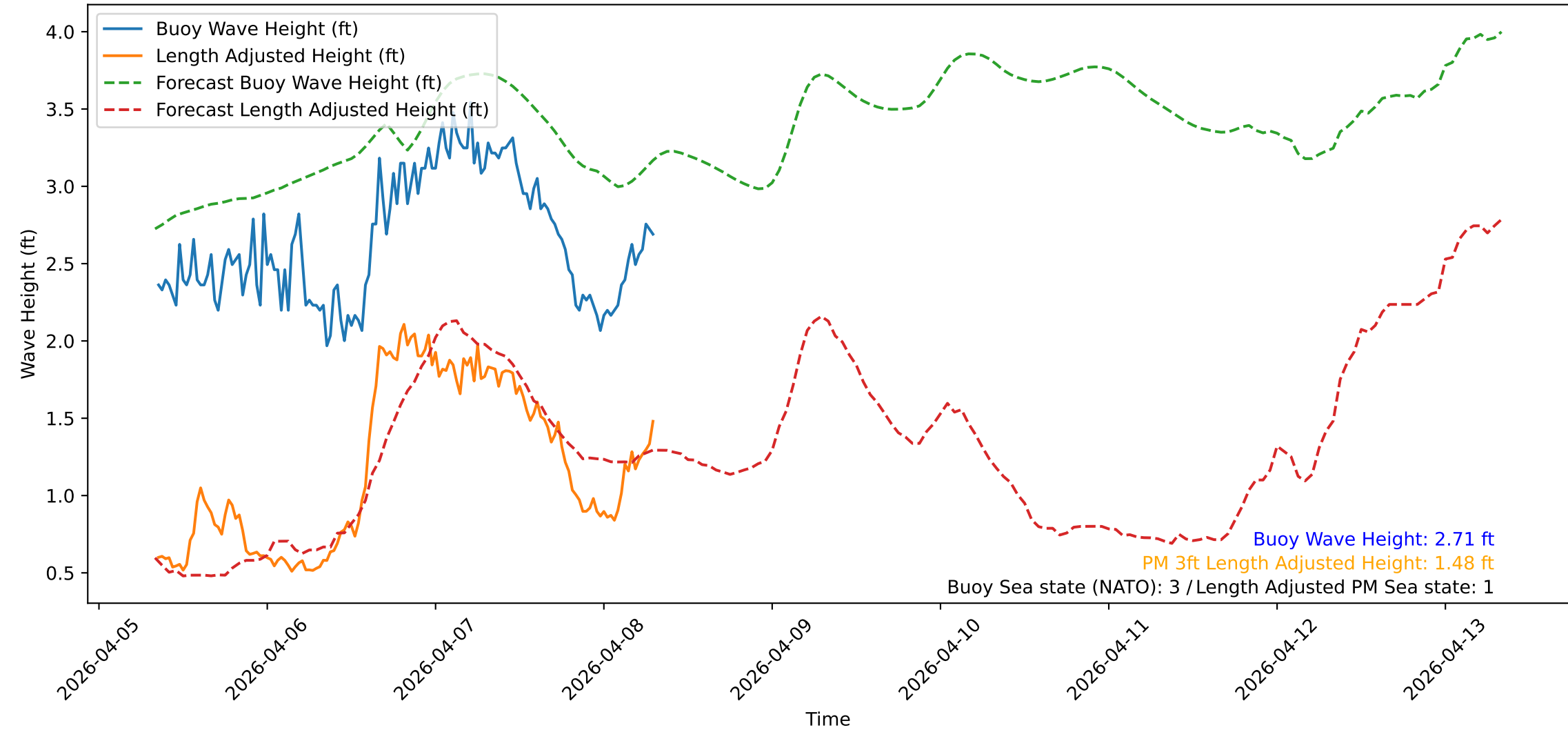
Wave Heights over Time for Red Beach at 2026-04-08 08:00:47
