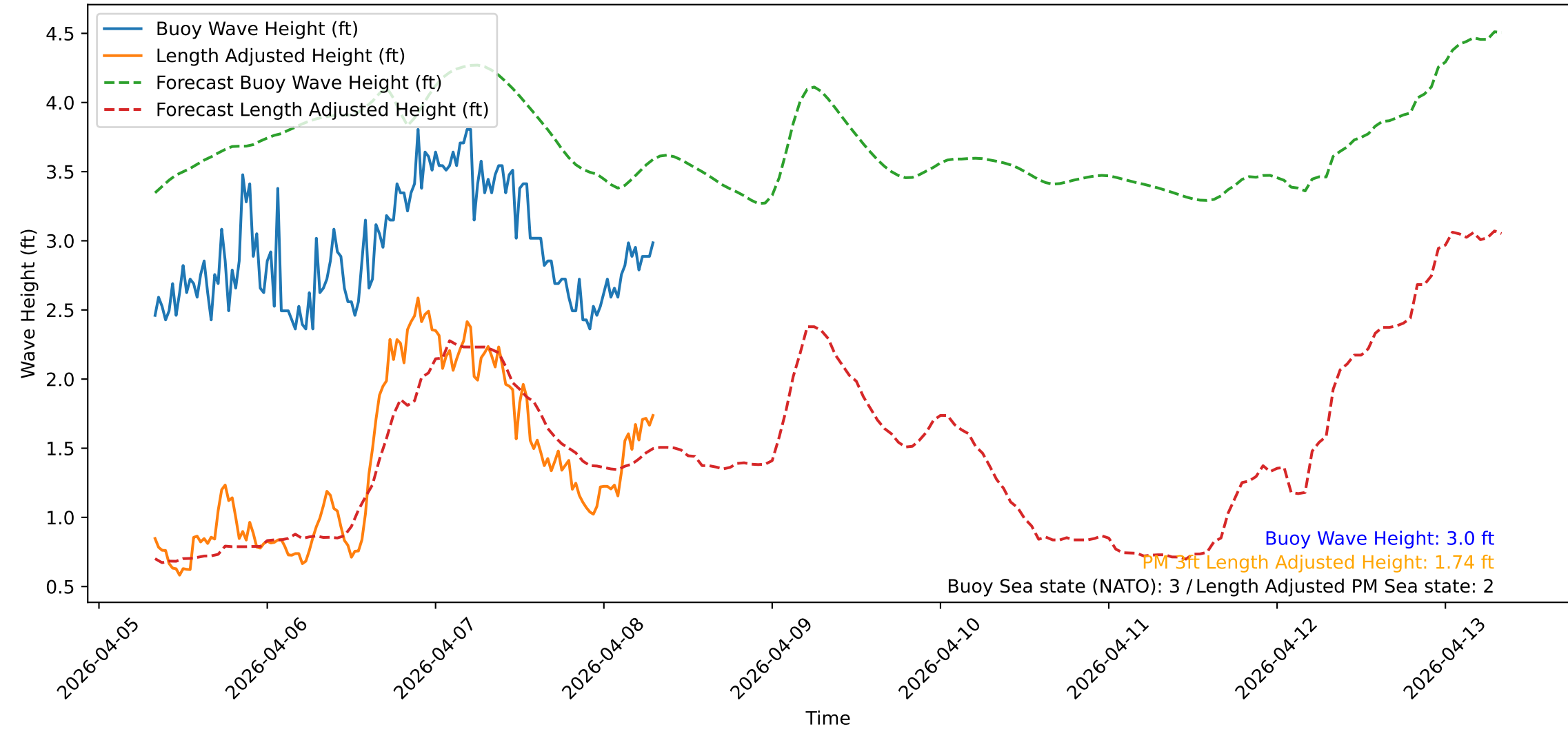
Wave Heights over Time for Green Beach at 2026-04-08 08:01:08
