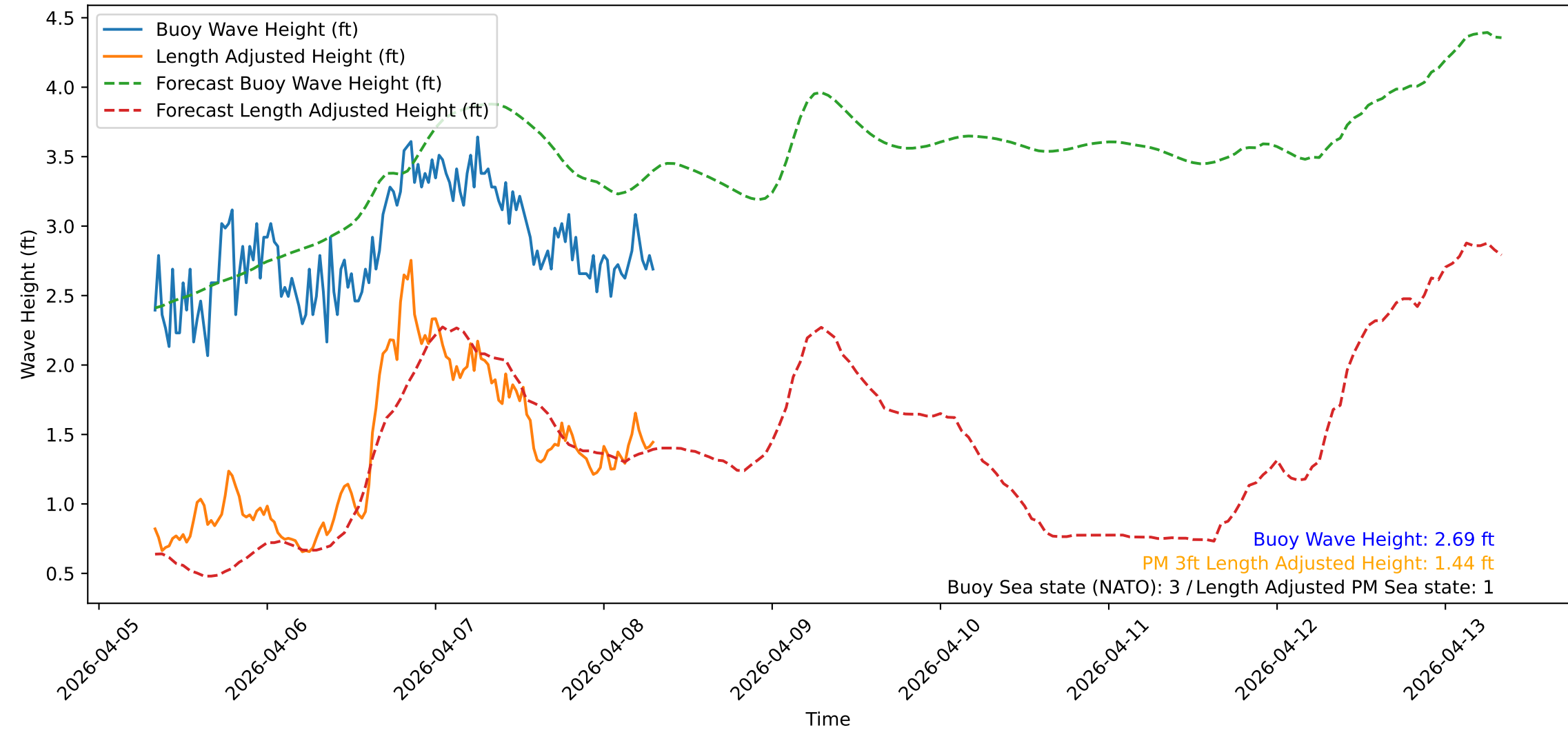
Wave Heights over Time for Oceanside Harbor at 2026-04-08 08:00:31
