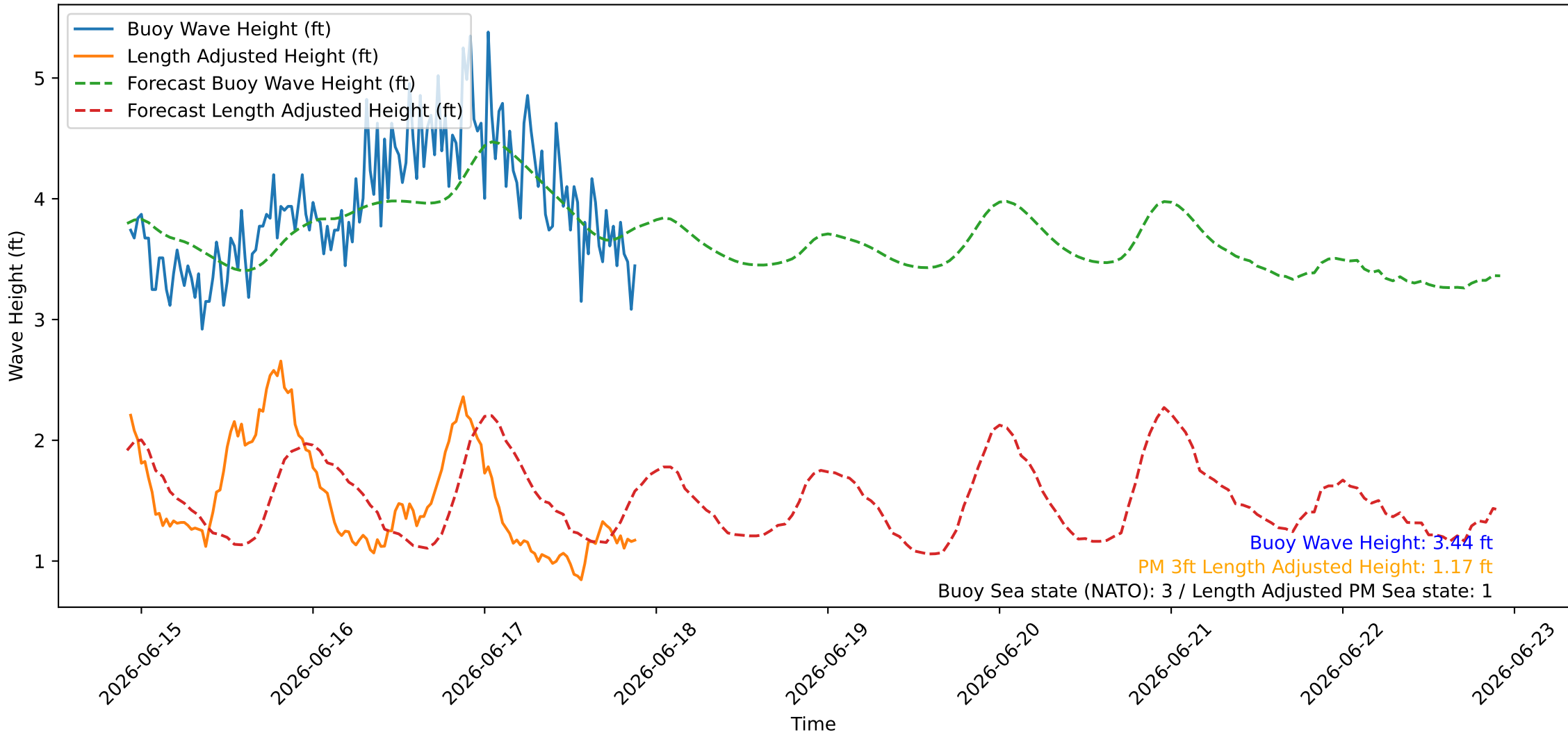
Wave Heights over Time for Red Beach at 2026-06-17 22:00:45
