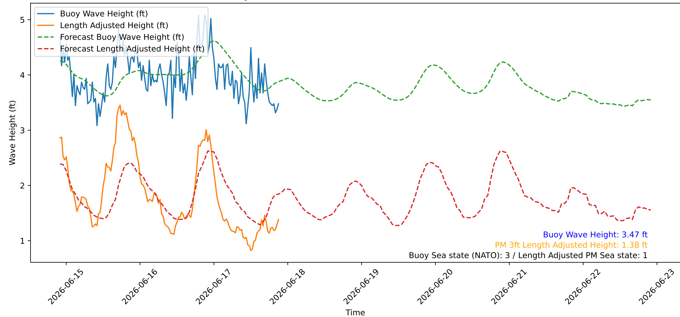
Wave Heights over Time for Green Beach at 2026-06-17 22:01:07
