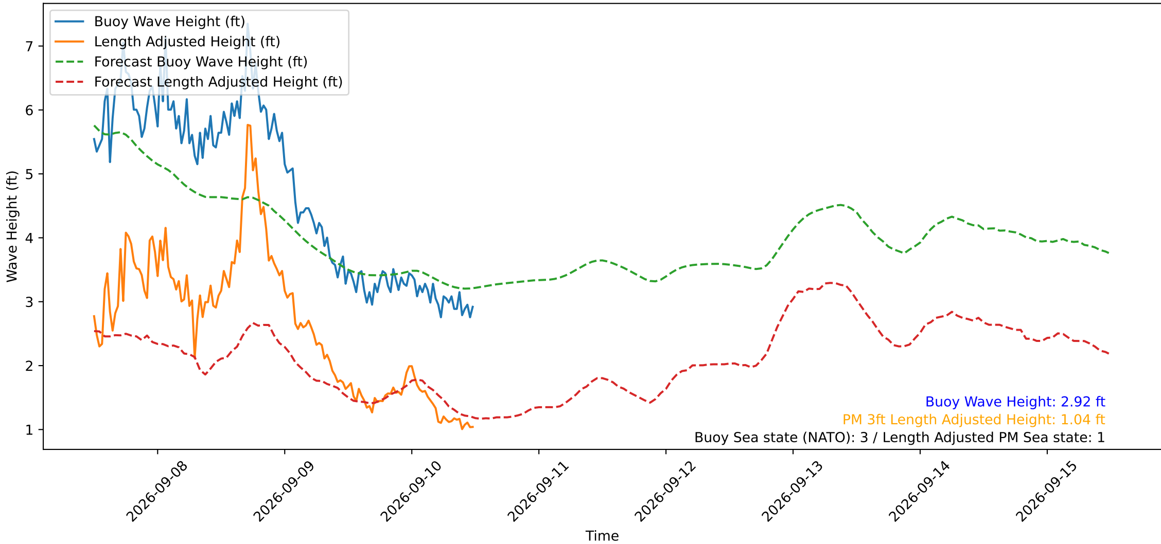
Wave Heights over Time for Oceanside Harbor at 2026-09-10 12:10:30
