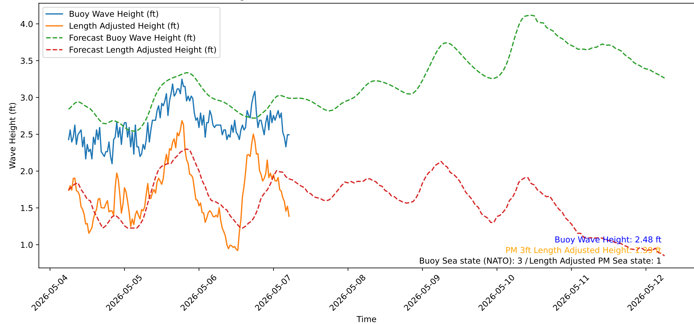
Wave Heights over Time for Oceanside Harbor at 2026-05-07 06:00:31
