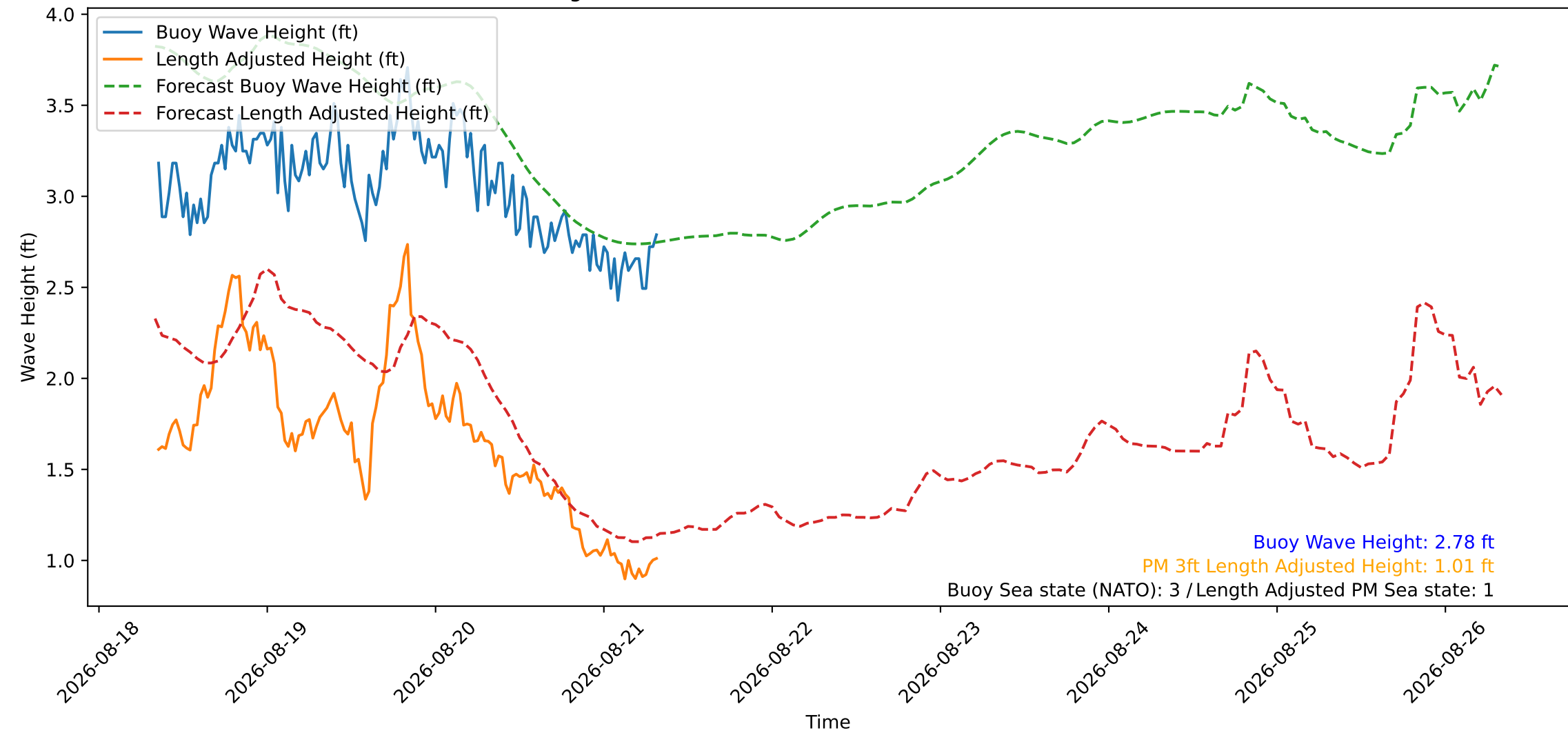
Wave Heights over Time for Green Beach at 2026-08-21 08:21:10
