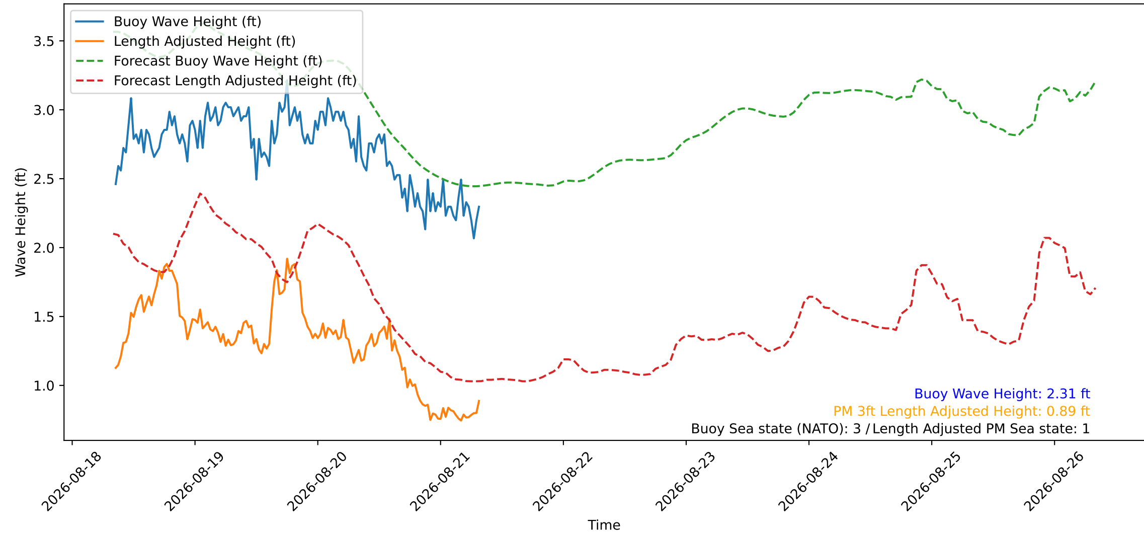
Wave Heights over Time for Red Beach at 2026-08-21 08:20:47
