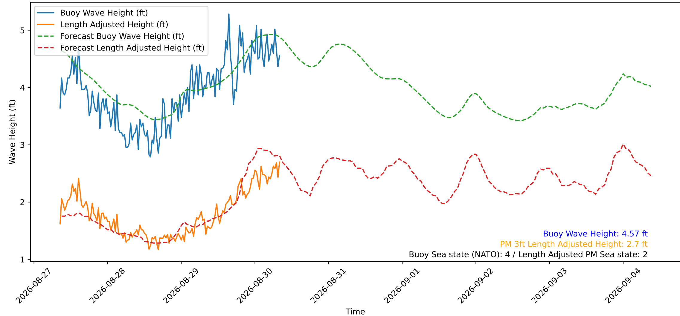
Wave Heights over Time for Oceanside Harbor at 2026-08-30 08:40:29
