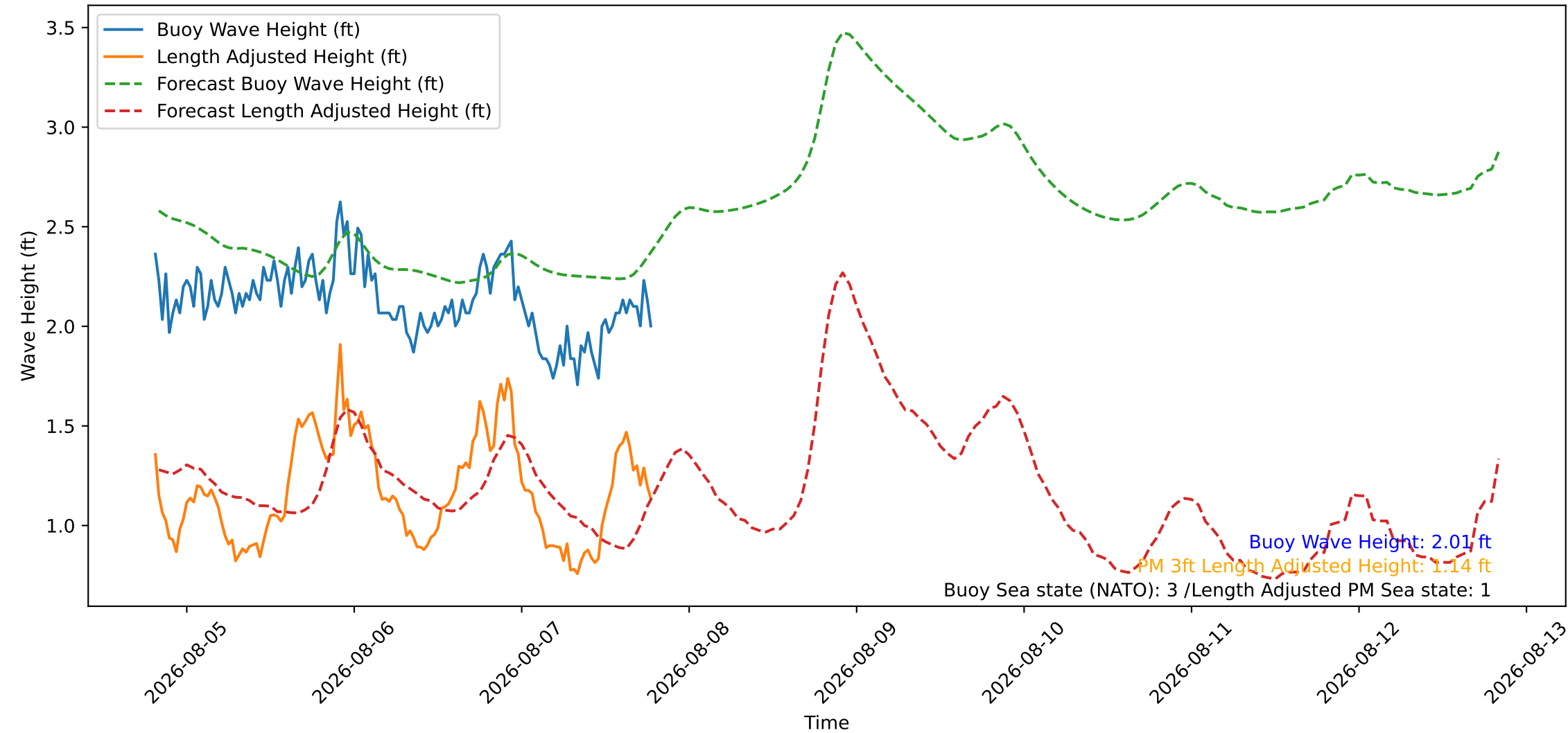
Wave Heights over Time for Green Beach at 2026-08-07 19:31:09
