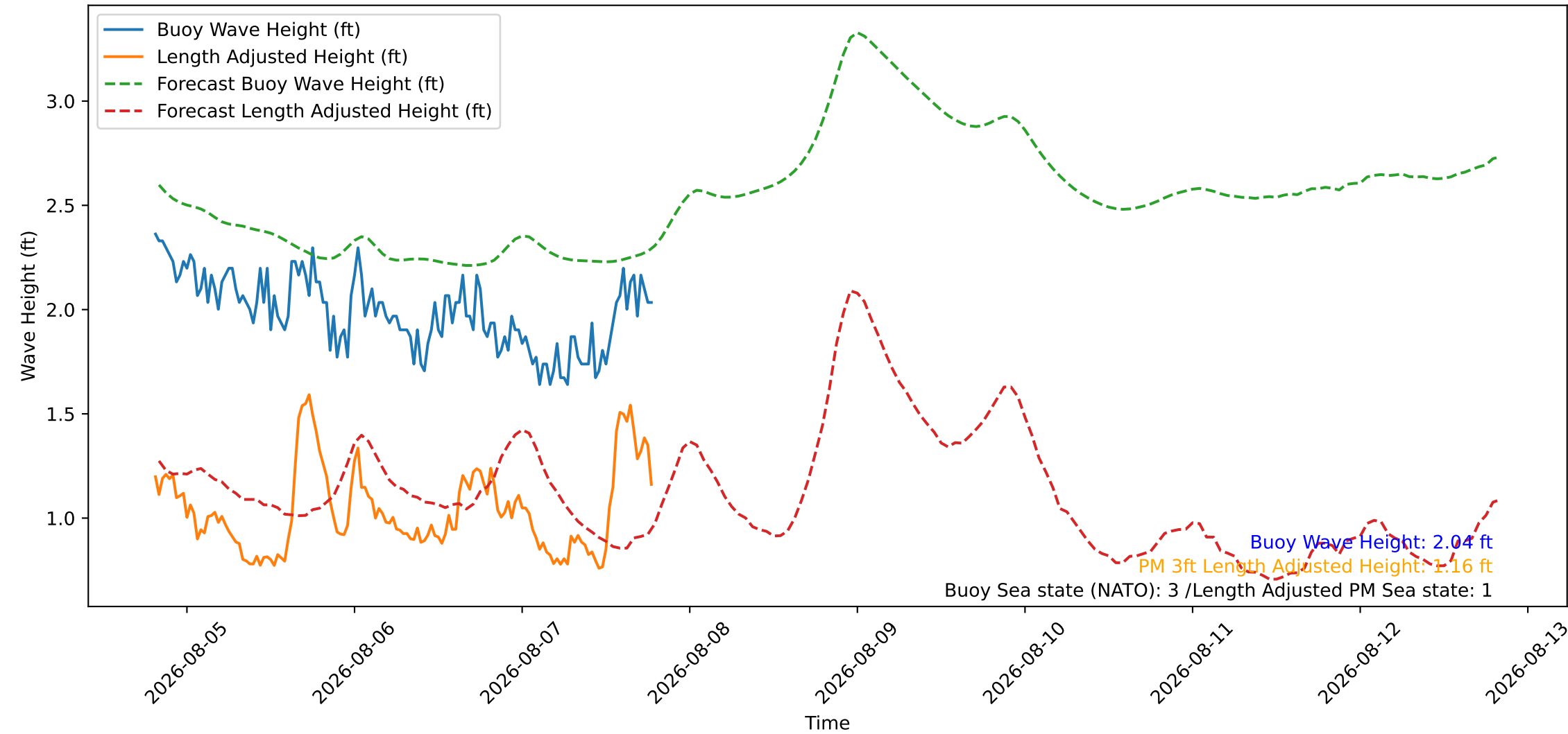
Wave Heights over Time for Oceanside Harbor at 2026-08-07 19:30:26
