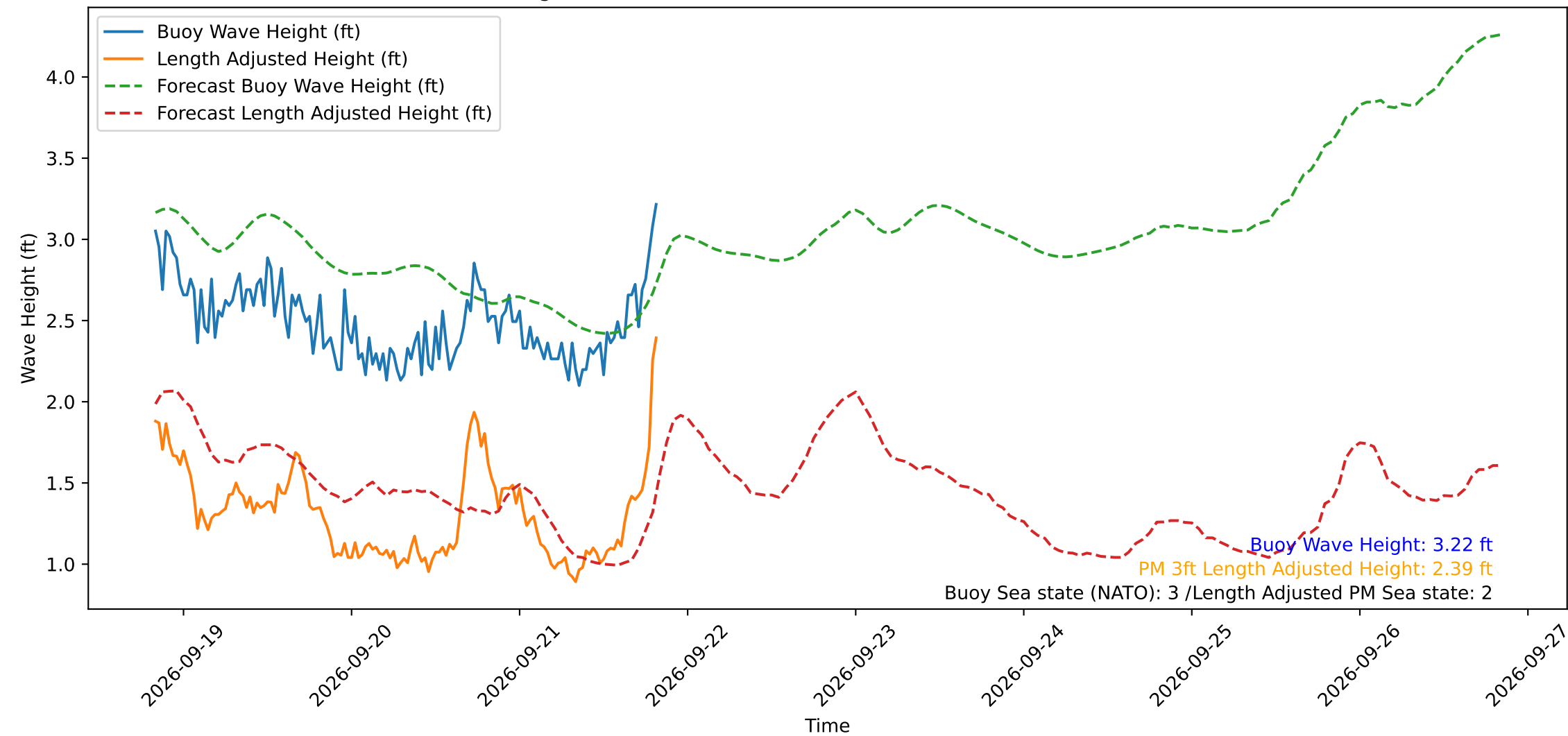
Wave Heights over Time for Oceanside Harbor at 2026-09-21 20:10:29
