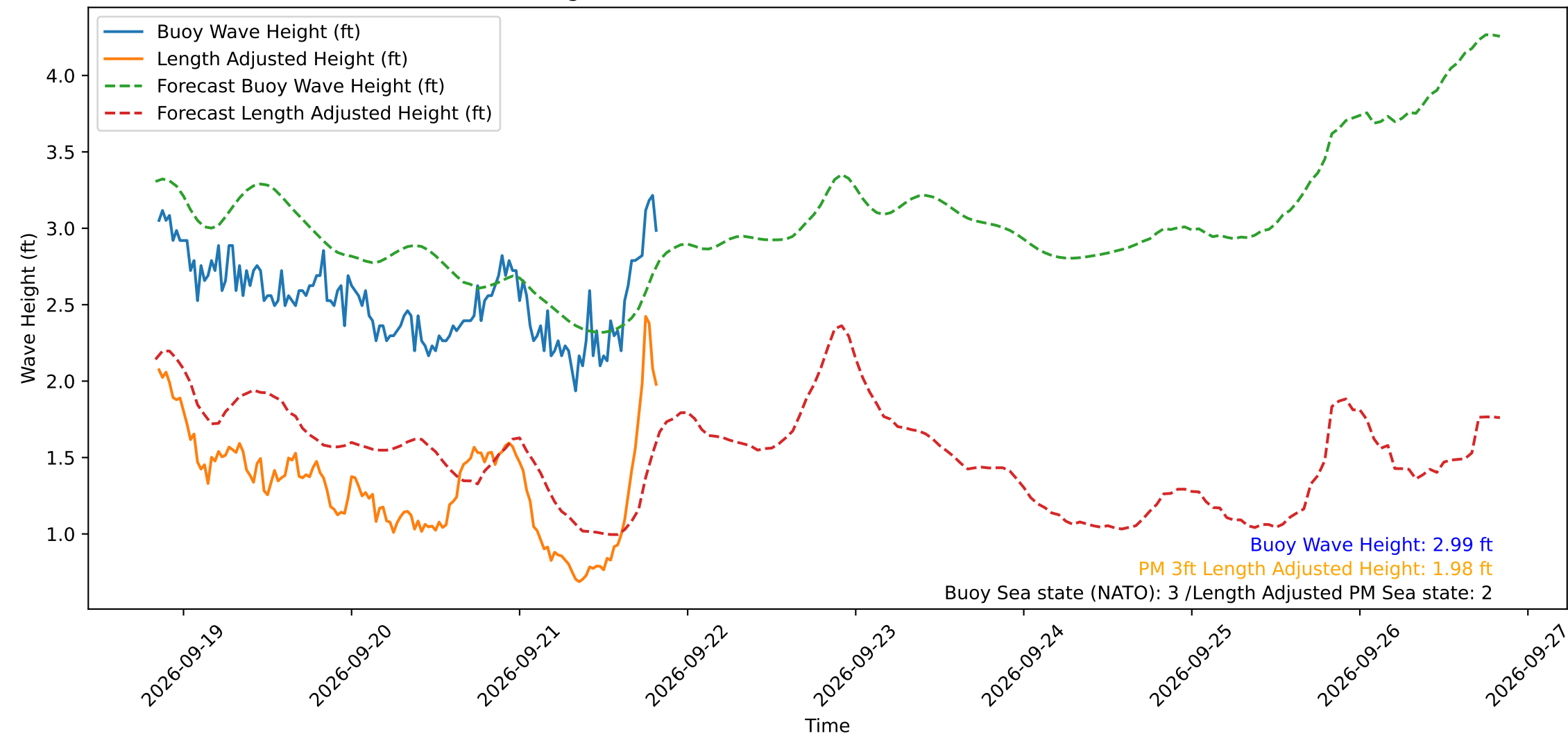
Wave Heights over Time for Green Beach at 2026-09-21 20:11:11
