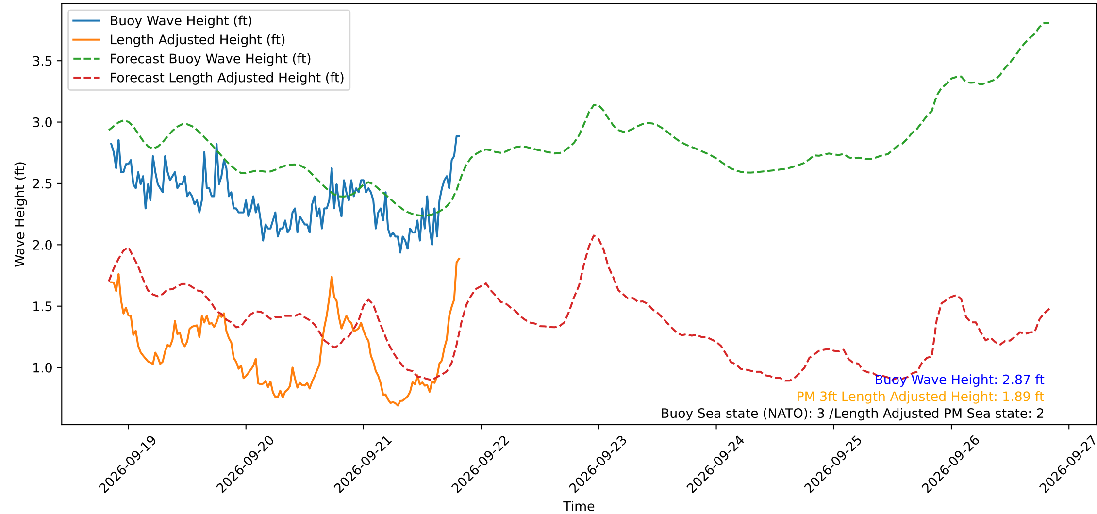
Wave Heights over Time for Red Beach at 2026-09-21 20:10:49
