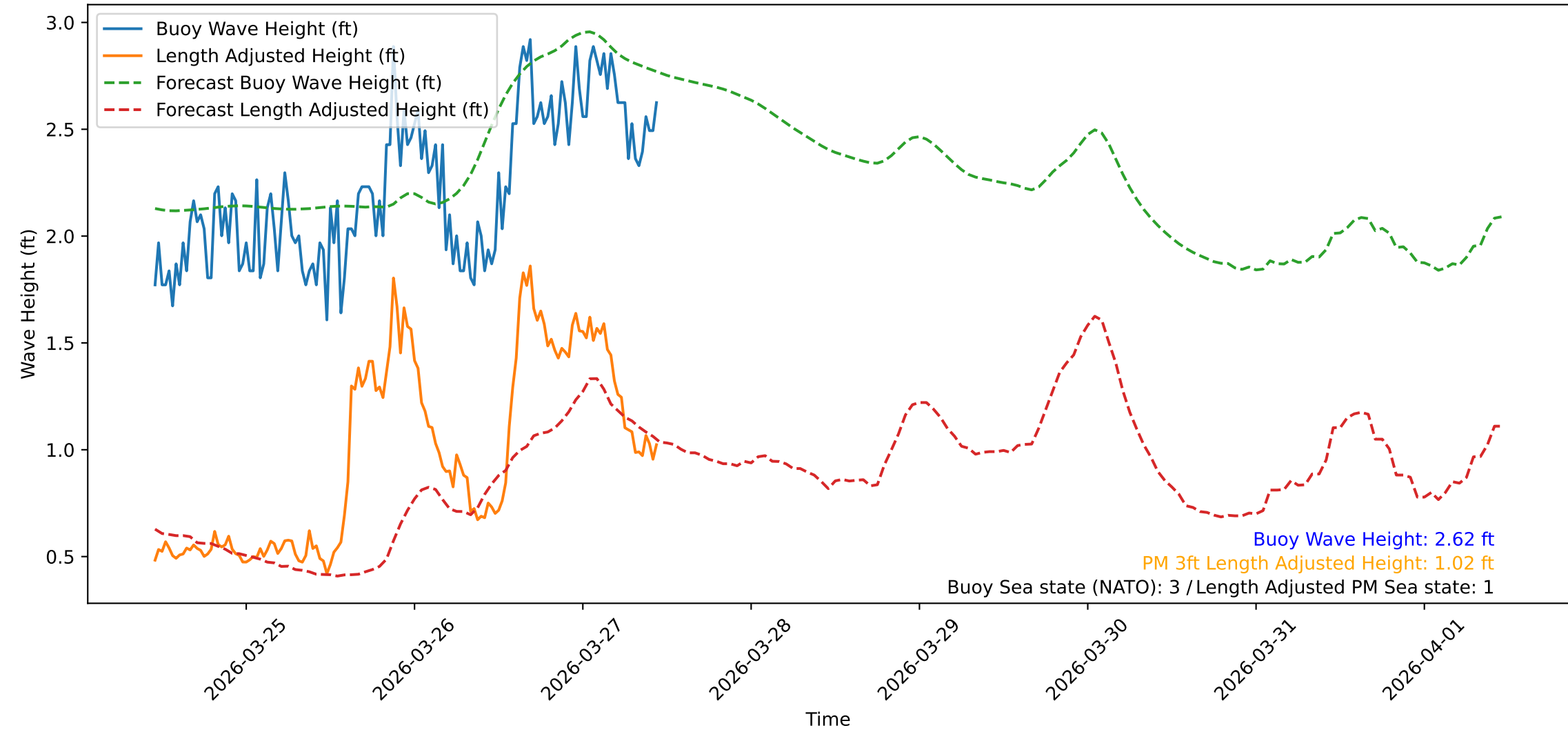
Wave Heights over Time for Oceanside Harbor at 2026-03-27 11:10:32
