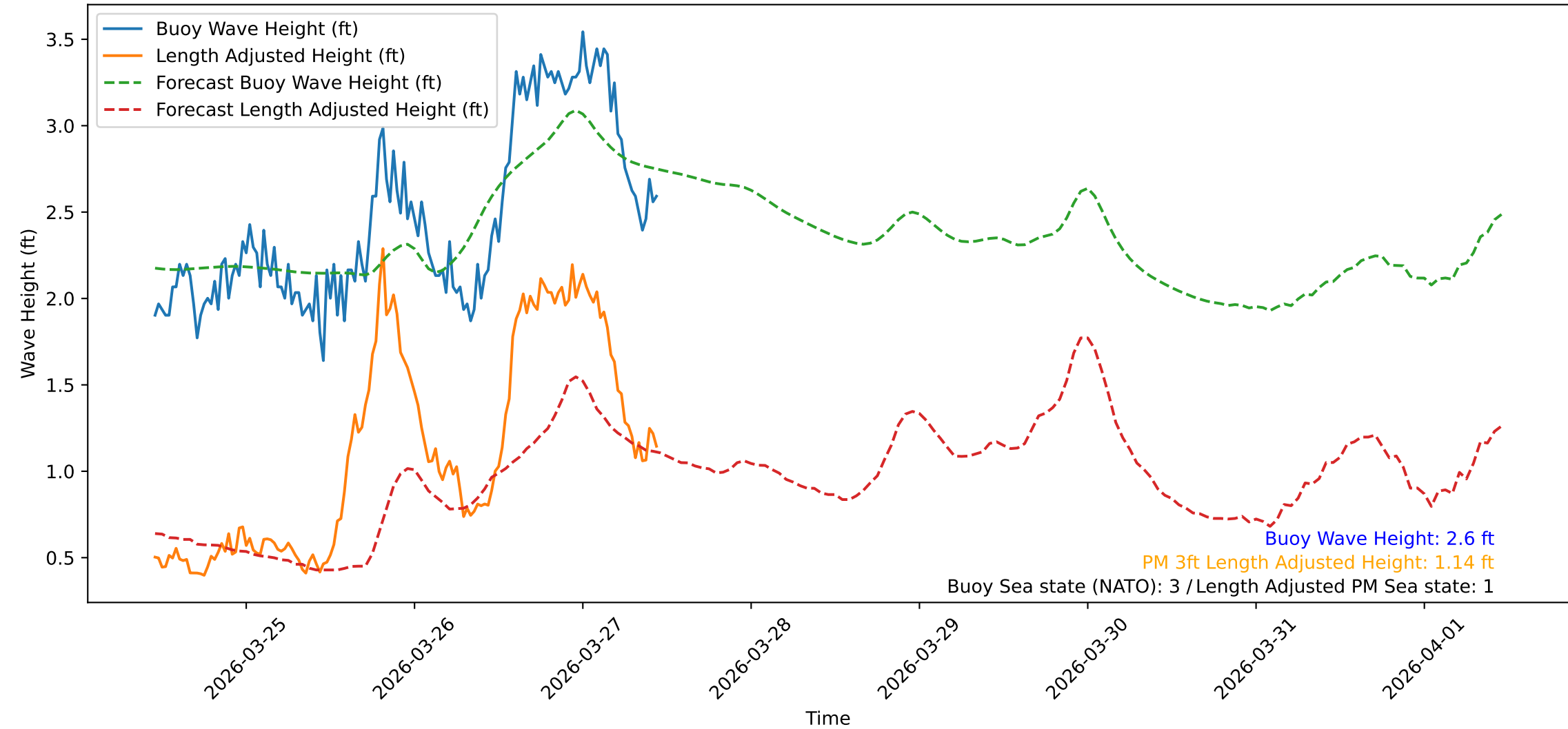
Wave Heights over Time for Green Beach at 2026-03-27 11:11:09
