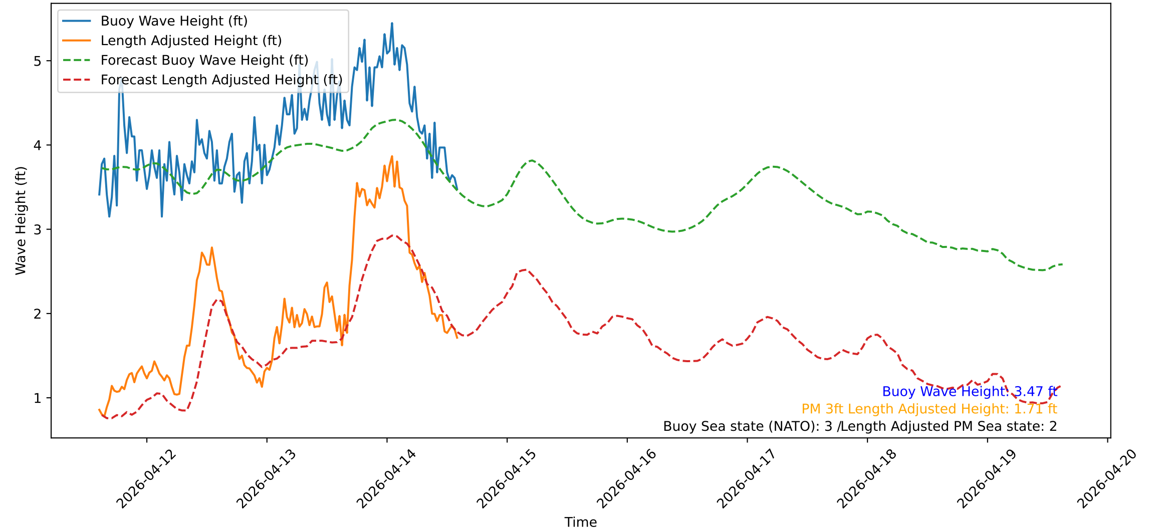
Wave Heights over Time for Oceanside Harbor at 2026-04-14 14:40:31
