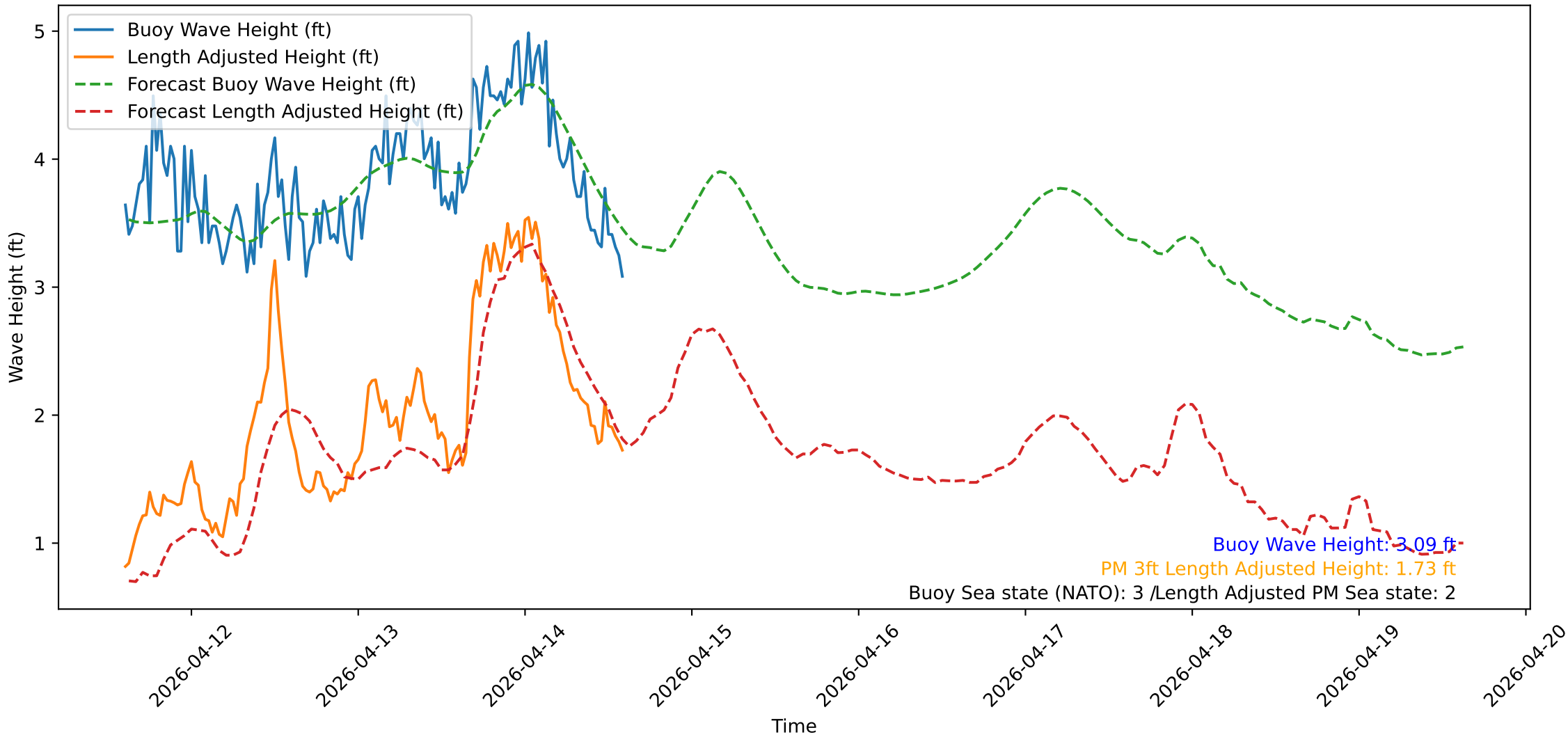
Wave Heights over Time for Green Beach at 2026-04-14 14:41:12
