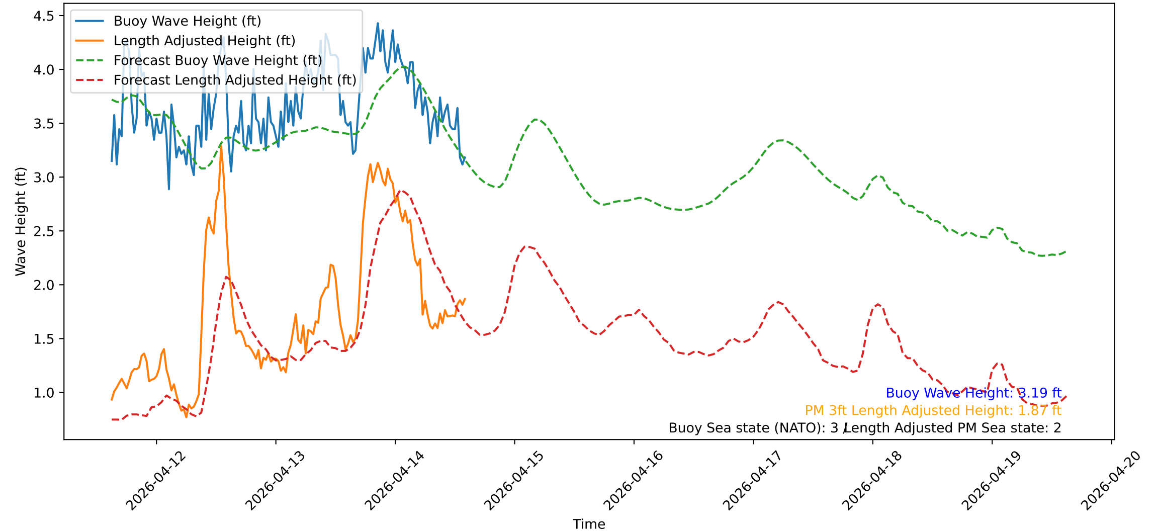
Wave Heights over Time for Red Beach at 2026-04-14 14:40:50
