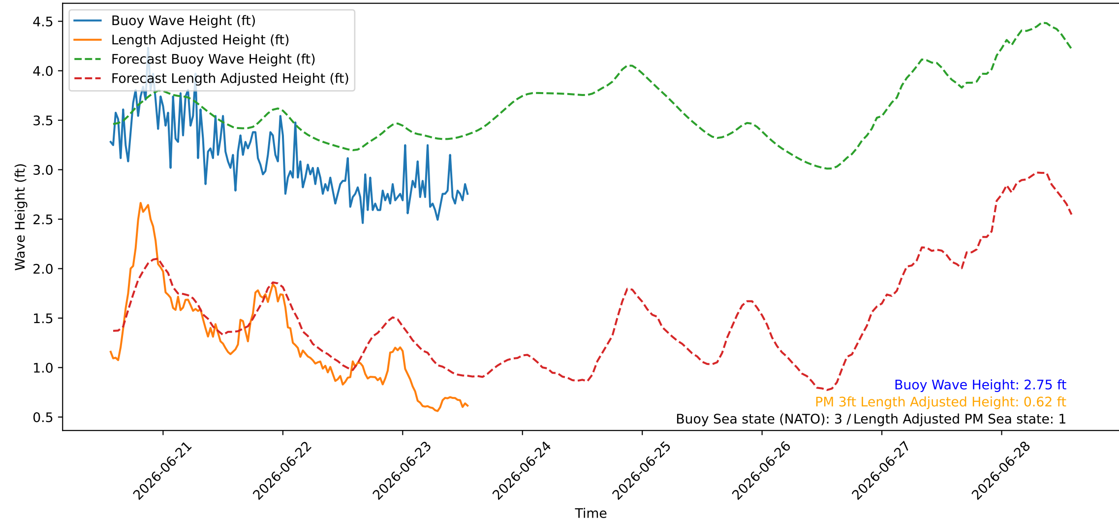
Wave Heights over Time for Green Beach at 2026-06-23 13:41:09
