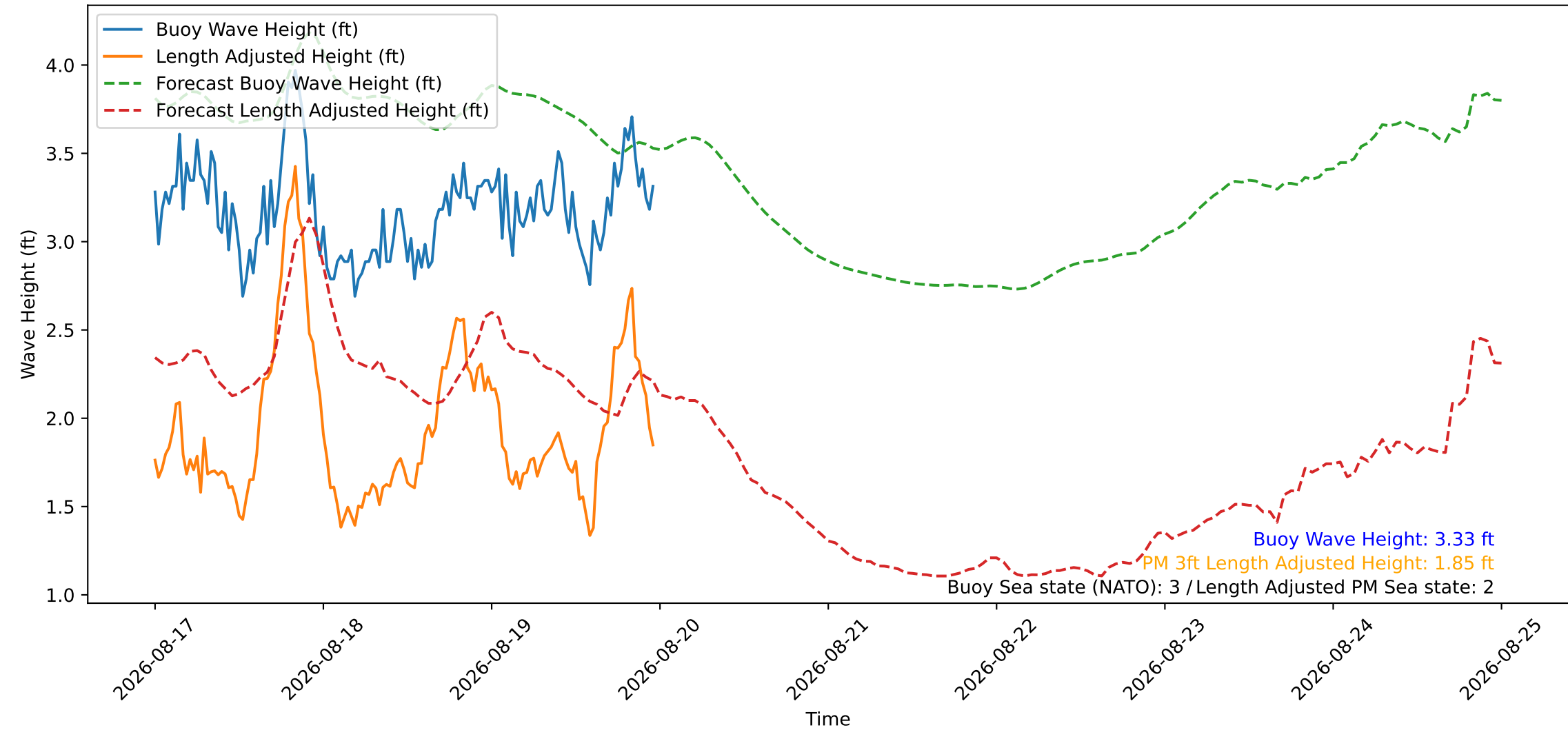
Wave Heights over Time for Green Beach at 2026-08-19 23:51:11
