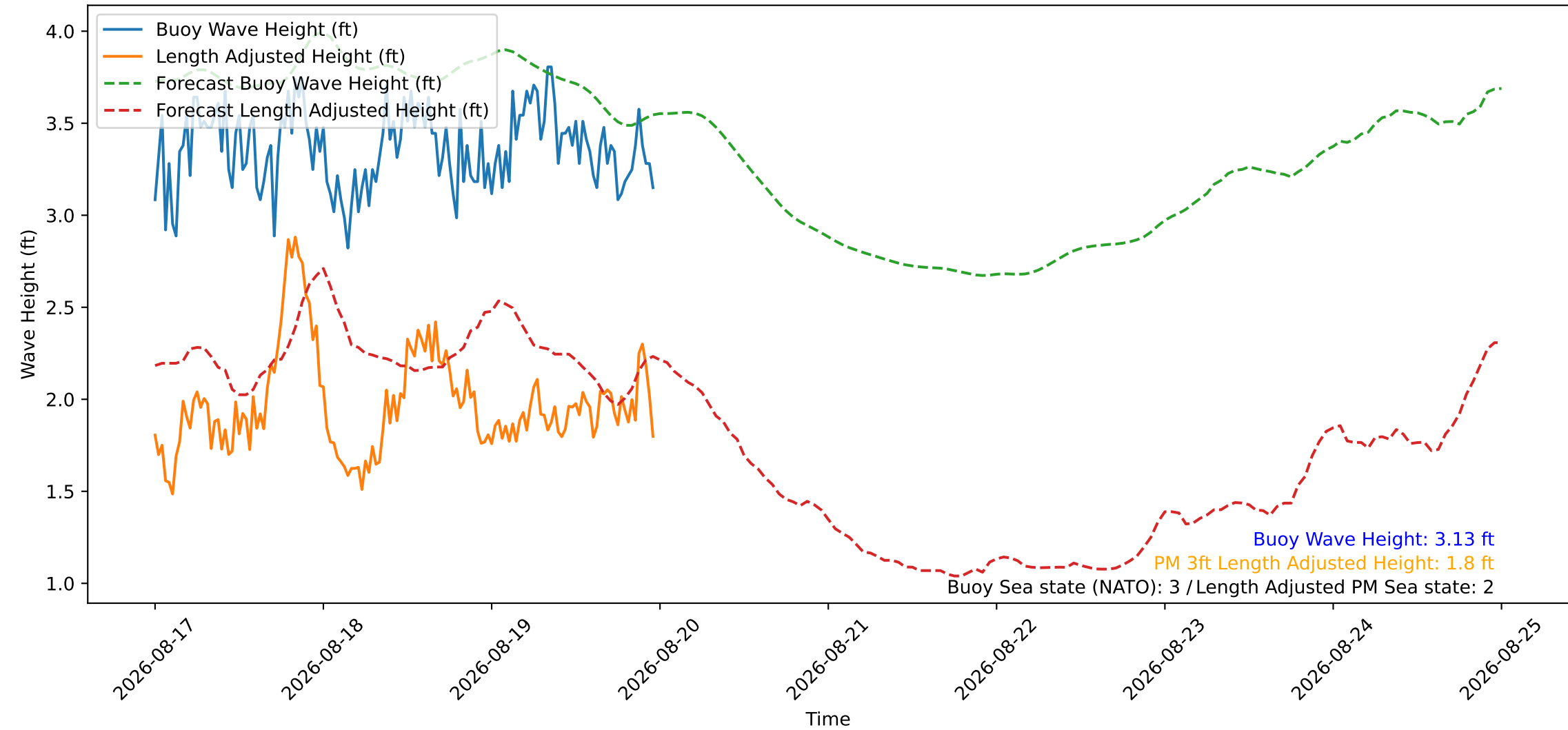
Wave Heights over Time for Oceanside Harbor at 2026-08-19 23:50:26
