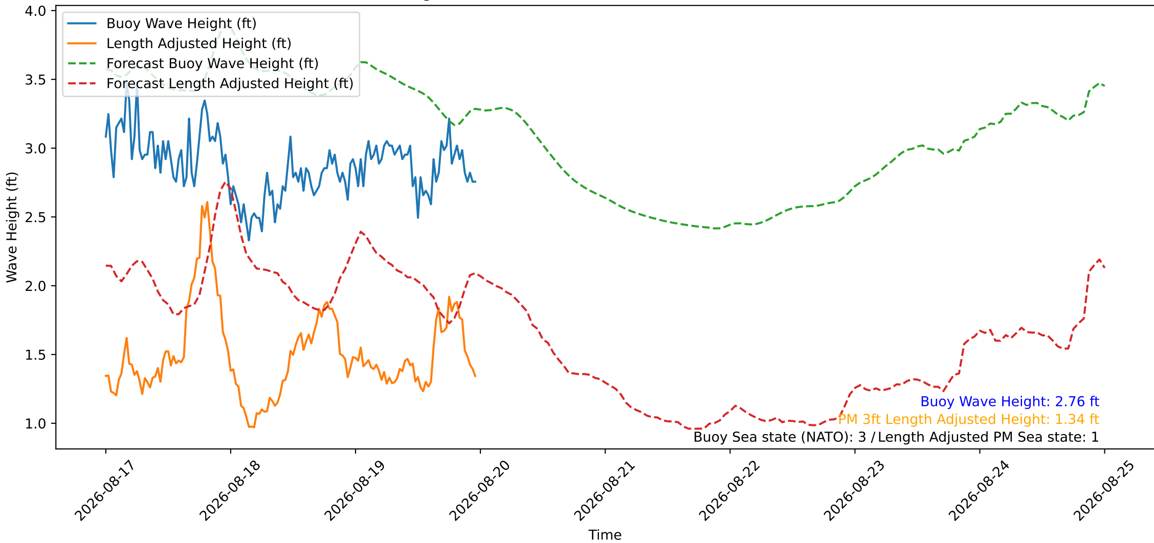
Wave Heights over Time for Red Beach at 2026-08-19 23:50:47
