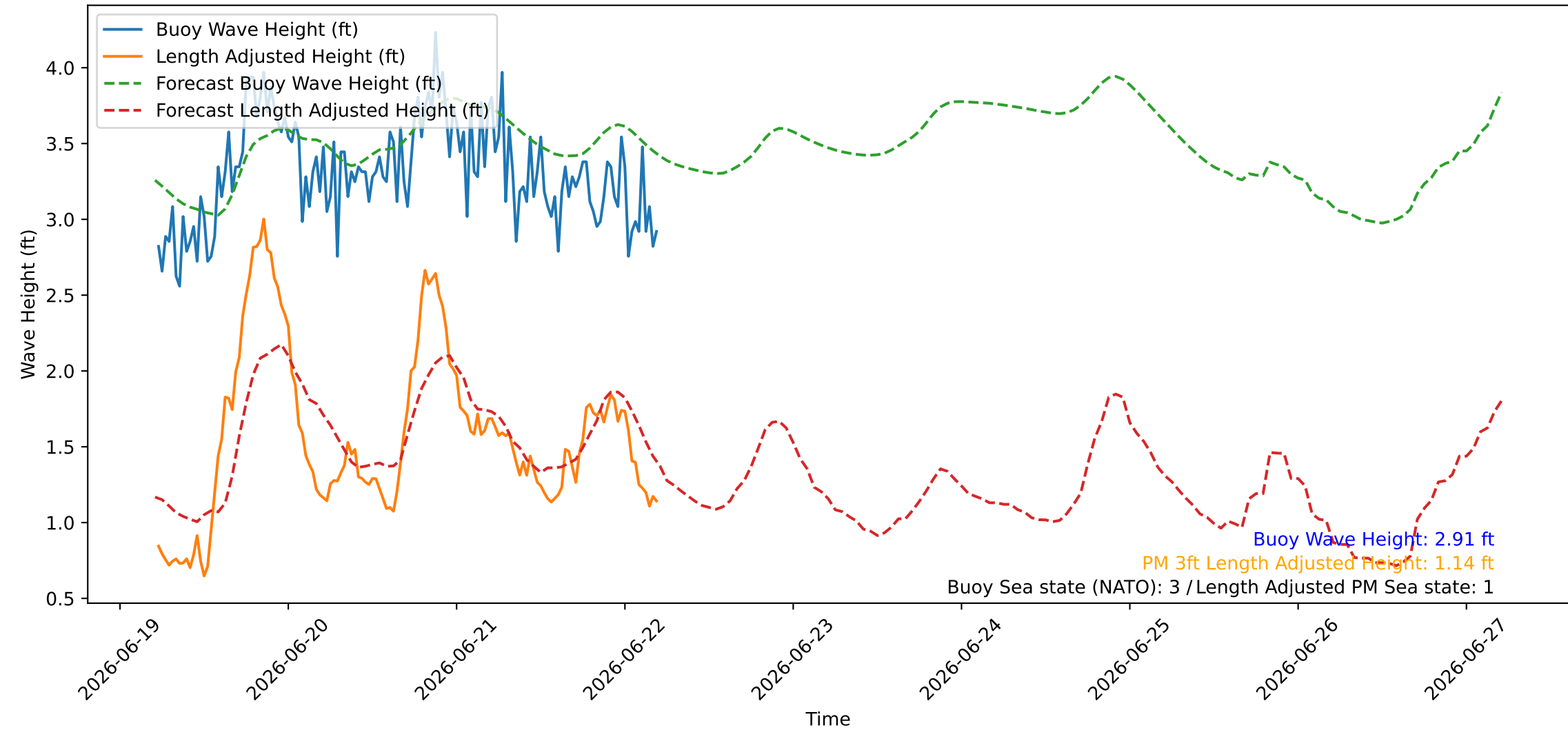
Wave Heights over Time for Green Beach at 2026-06-22 05:21:08
