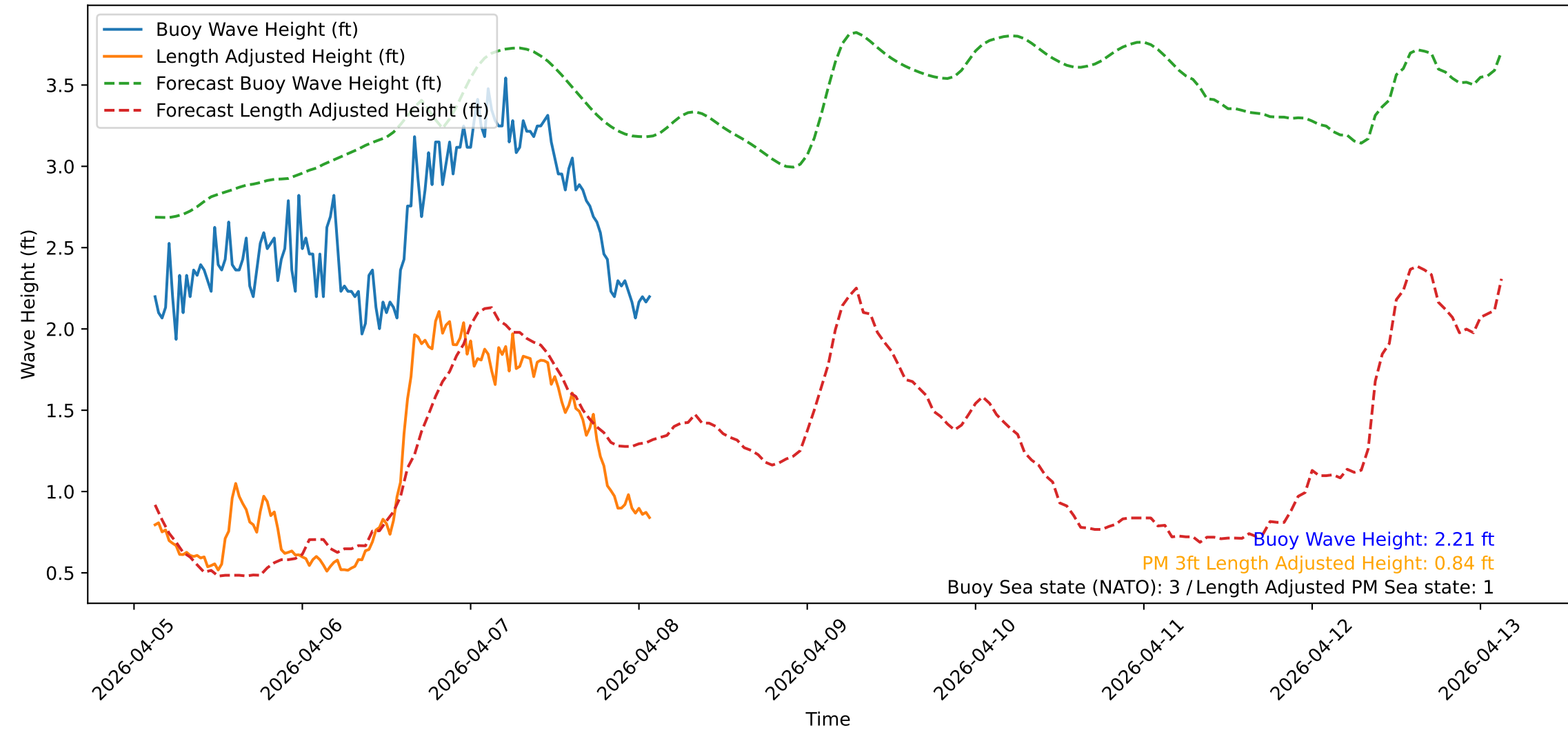
Wave Heights over Time for Red Beach at 2026-04-08 02:30:48
