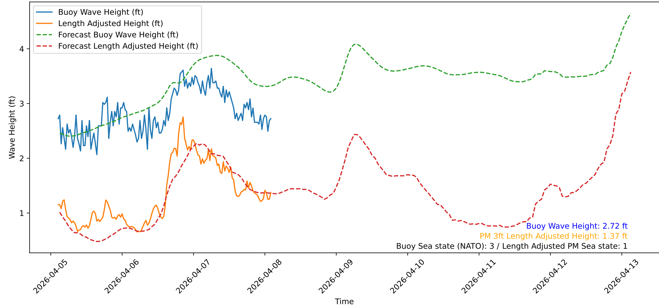
Wave Heights over Time for Oceanside Harbor at 2026-04-08 02:30:32
