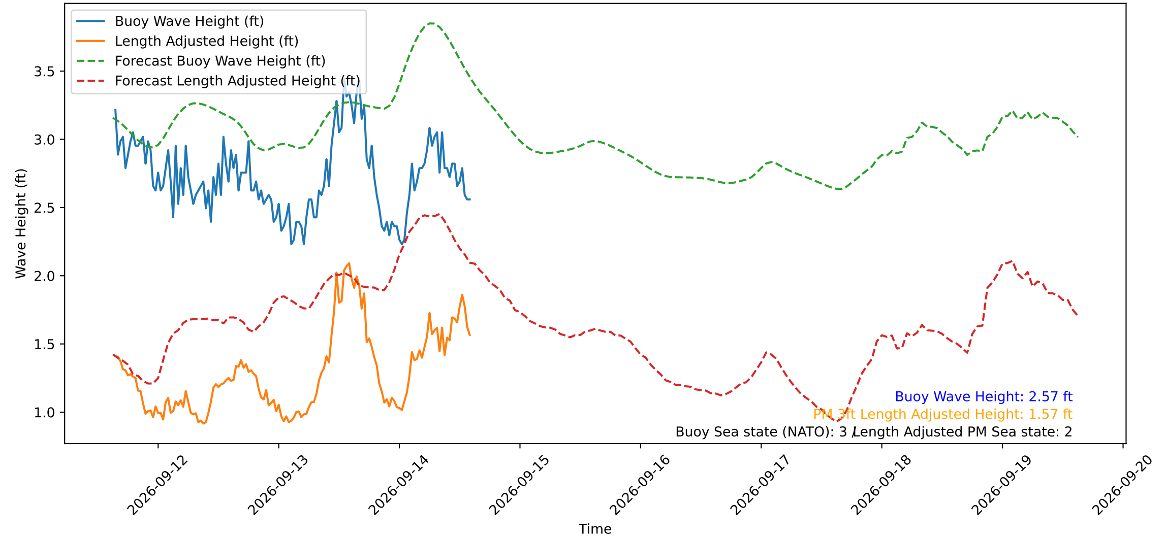
Wave Heights over Time for Red Beach at 2026-09-14 15:00:49
