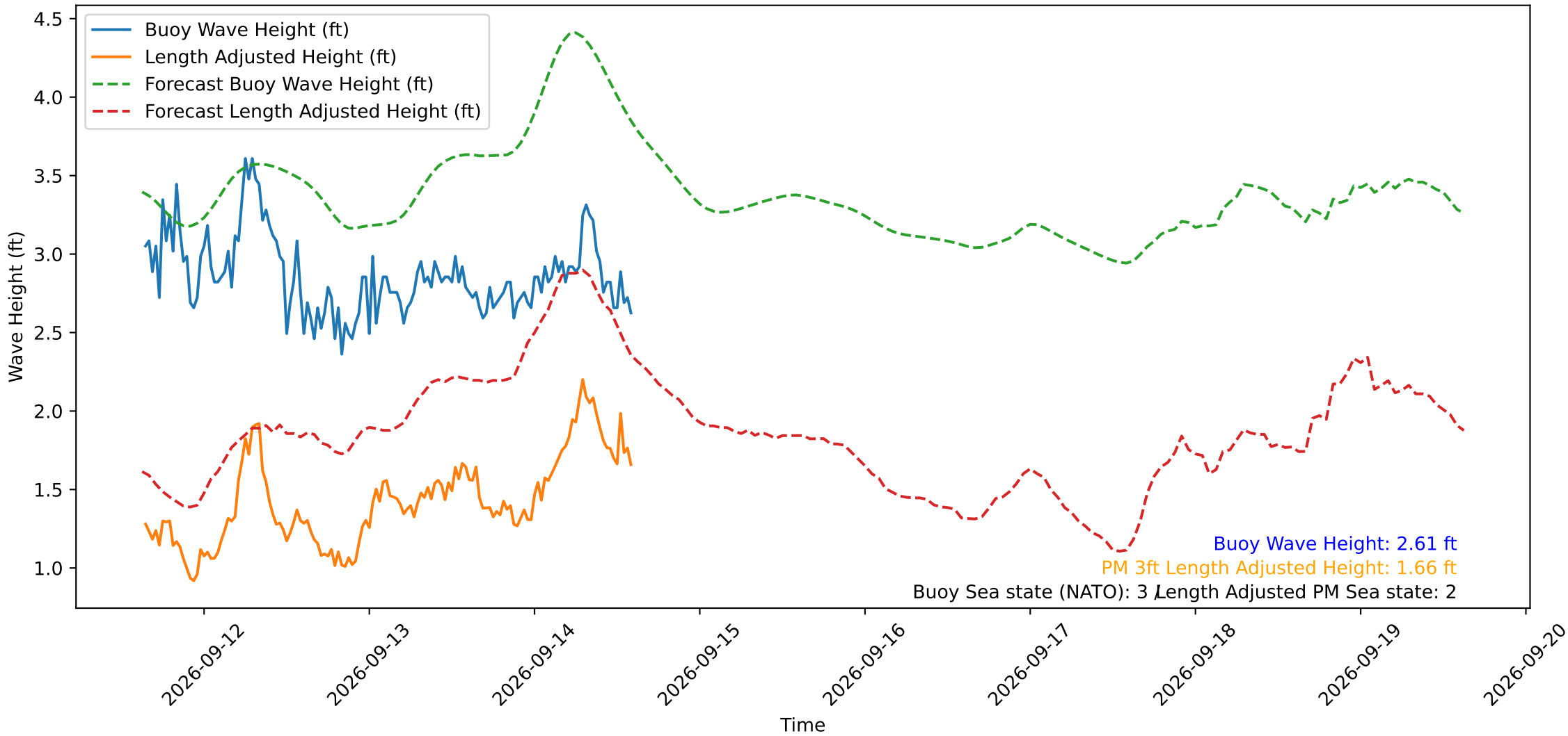
Wave Heights over Time for Green Beach at 2026-09-14 15:01:11
