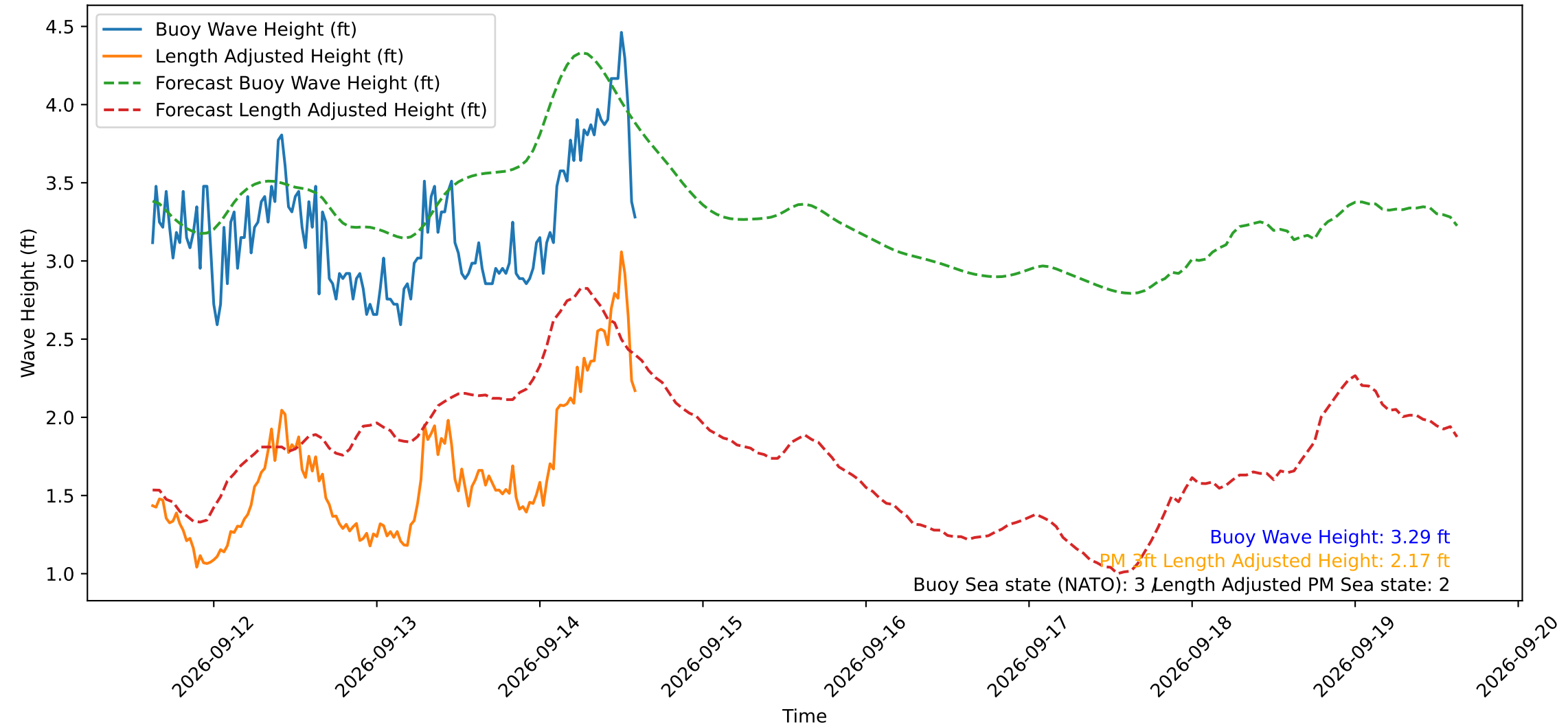
Wave Heights over Time for Oceanside Harbor at 2026-09-14 15:00:30
