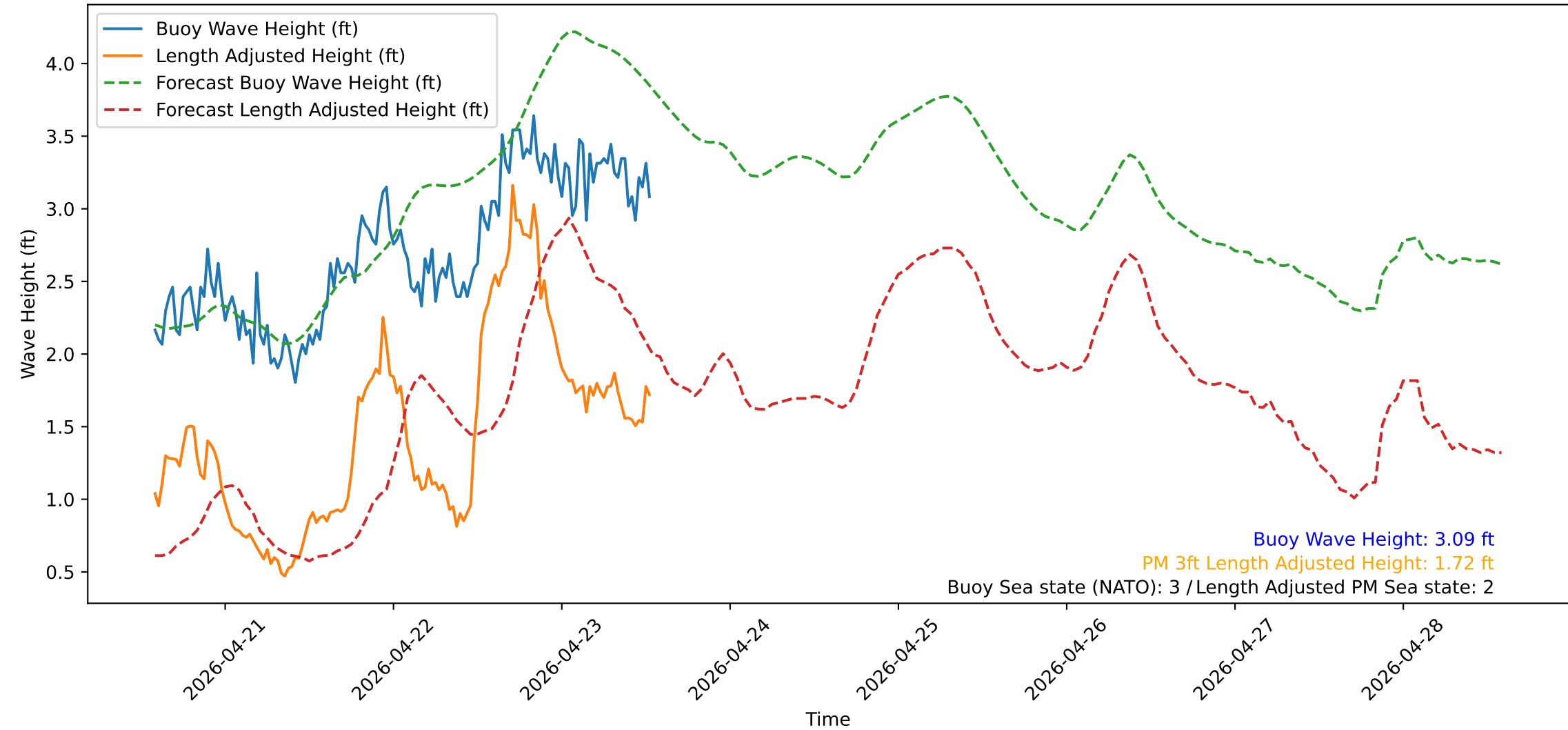
Wave Heights over Time for Red Beach at 2026-04-23 13:30:50
