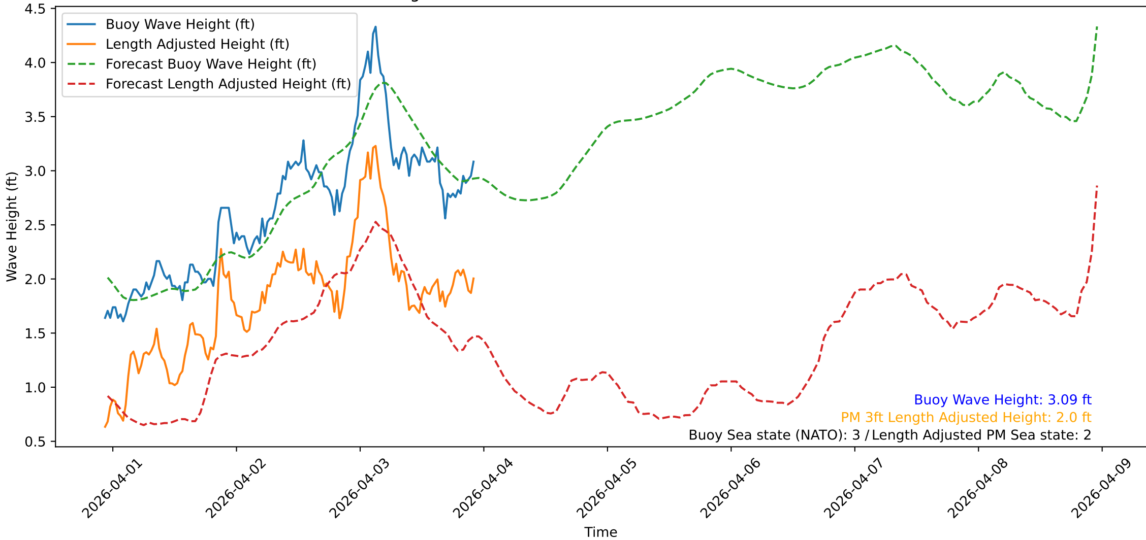
Wave Heights over Time for Green Beach at 2026-04-03 22:41:28
