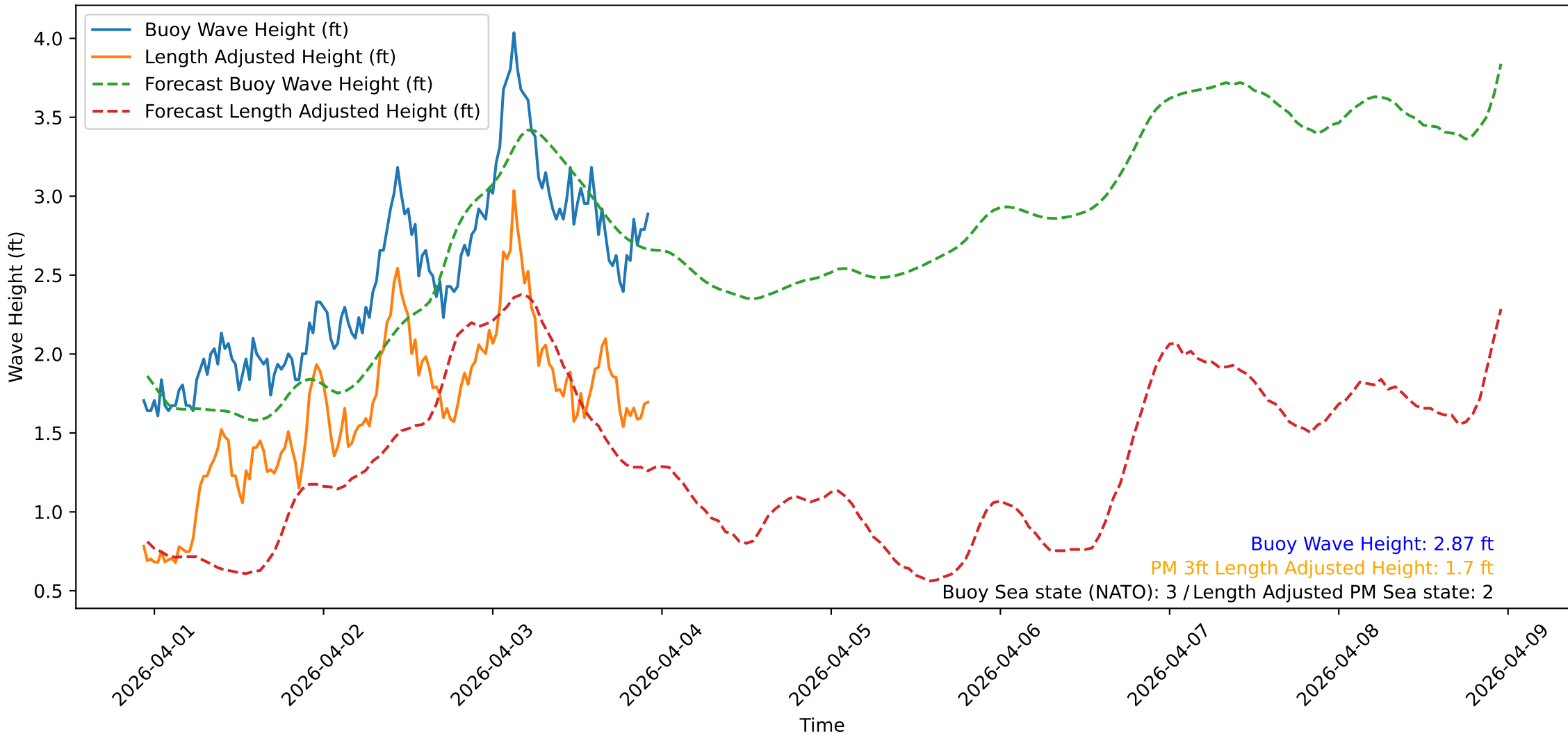
Wave Heights over Time for Oceanside Harbor at 2026-04-03 22:40:37
