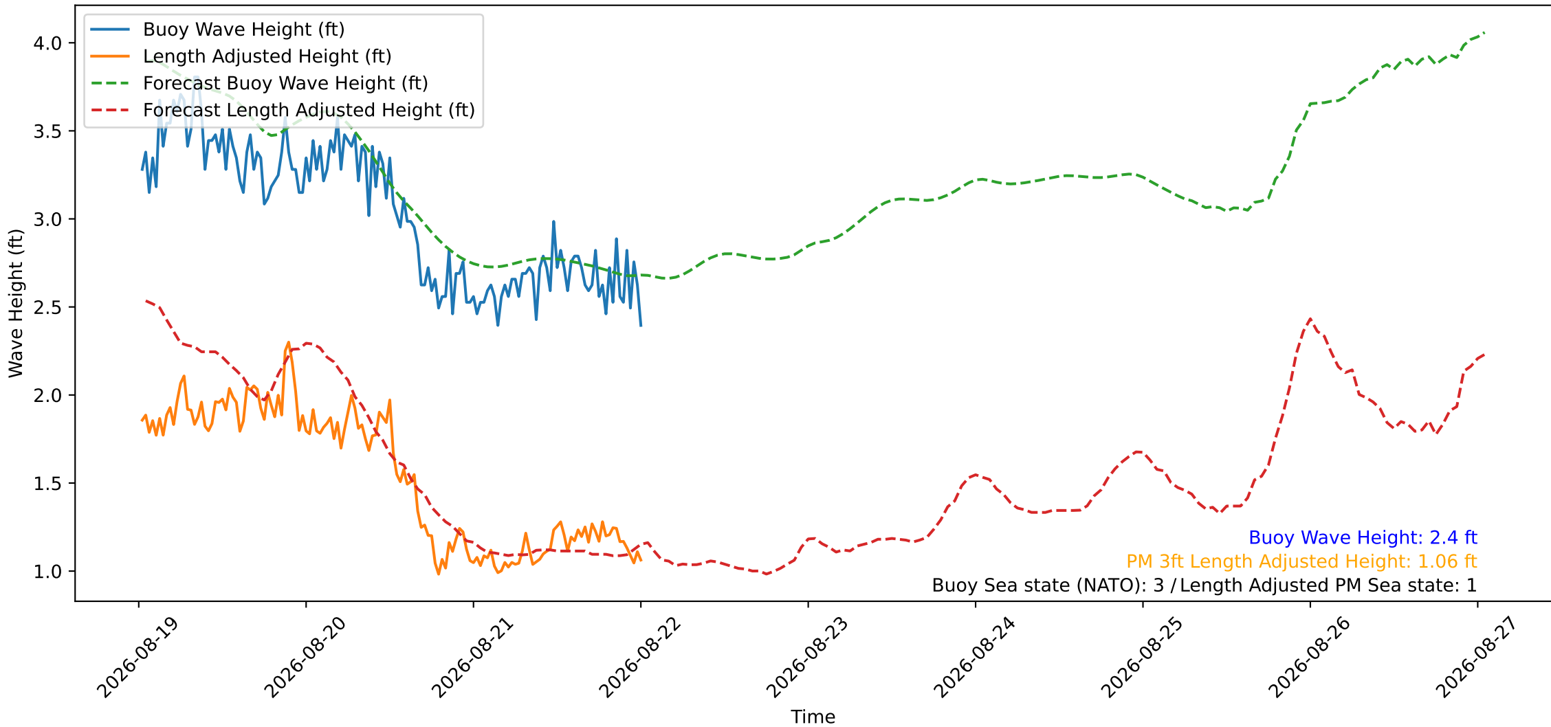
Wave Heights over Time for Oceanside Harbor at 2026-08-22 00:40:29
