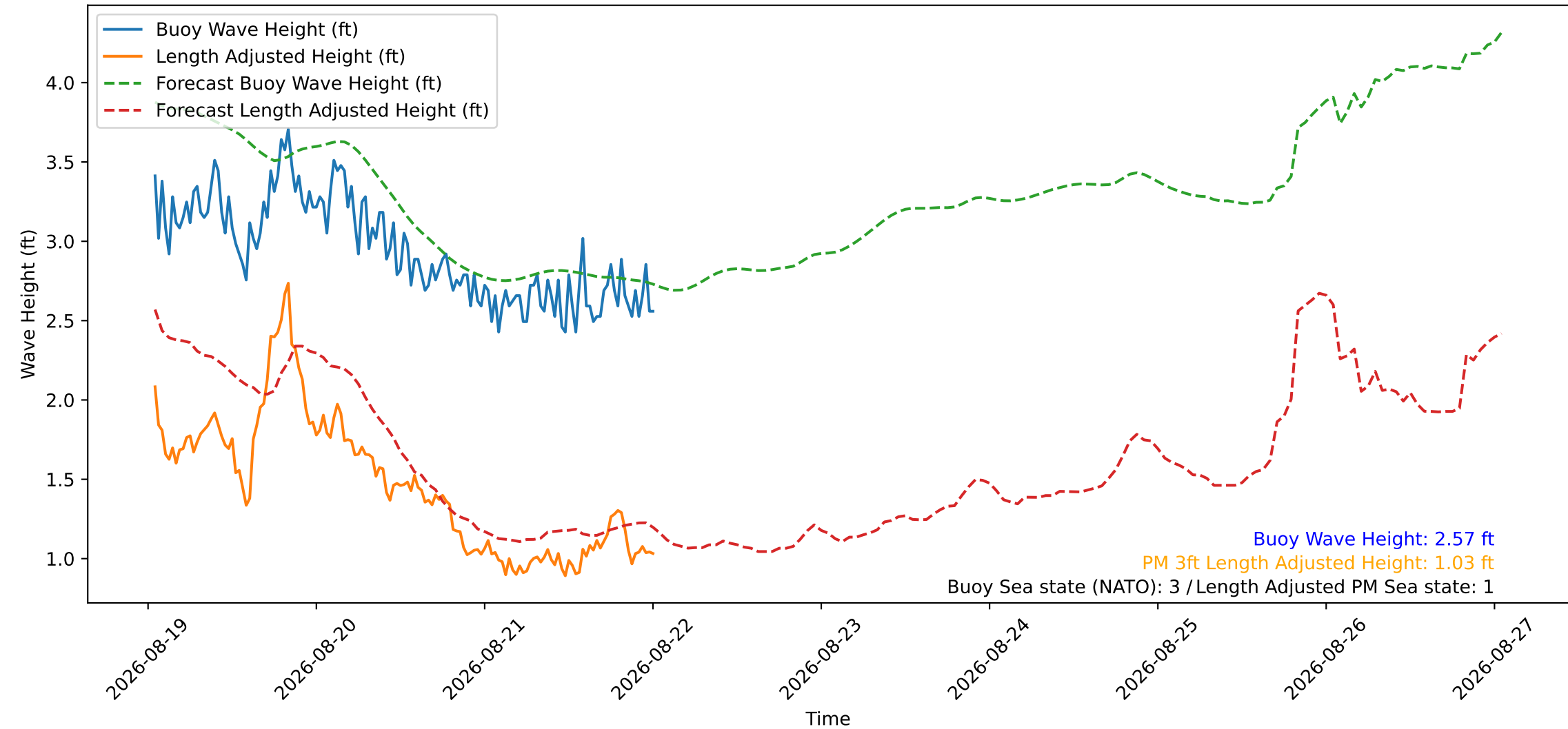
Wave Heights over Time for Green Beach at 2026-08-22 00:41:12
