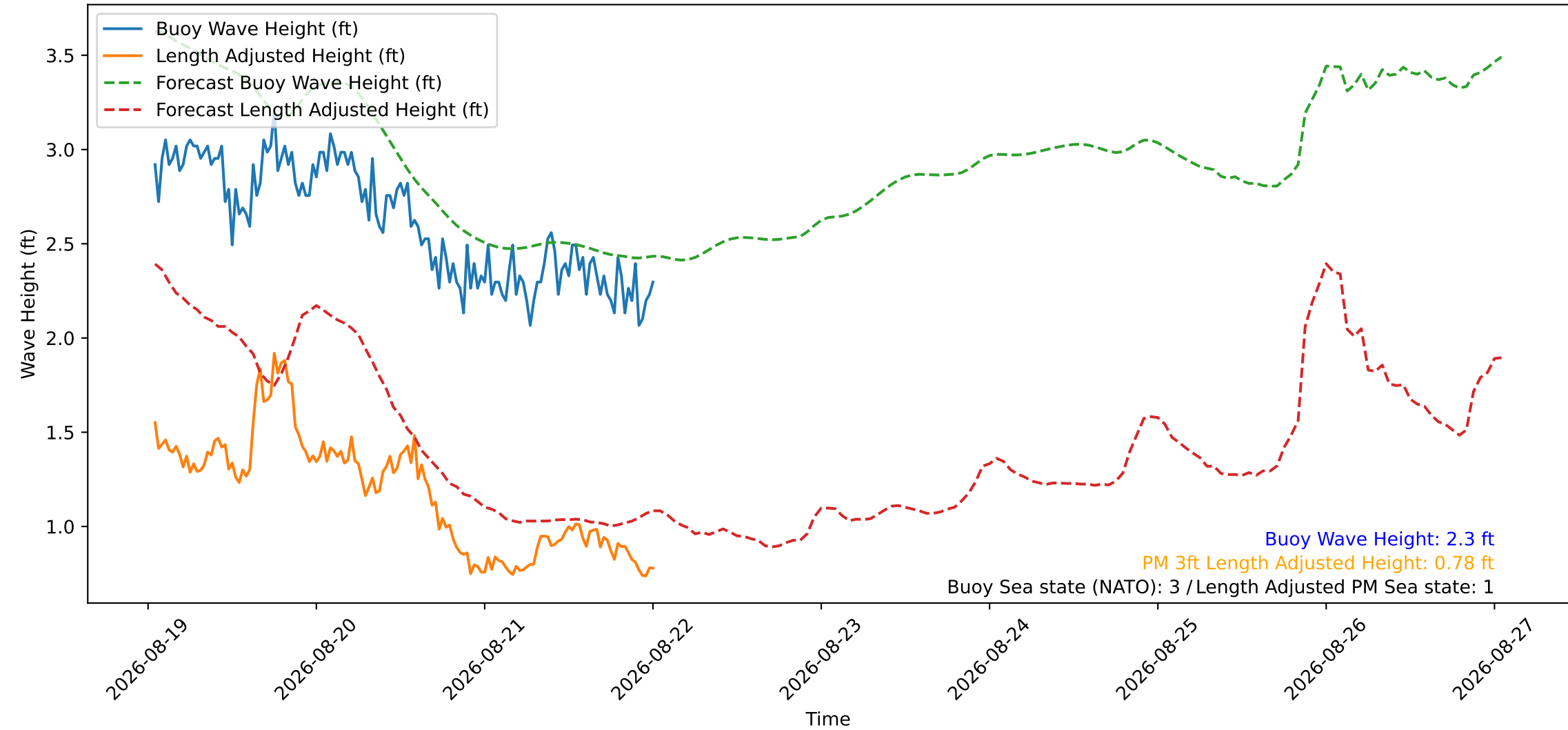
Wave Heights over Time for Red Beach at 2026-08-22 00:40:50
