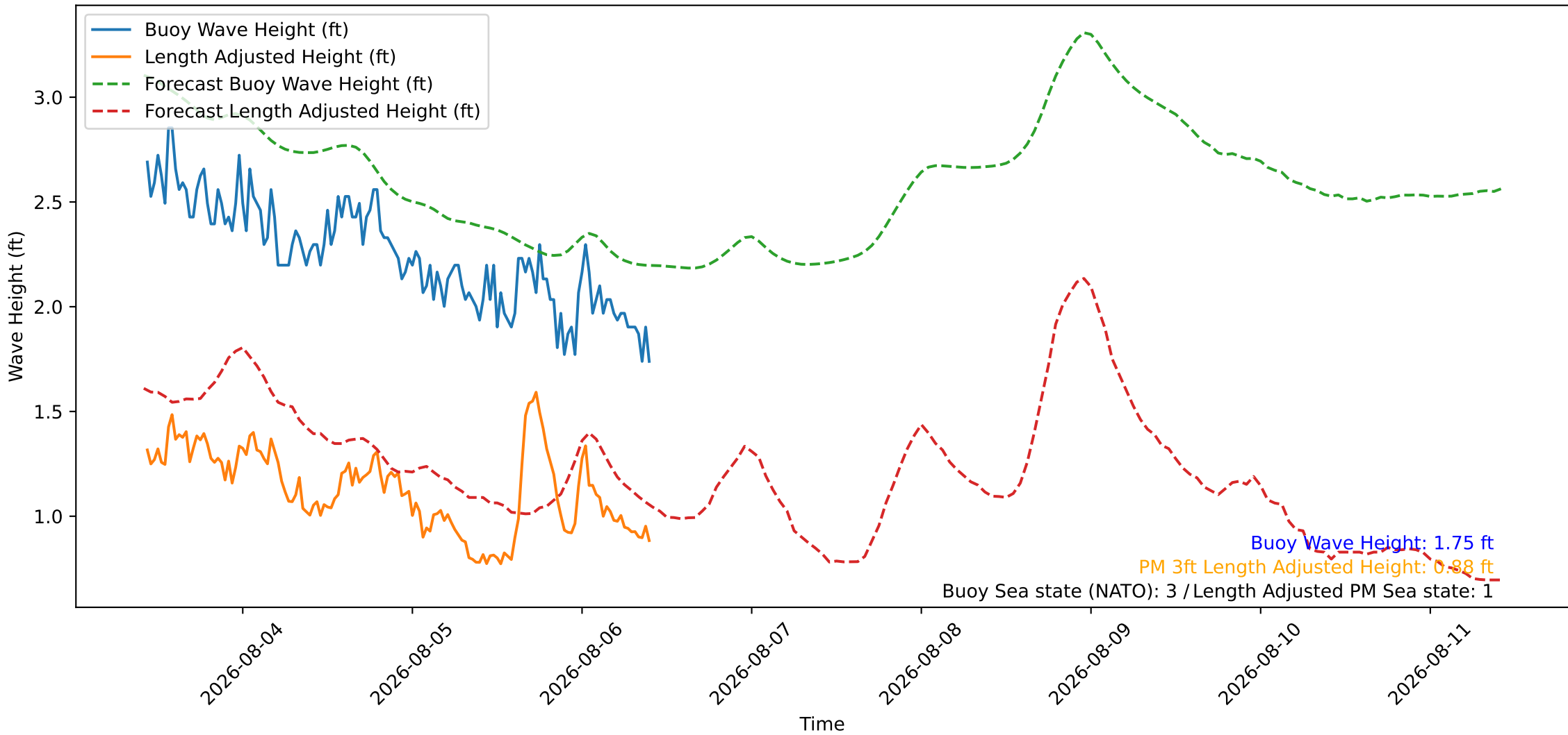
Wave Heights over Time for Oceanside Harbor at 2026-08-06 10:20:27
