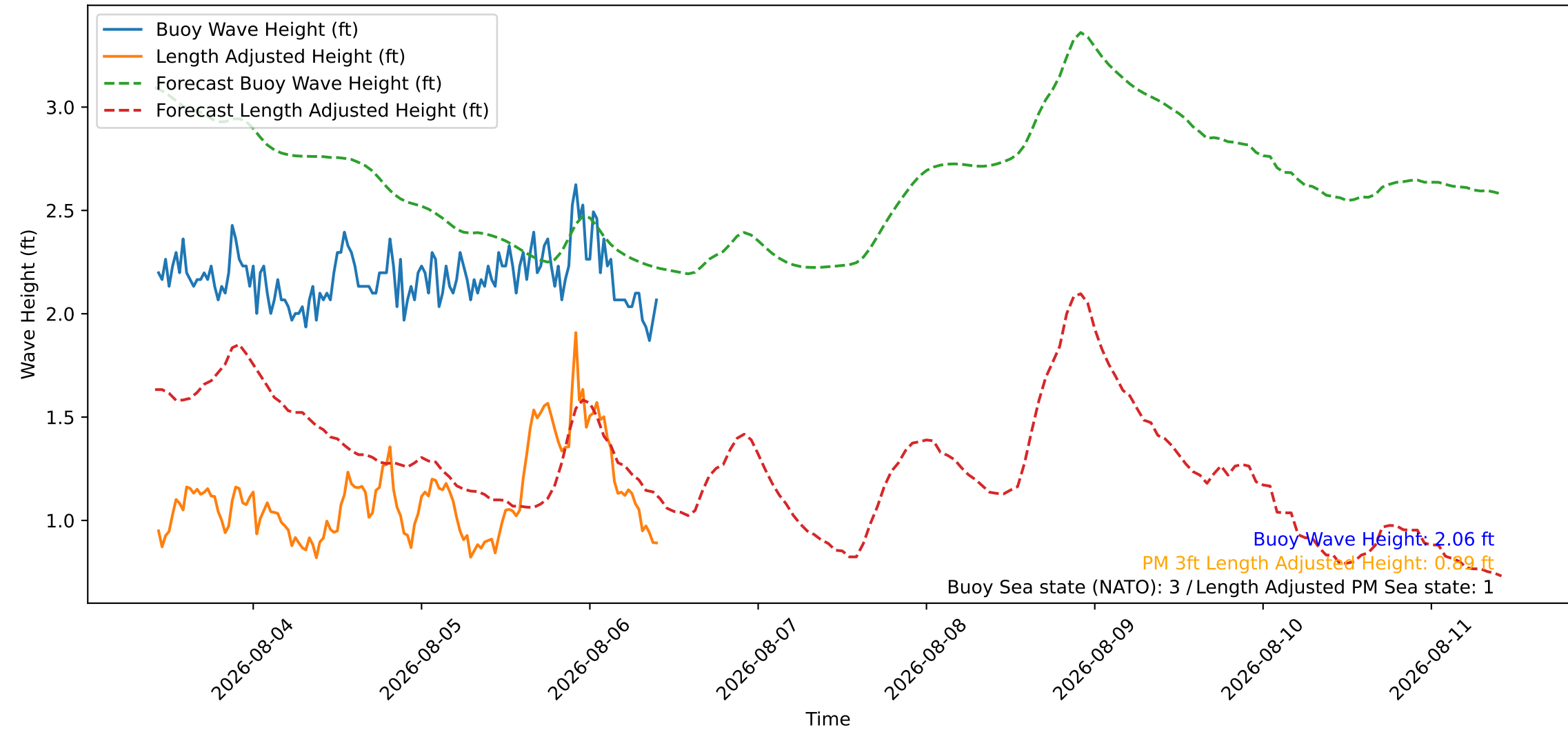
Wave Heights over Time for Green Beach at 2026-08-06 10:21:09
